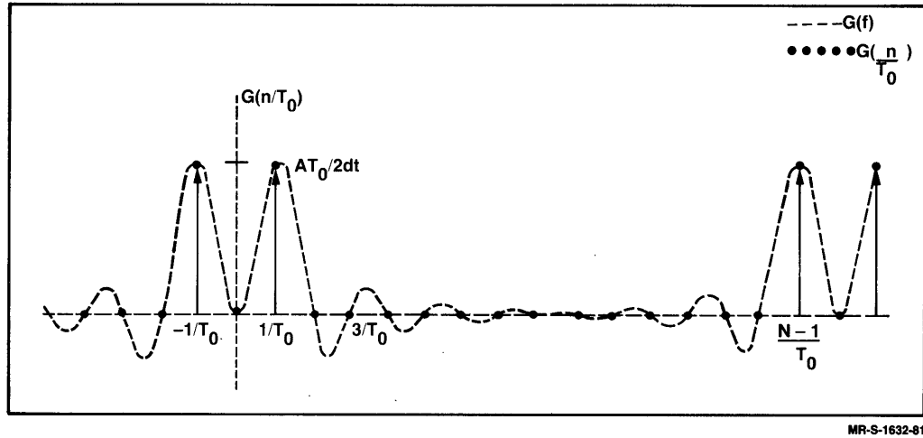
Figure 6-4: G(n \cdot df) Returned by the FFT
