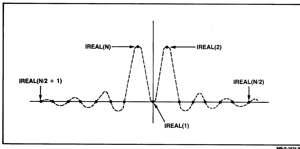
Figure 6-6: Five Elements in the IREAL Output Array
