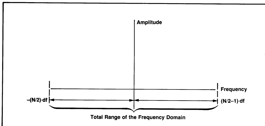
Figure 6-5: Total Range of the Frequency Domain
