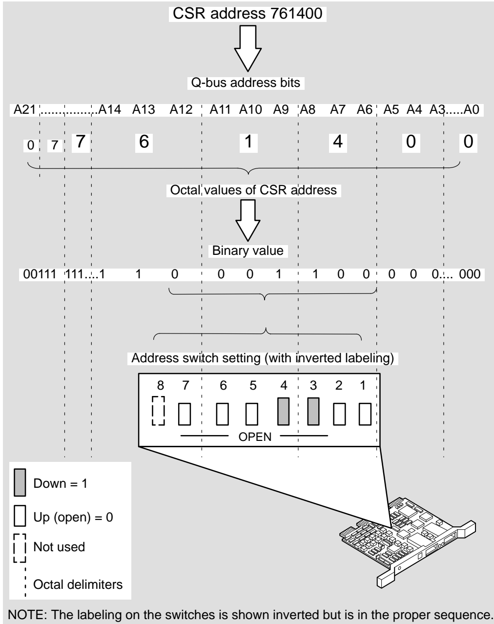
Figure 3–1: An Example of CSR Address Switch Settings (Top View)
