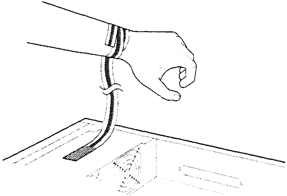
Figure 18 Attaching Antistatic Strap
