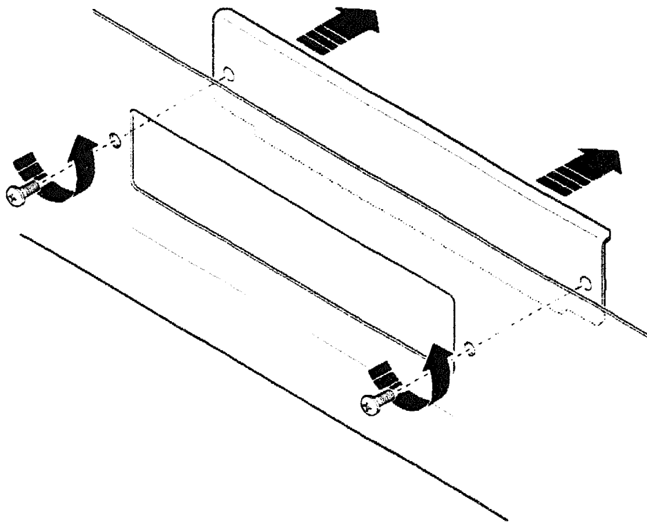
Figure 19 Removing the Options Slot Cover
