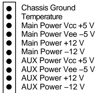
Figure 2–6 Power Tray Service Indicators
