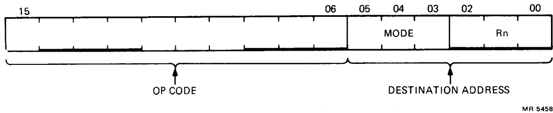
Figure 6-1 Single-Operand Addressing
