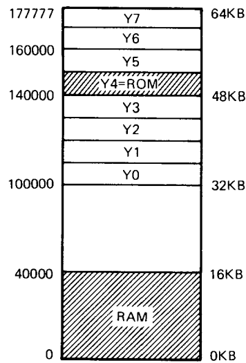
Figure 5-13 8-Bit System Memory Map
