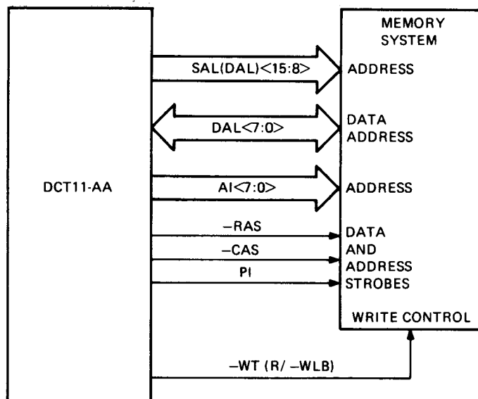
Figure 2-16 8-Bit Dynamic Write, Block Diagram
