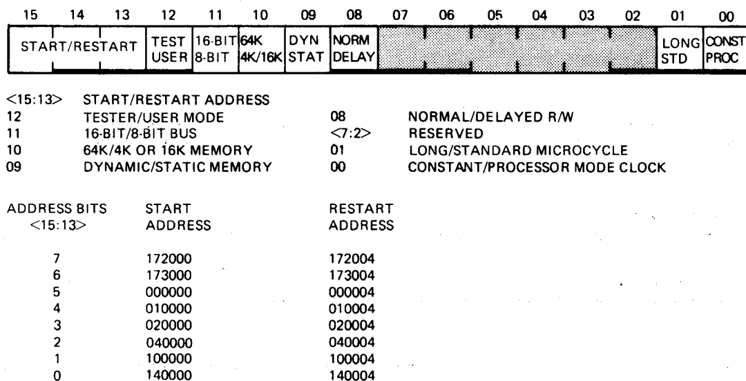
Figure 1-4 Mode Register
