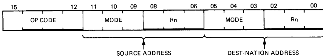
Figure 6-2 Double-Operand Addressing
