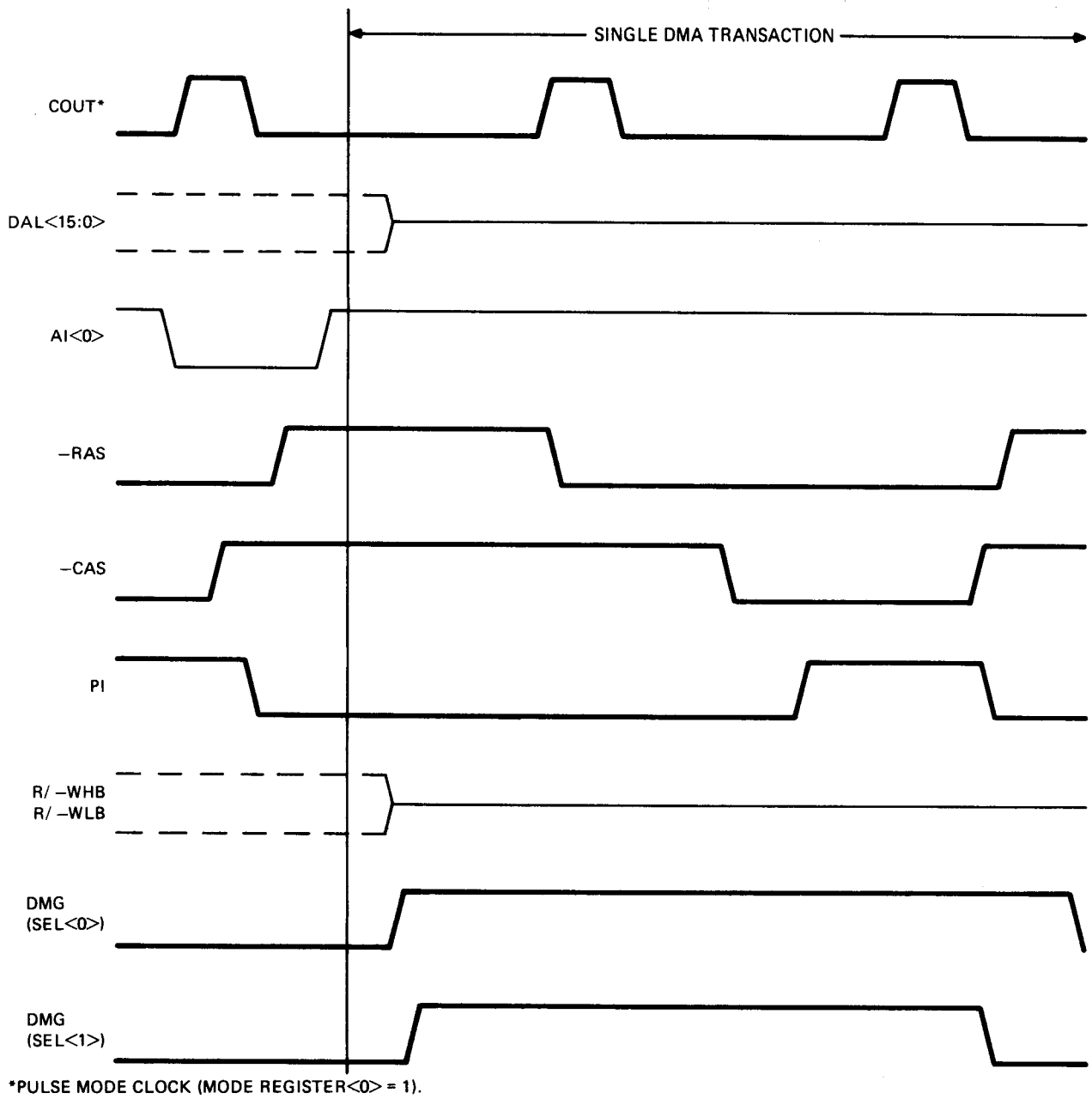
Figure 2-22 DMA Timing
