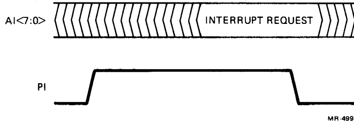
Figure 1-6 Interrupt Timing
