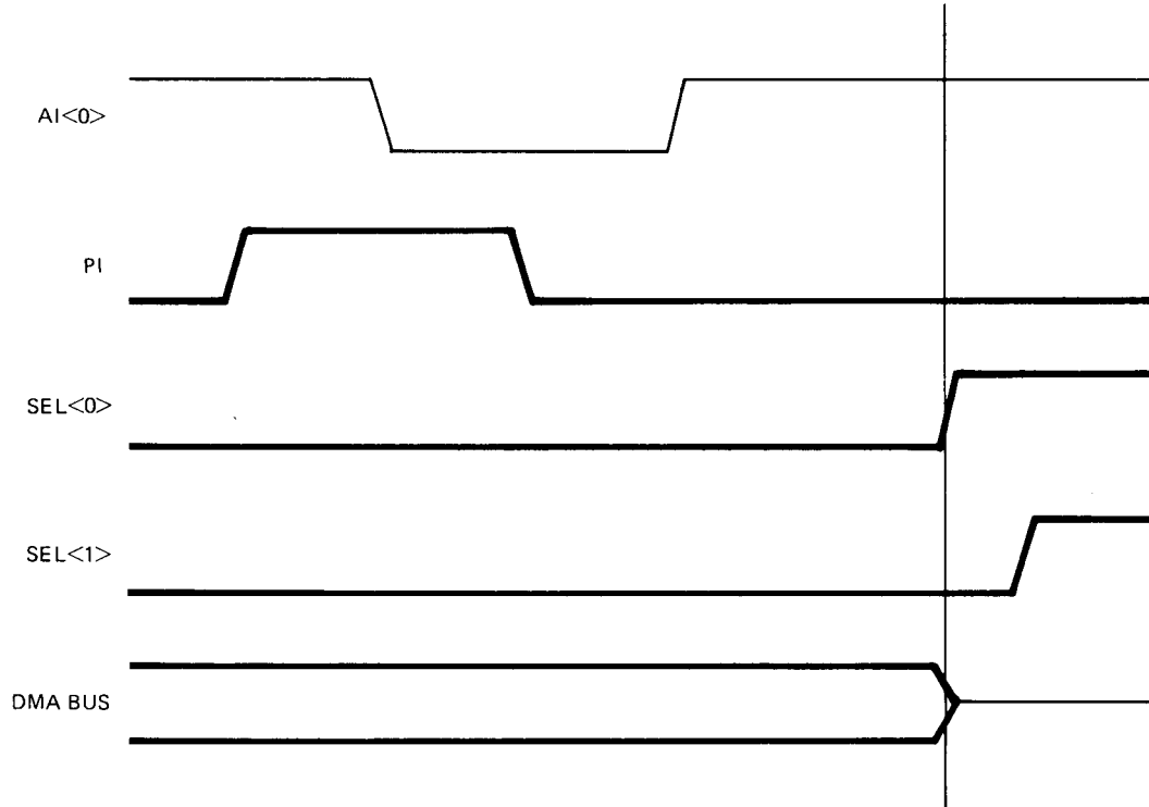
Figure 1-7 DMA Timing
