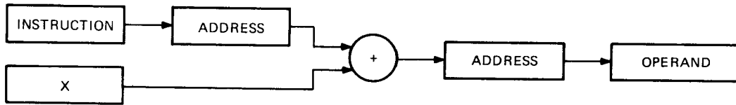
Figure 6-22 Mode 7 Index-Deferred
