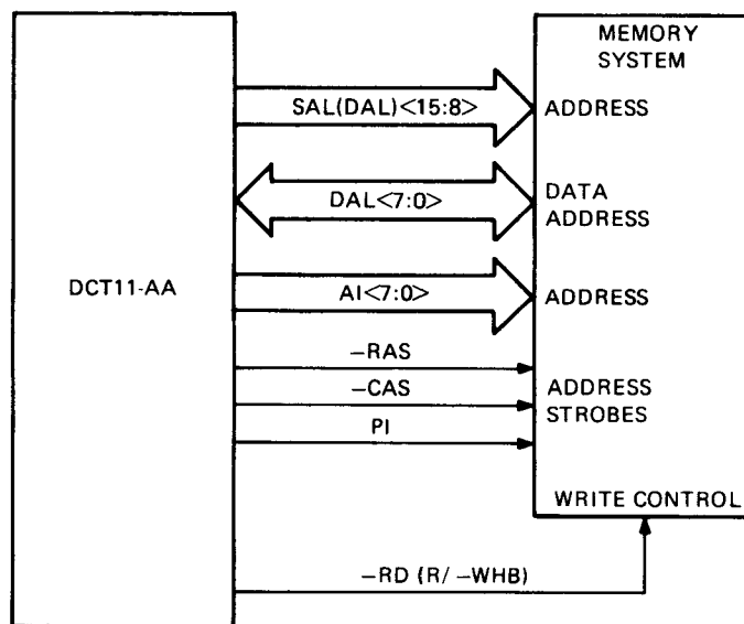
Figure 2-14 8-Bit Dynamic Read, Block Diagram
