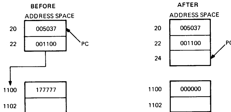
Figure 6-28 CLR @ # 1100 Clear
