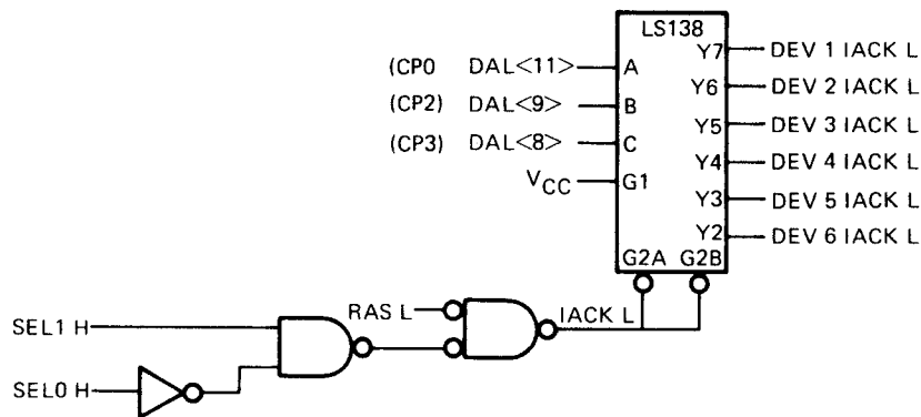
IACK CIRCUIT
