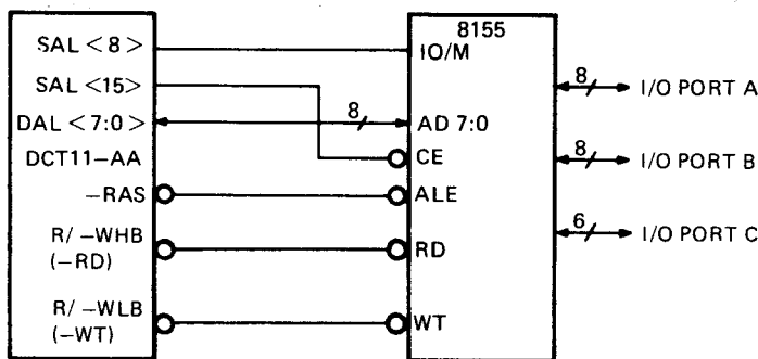
Figure 5-23 8155 RAM
