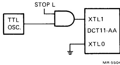
Figure 5-6 Gating XTL1
