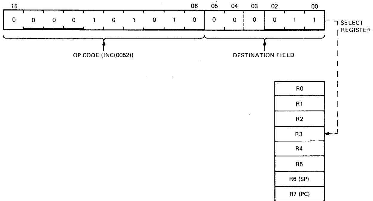
Figure 6-7 INC R3 Increment
