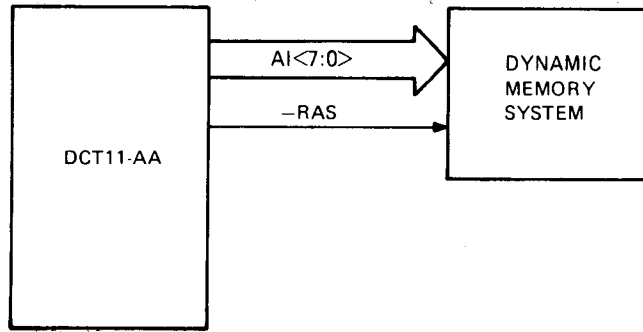
Figure 2-18 Refresh Transaction, Block Diagram
