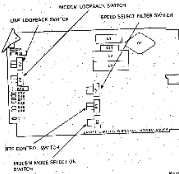
Figure 3-9 M8998 Switch Locations
