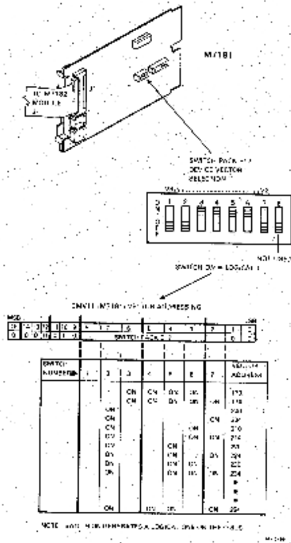
Figure 2-4 CMV11 (M7181) Vector Address Selection
