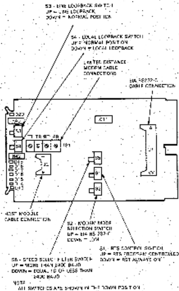
Figure 2-6 HWF LDM (M8996) Modem Variables
