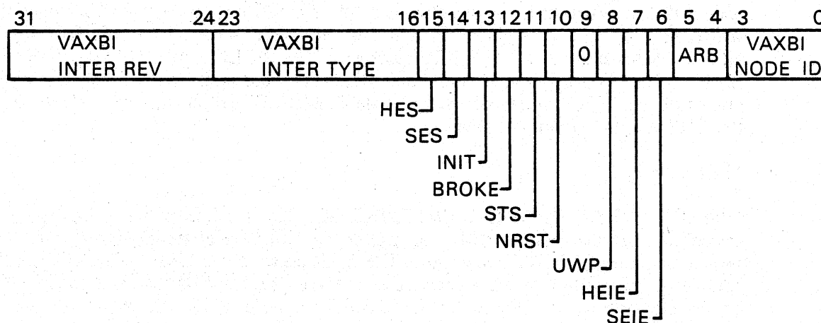
Figure A-10 VAXBI Control and Status Register
