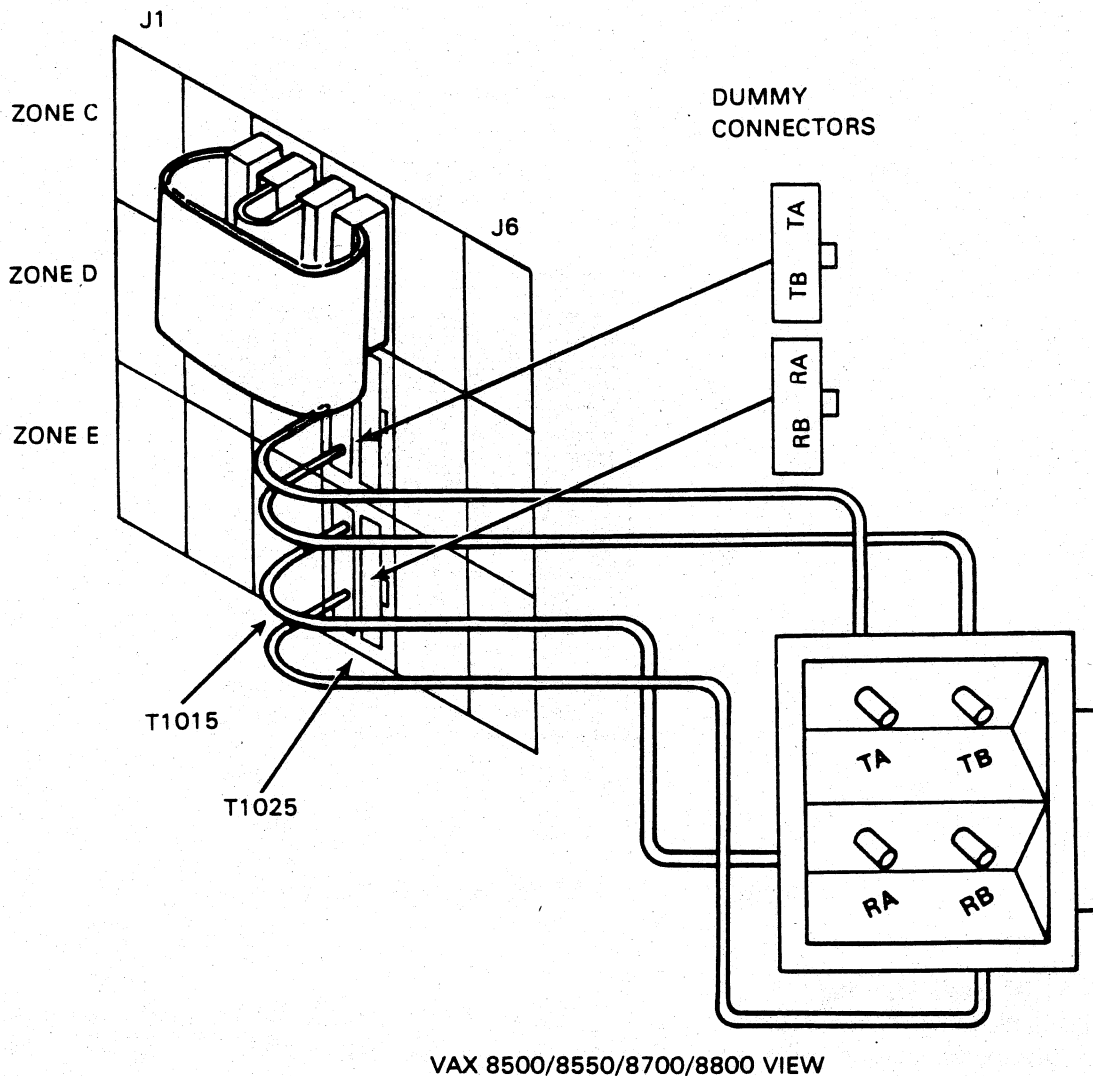
Figure 2-6 CIBCA CI Internal Bulkhead Cable Assembly Installation
