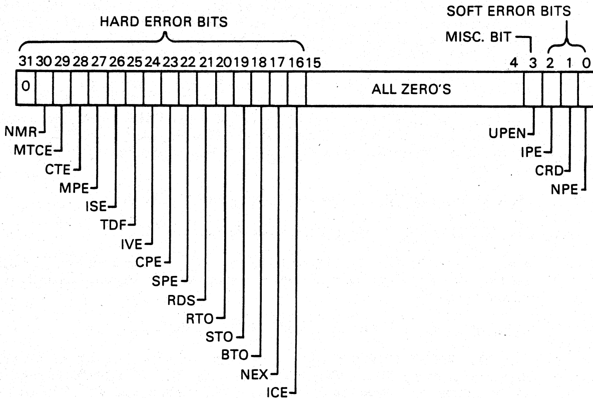
Figure A-11 Bus Error Register
