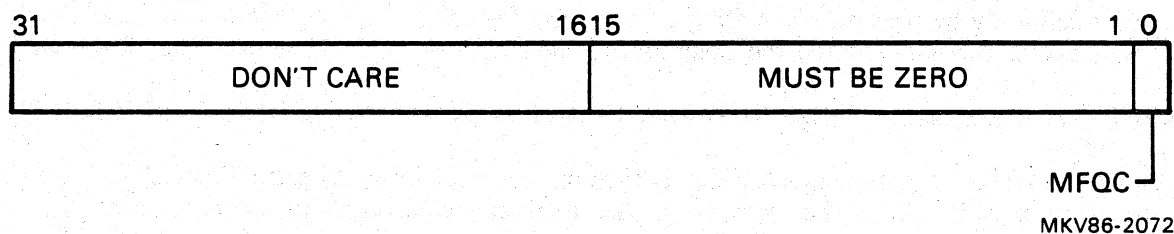
Figure A-38 Port Message Free Queue Control Register
