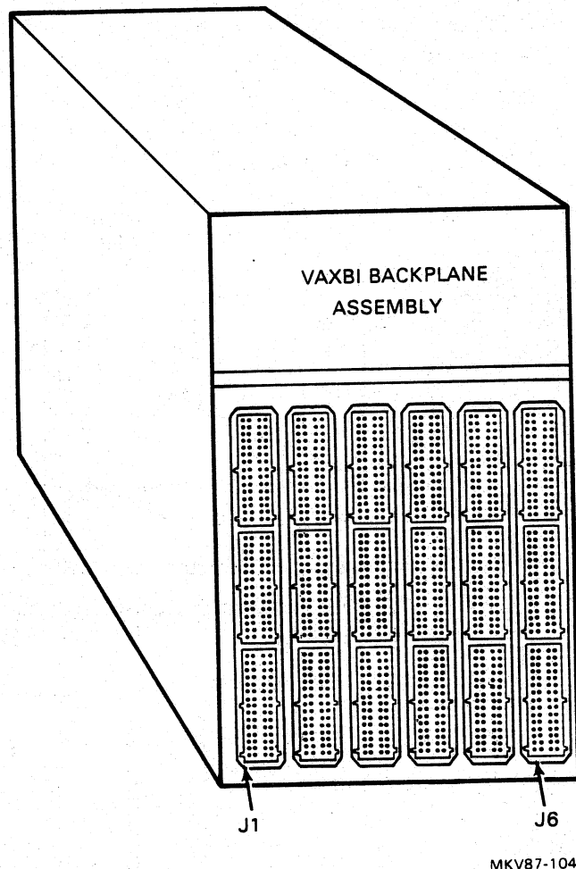
Figure 2-7 VAXBI Stationary Backplane
