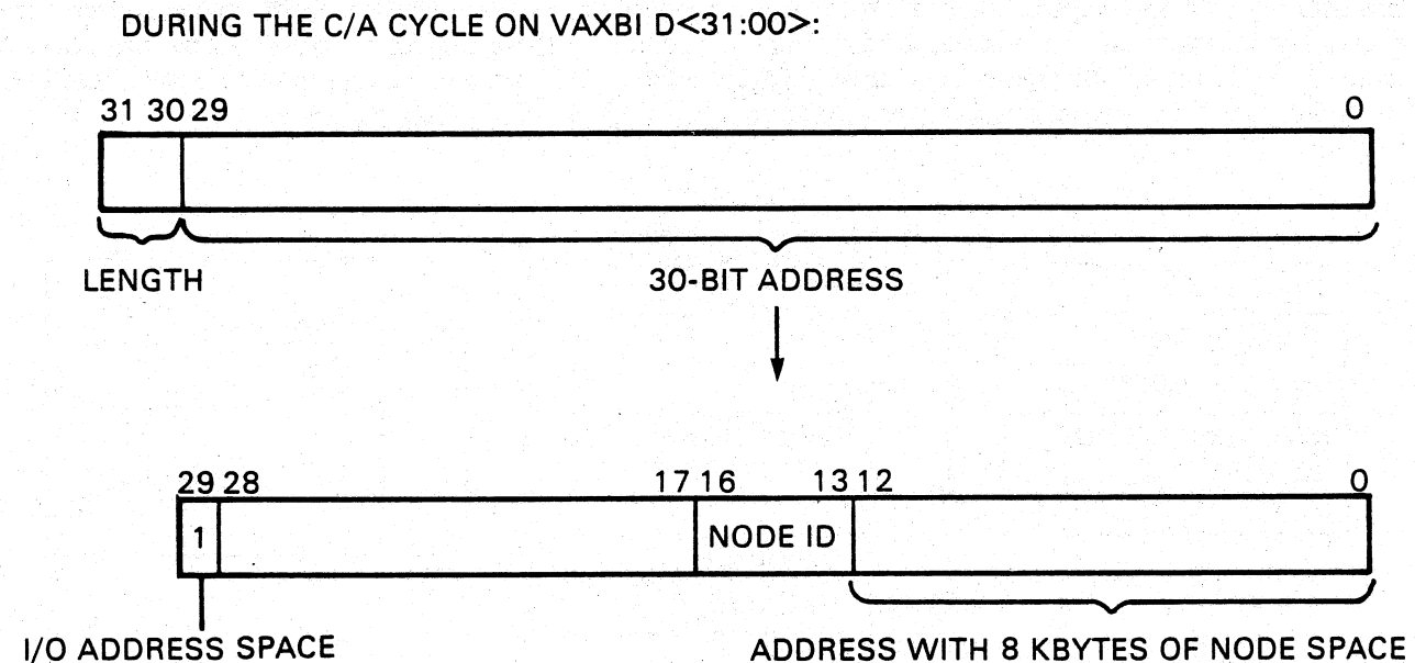
Figure A-4 30-Bit I/O Address Bit Map
