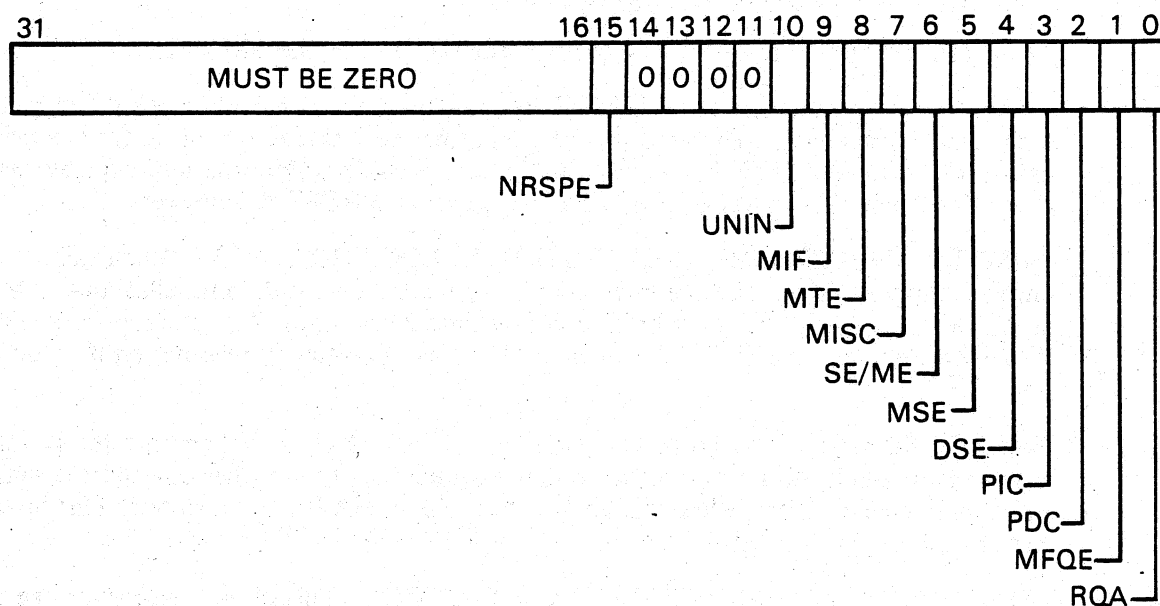
Figure A-24 Port Status Register
