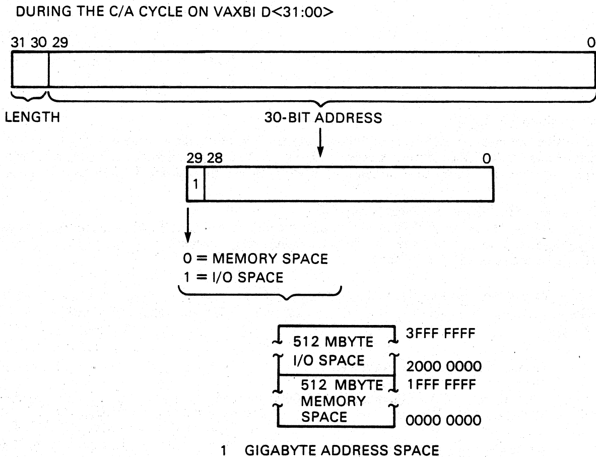
Figure A-1 VAXBI Physical Address Space
