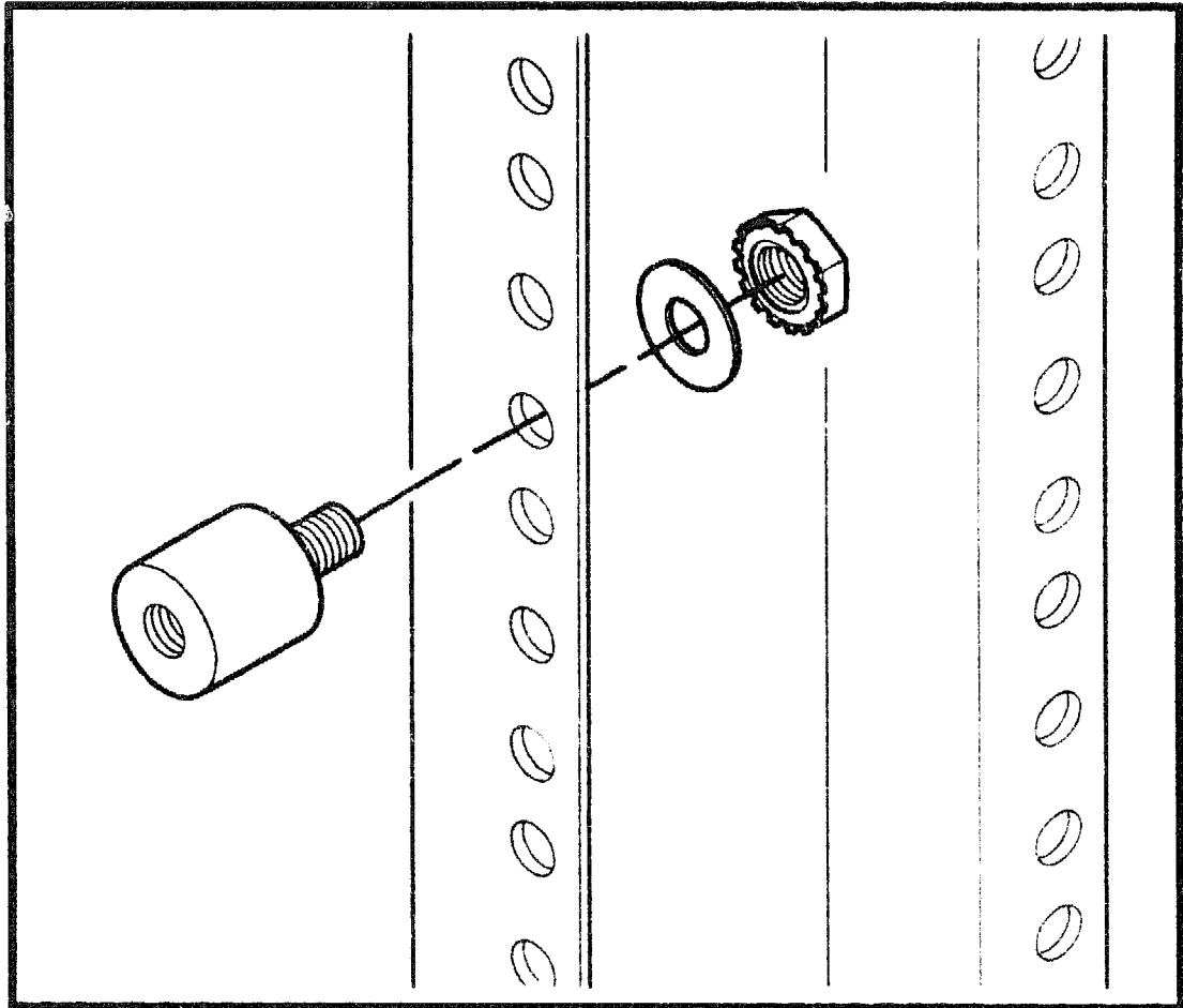
Figure 9: Mounting Isolators
