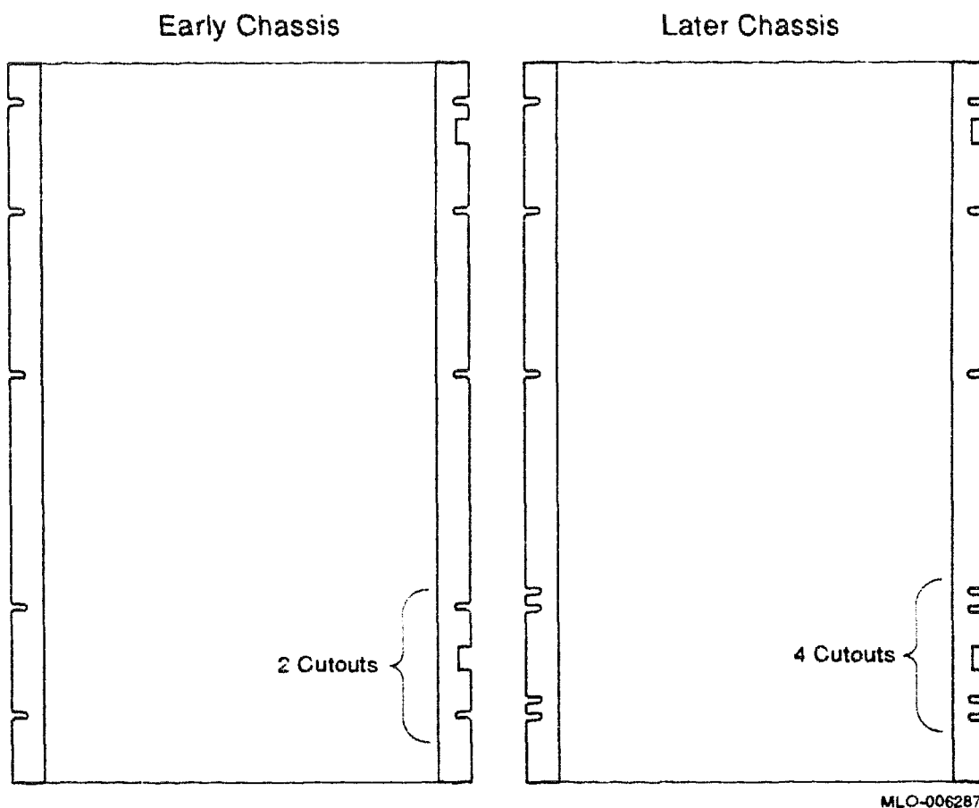
Figure 4: Flanges on BA400-Series Chassis
