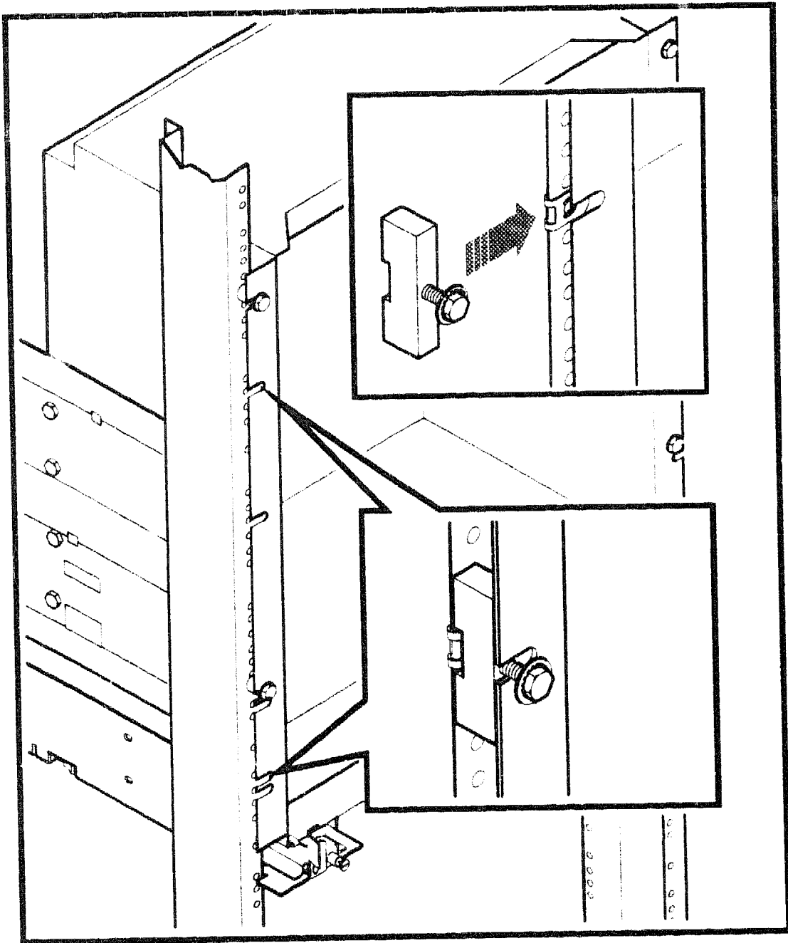
Figure A-3: Installing the Shipping Locks
