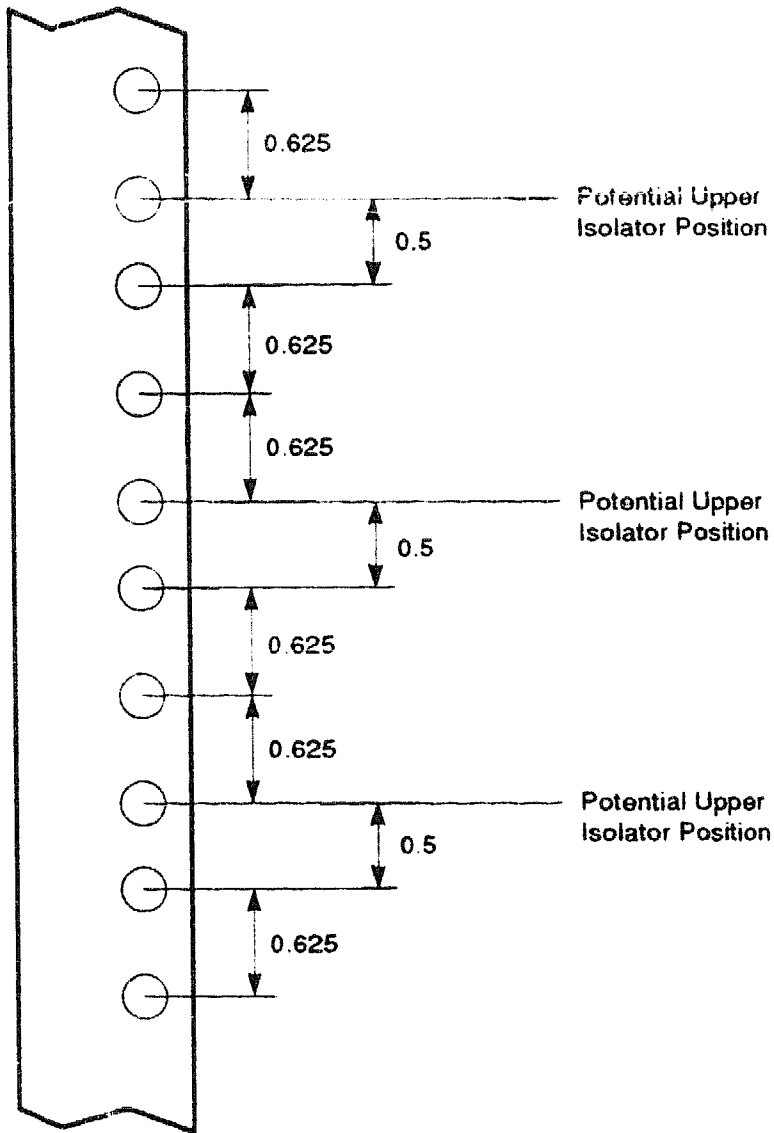
Figure 5: Restriction for Upper Isolator (Early Chassis)
