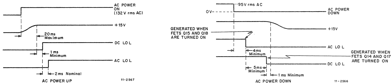
Figure 3-8 5411086 Power Up and Power Down
