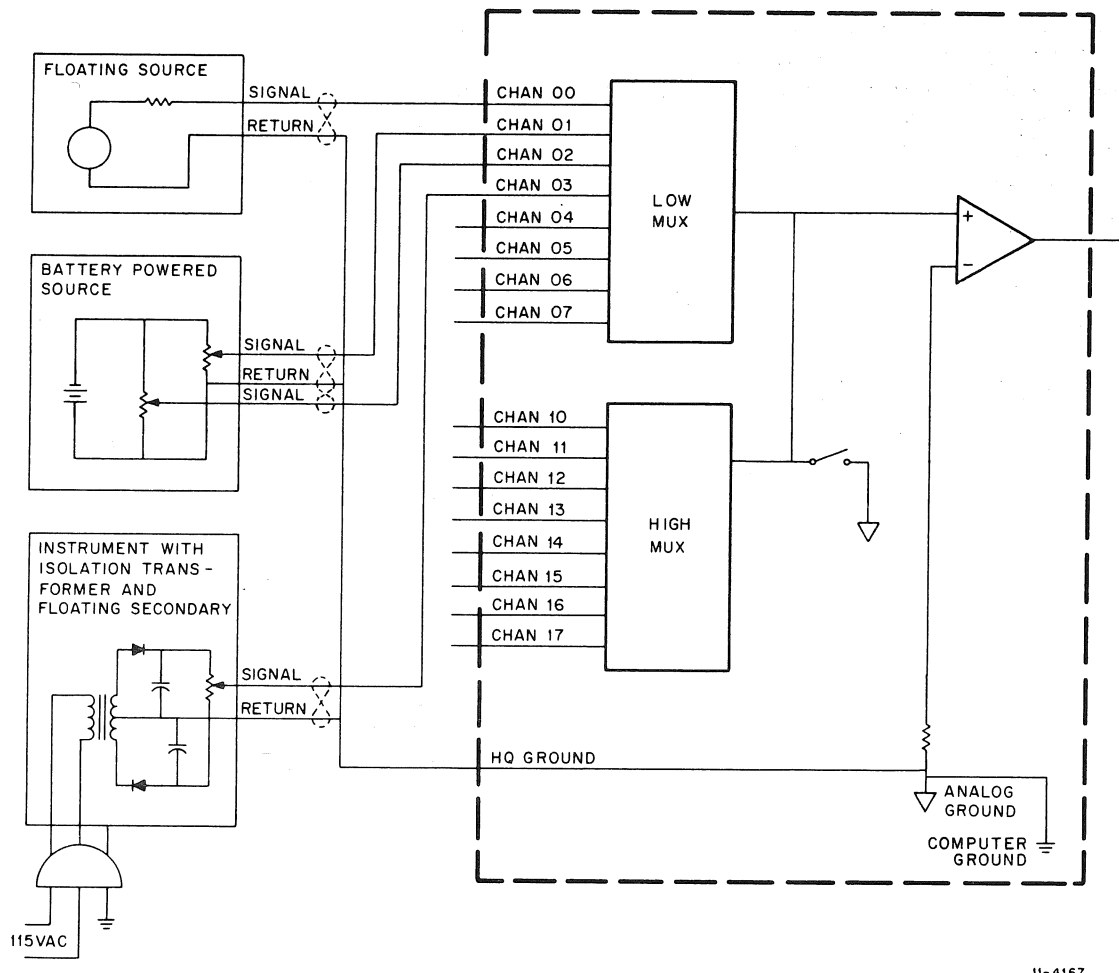
Figure 2-3 Floating ADV11-A Input Signals
