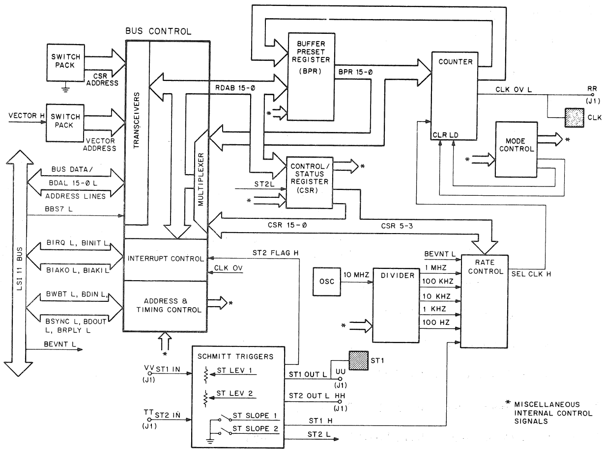
Figure 3-2 K WV11-A Real-Time Clock Block Diagram
