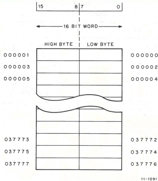
Figure 3-9 Memory Organization for 8K Words
