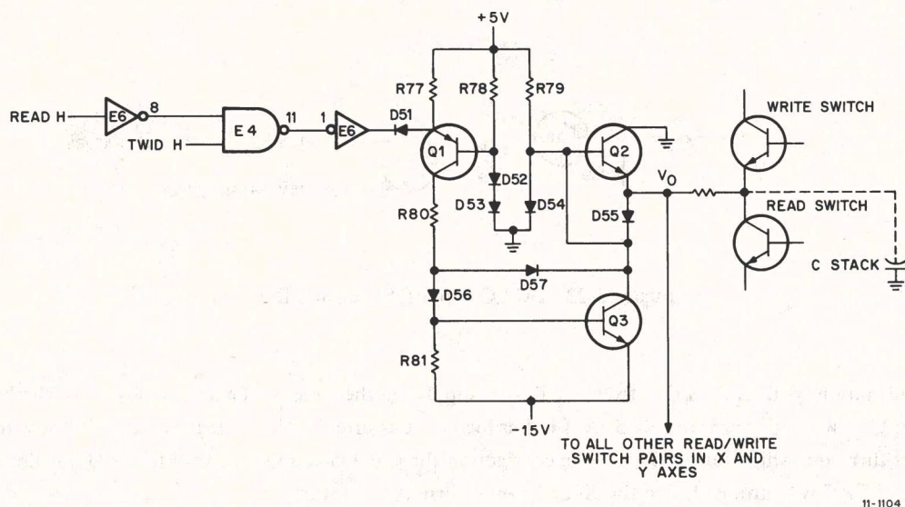
Figure 3-22 Stack Discharge Circuit
