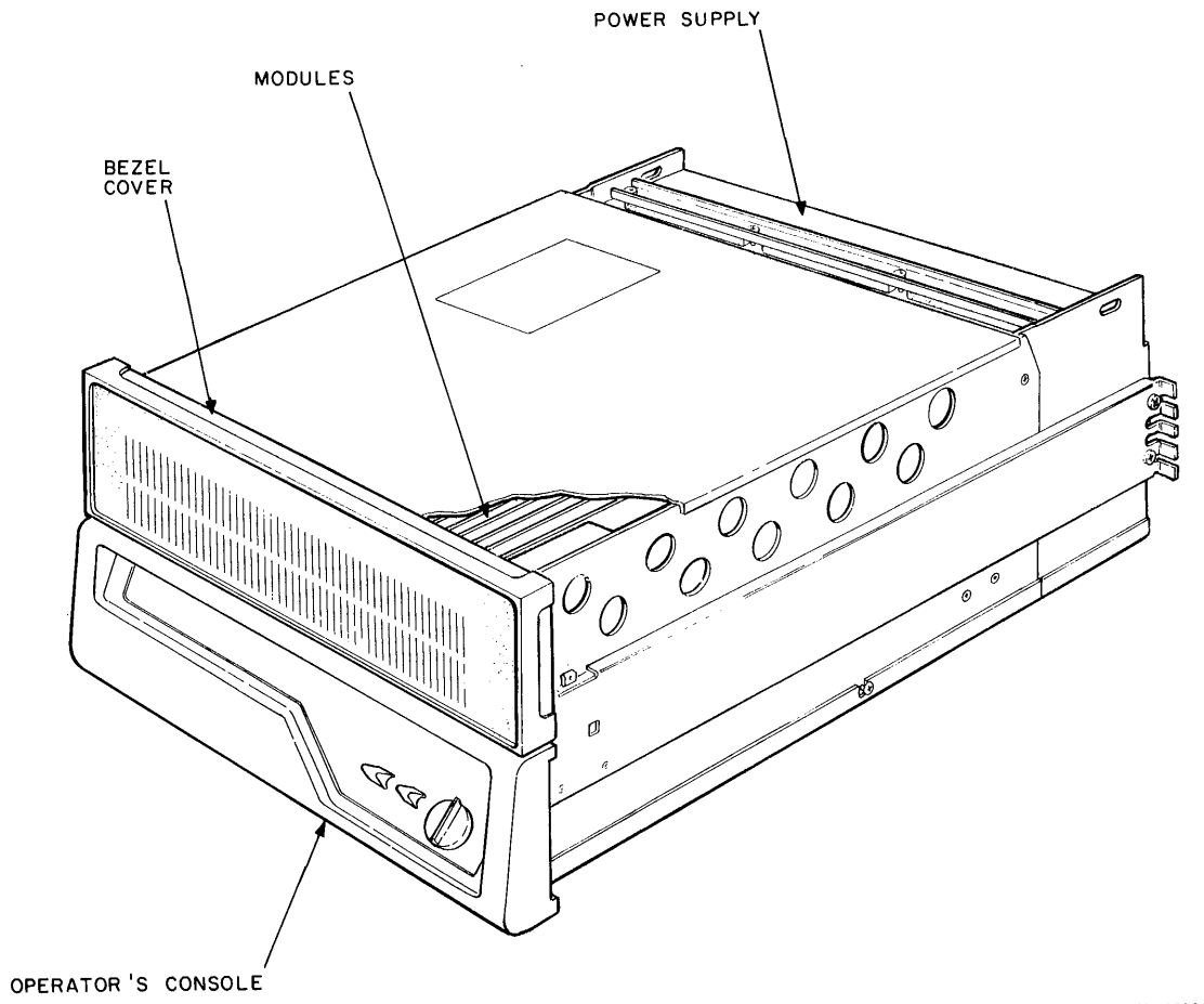
Figure 5-7 Computer Subassemblies of BA11-K Mounting Box
