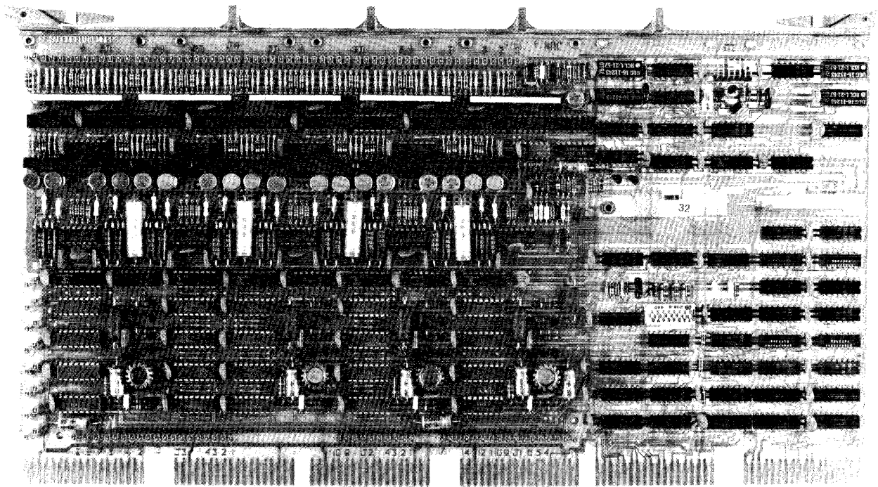
Figure 1-9 MM11-CP Core Memory Module
