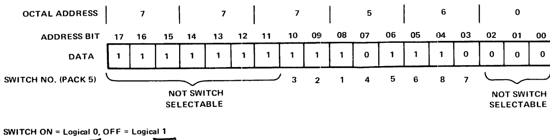
Figure 4-10 DL11-W Device Address Selection
