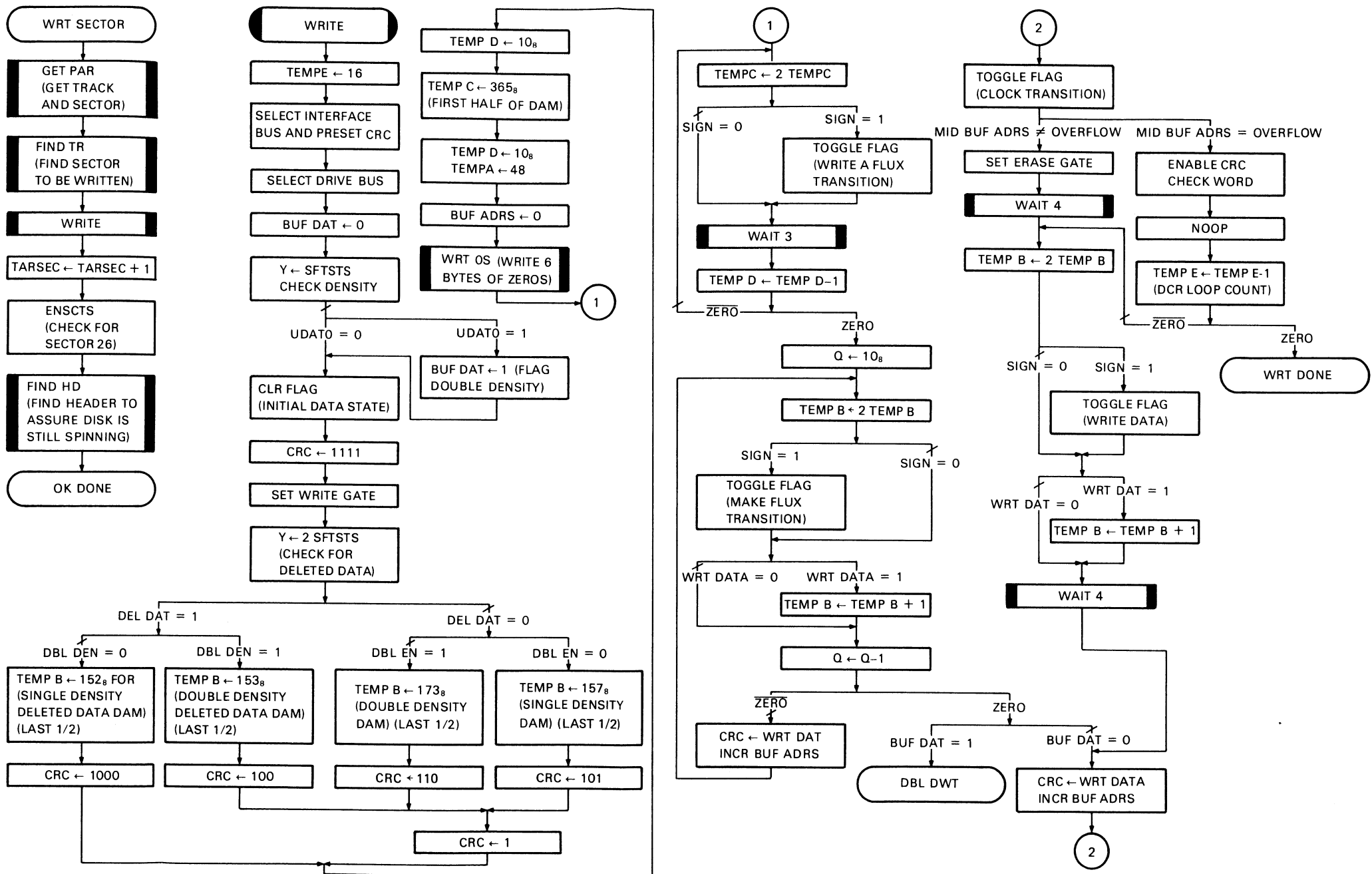
Figure 5-22 Write/Write Sector Subroutine Flowchart (Sheet 1 of 2)
