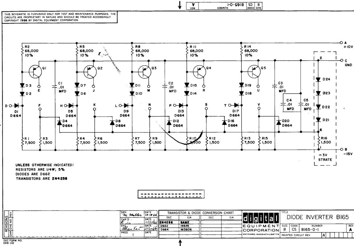
Figure 6-5 Diode Inverter B165
