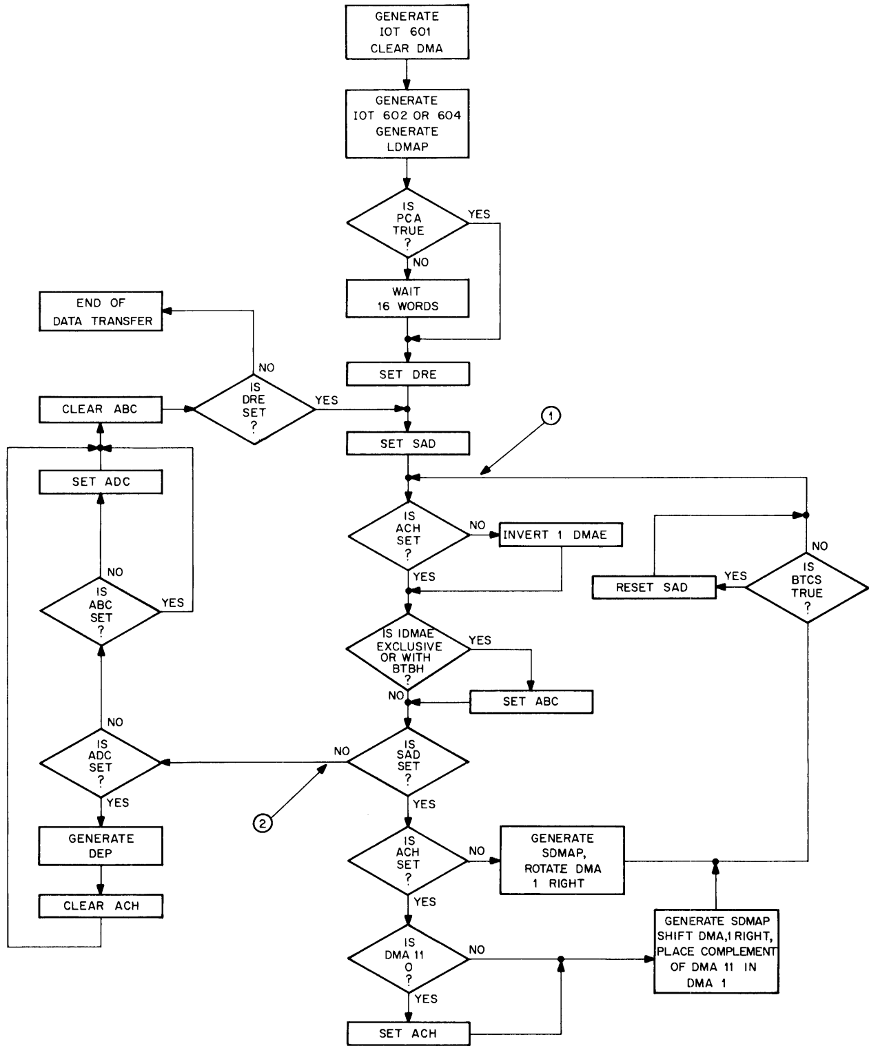
Figure 3-8 Address Flow Diagram
