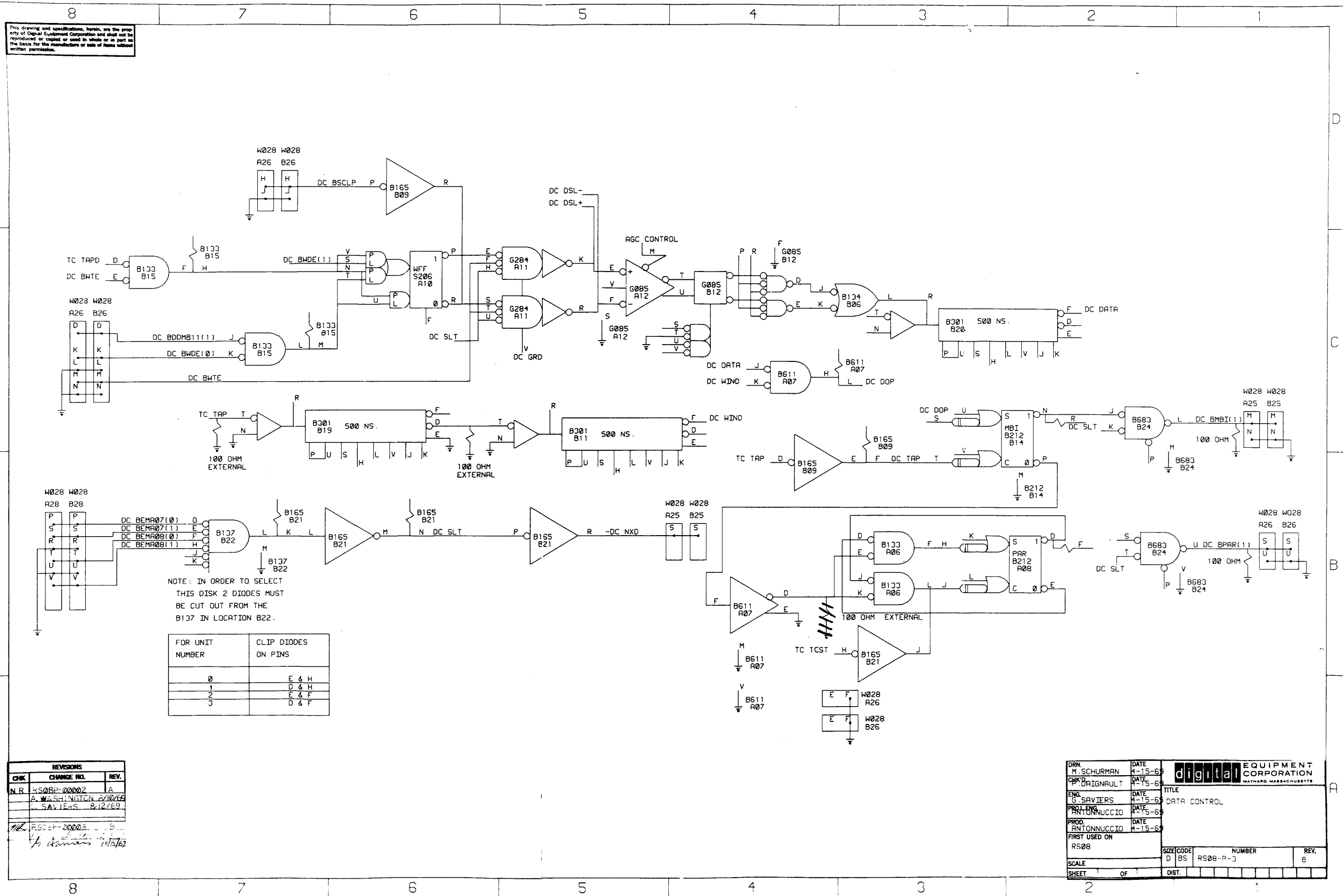
Figure 6-40 Data Control
