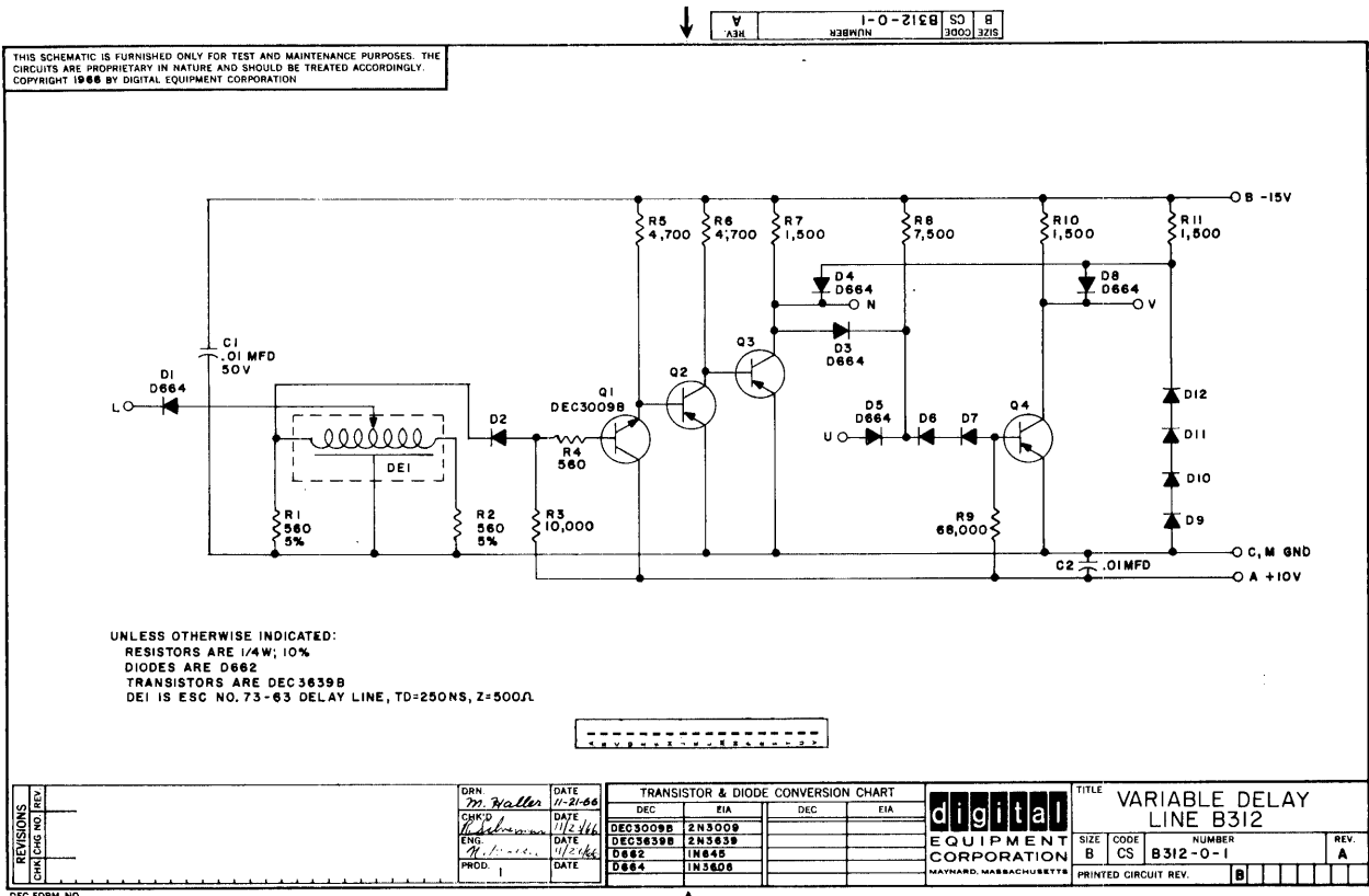
Figure 6-9 Variable Delay Line B312
