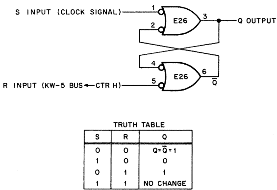
Figure 3-4 RS Latch, Logic Diagram
