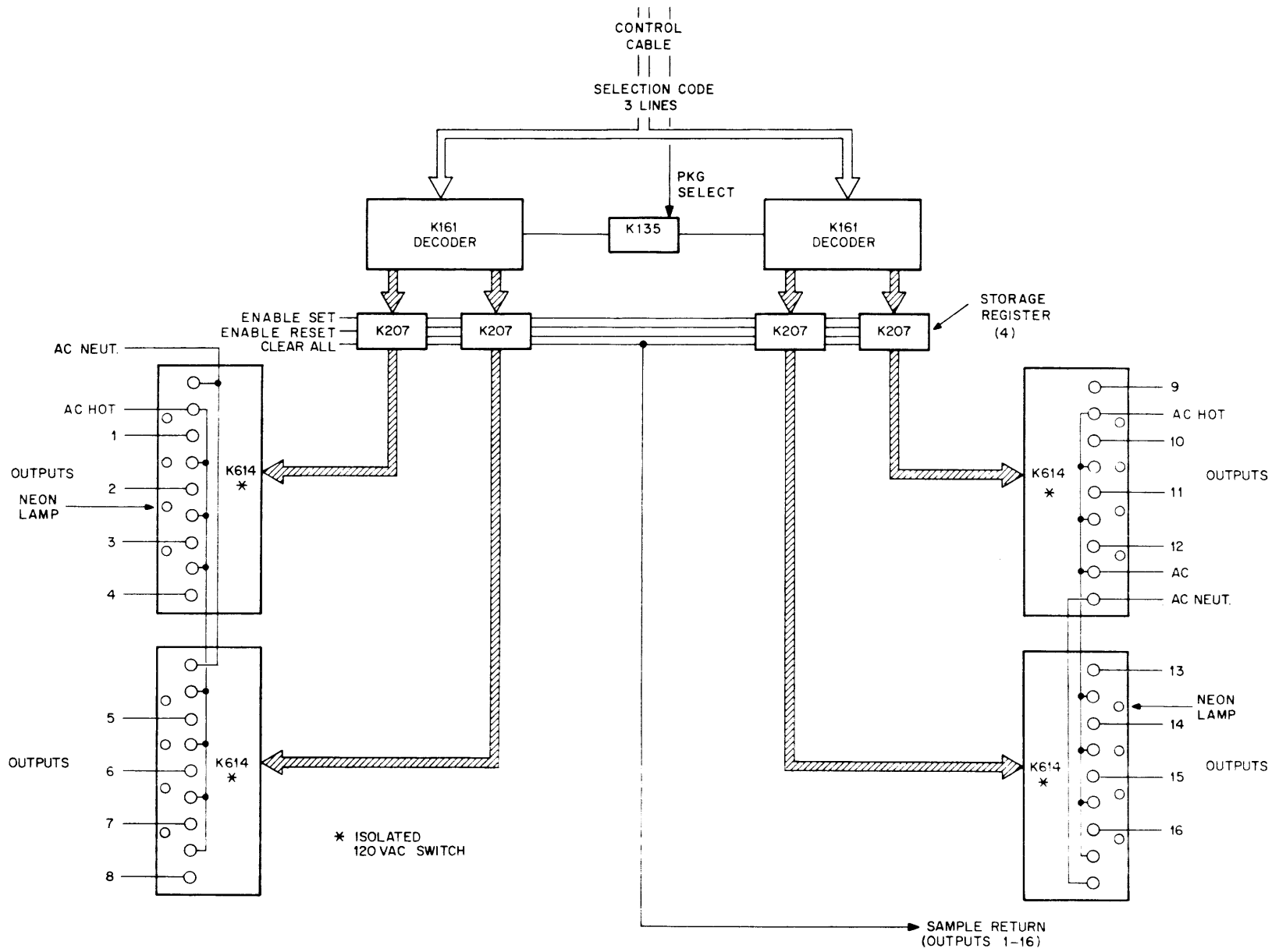
Figure 3-4 O Box Selection System
