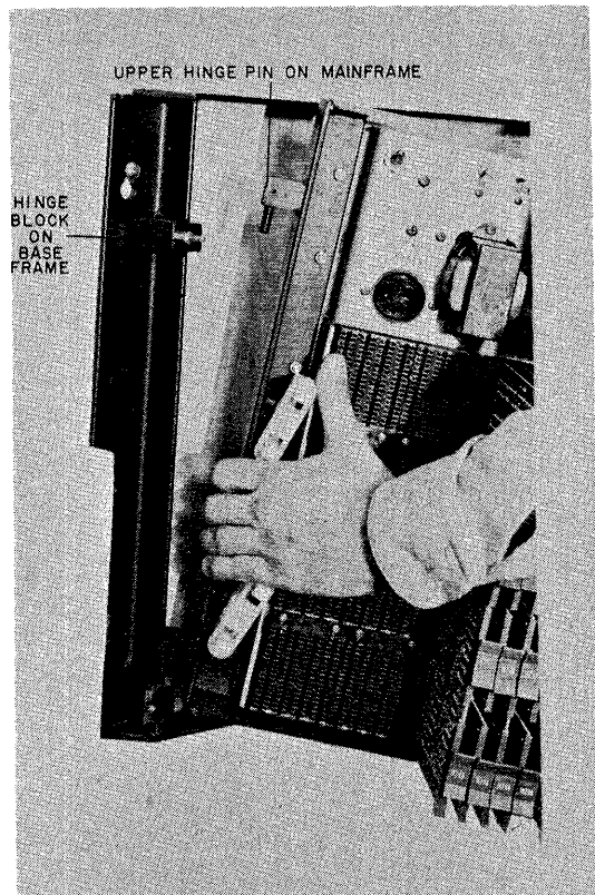
Figure 11-4 Control Unit Mainframe Mounting
