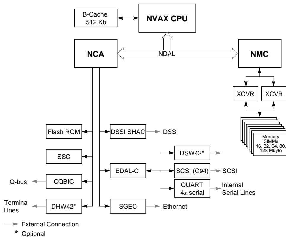
Figure 1-1 Block Diagram of the VAX 4000 Model 105A/106A System
