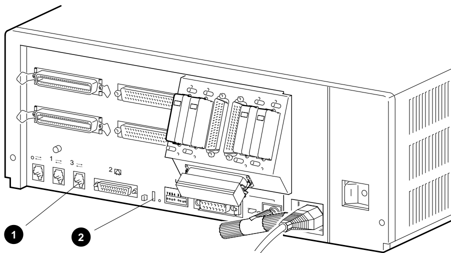
Figure 2-2 Console Port
