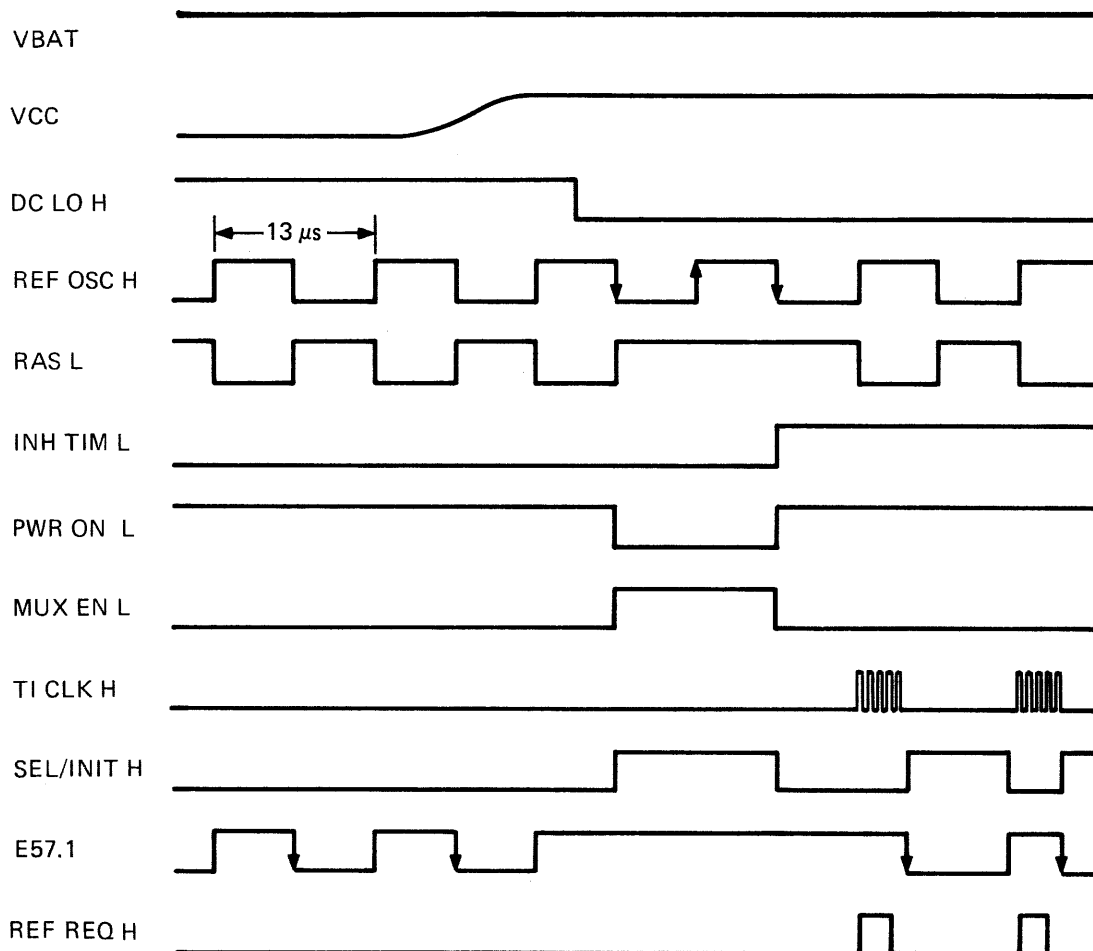
Figure 3-12 End of Battery Backup Mode
