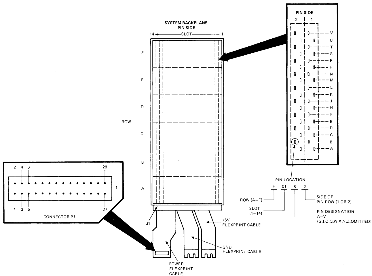
Figure 3-2 Backplane Assembly, Pin Designations
