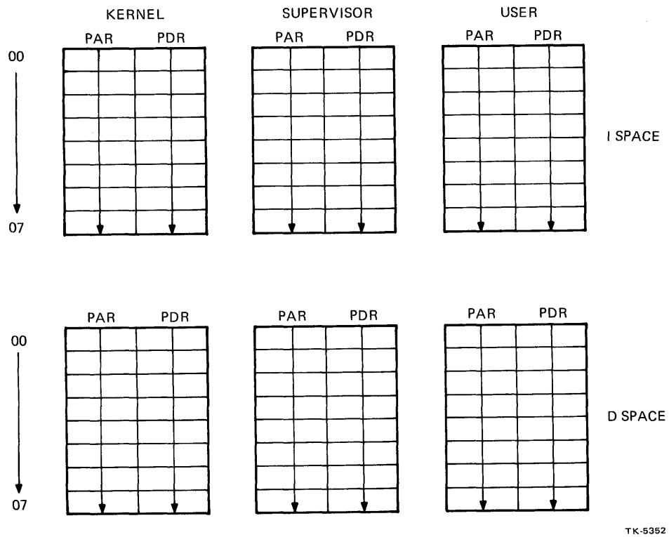
Figure 6-32 Memory Management Relocation Registers
