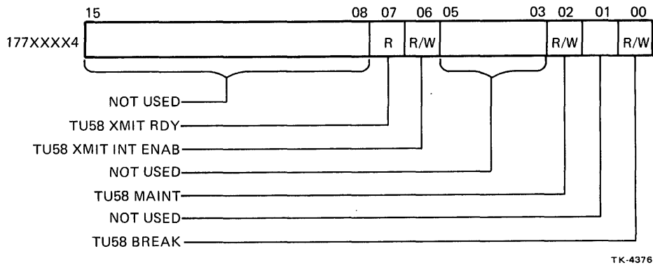
Figure 6-53 TU58 Transmitter Status Register
