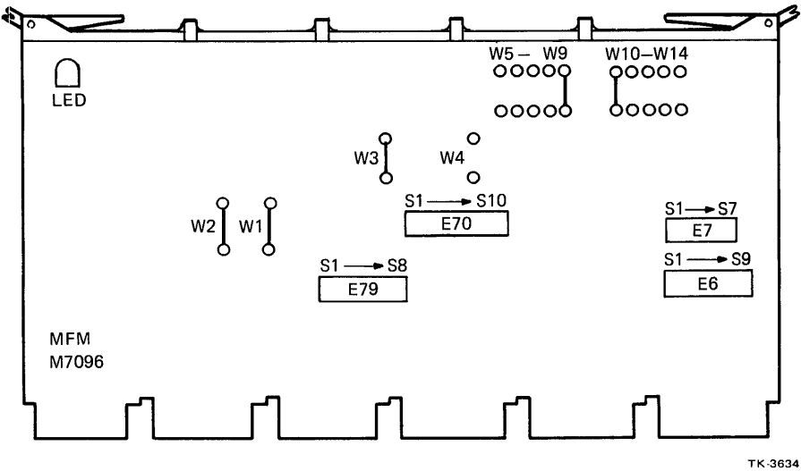
Figure 3-6 MFM Jumper Lead Locations Switches and LED Indicator
