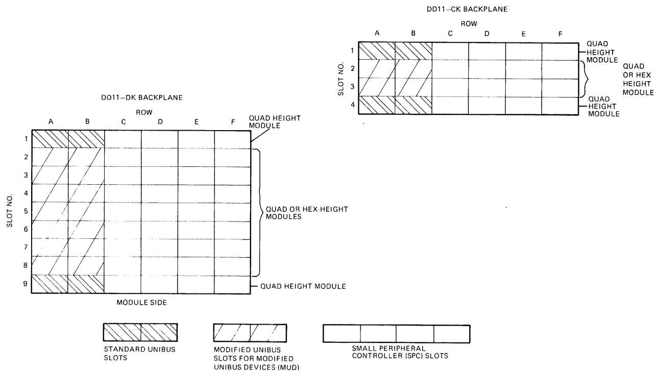
Figure 5-19 Optional Backplane Slot Assignments
