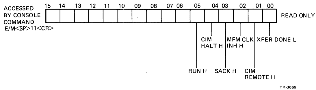
Figure 2-13 Signal Register Format
