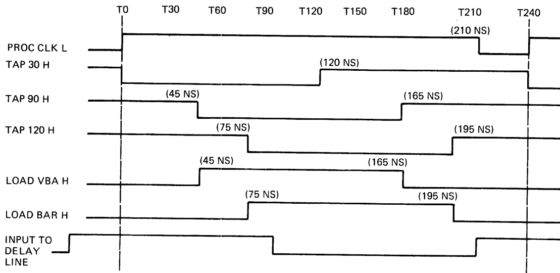
Figure 6-18 PDP-11/44 System Clock Long Cycle Timing Diagram
