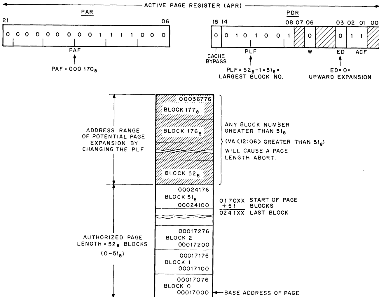
Figure 6-34 Upward Expansion
