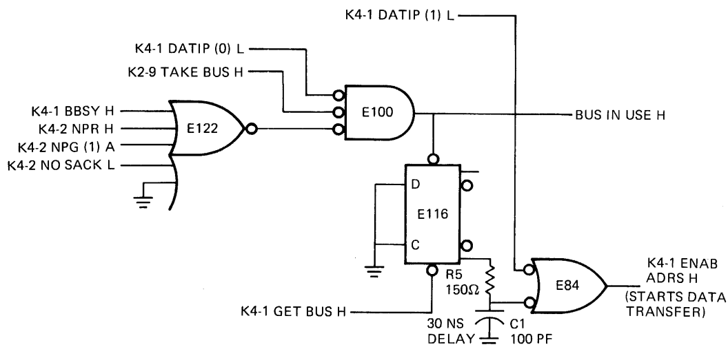
Figure 6-10 UNIBUS Synchronizer
