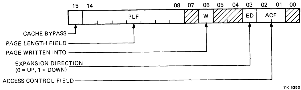
Figure 6-33 Page Descriptor Register
