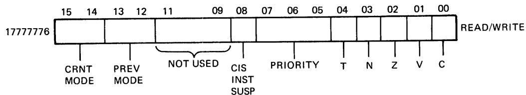
Figure 2-2 PSW Register Format
