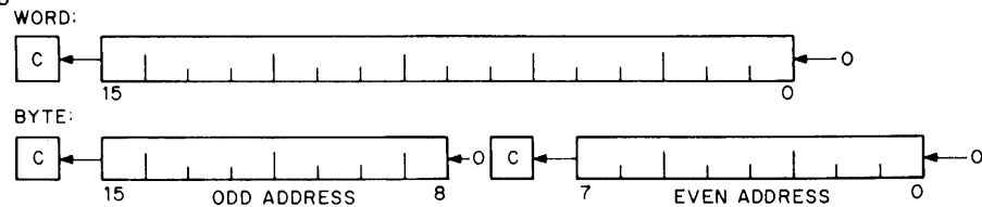
Figure 6-6 Rotate Instructions
