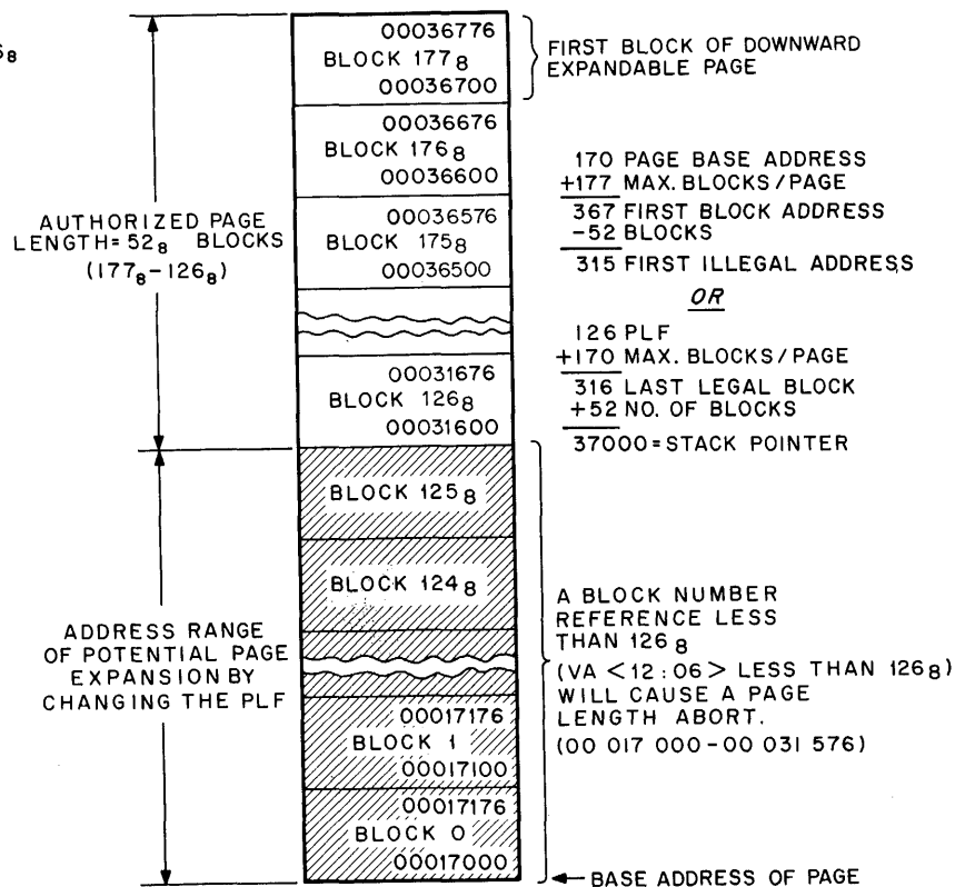
Figure 6-35 Downward Expansion
