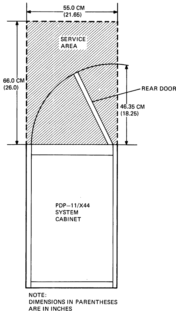
Figure 4-18 PDP-11X44 System Cabinet Service Area
