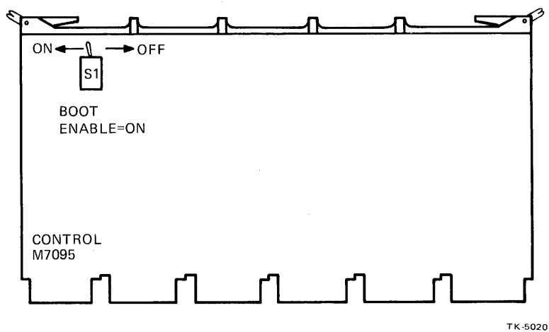
Figure 3-11 Control Module, Bootstrap Control Switch
