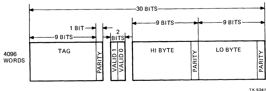
Figure 6-58 Cache Memory Organization
