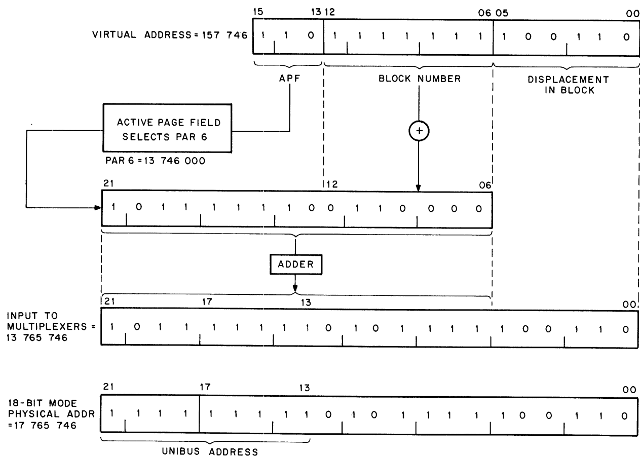
Figure 6-29 18-Bit Mapping: UNIBUS Address
