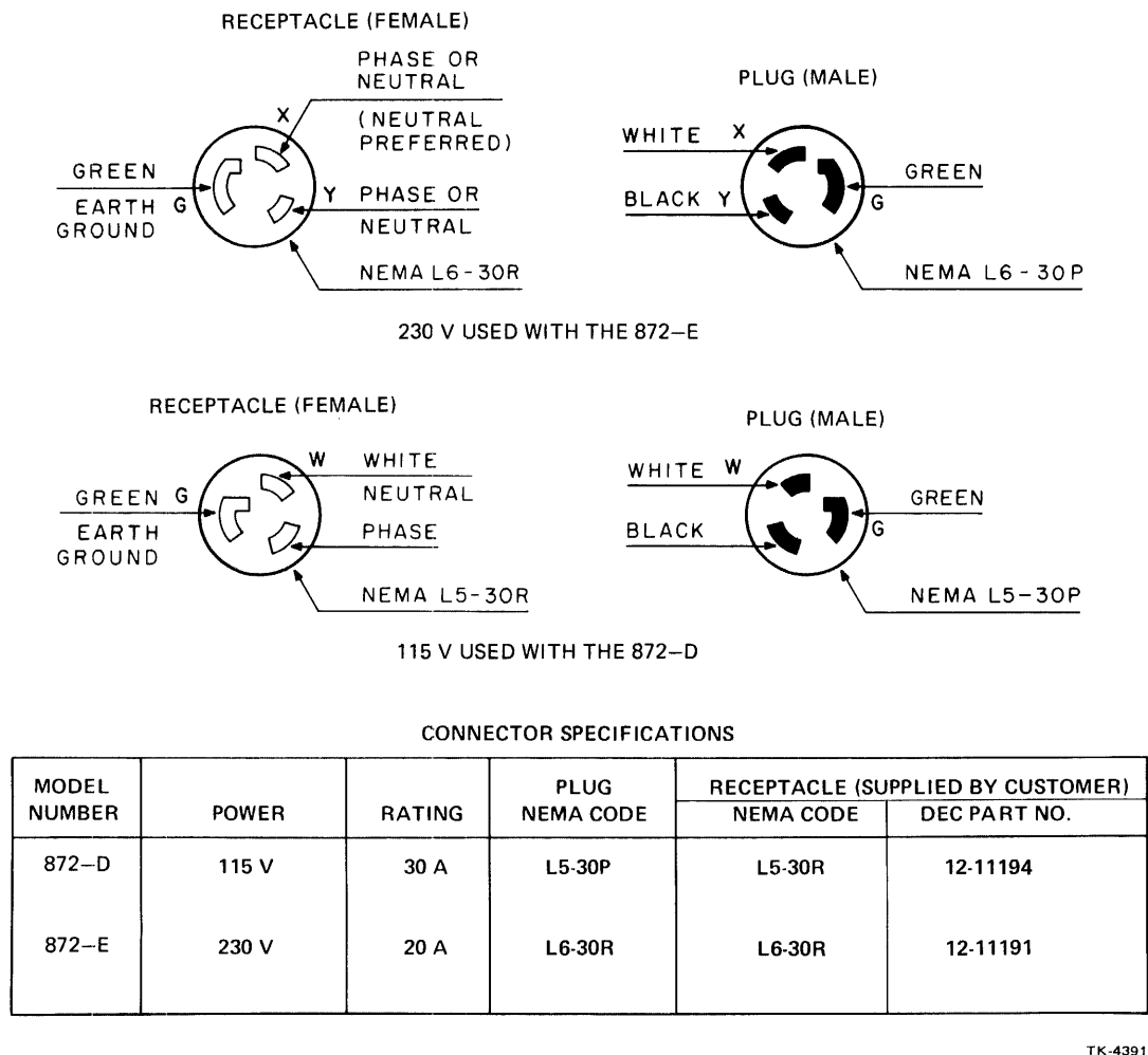
Figure 4-10 872-D, -E Power Controller Input Power Specifications
