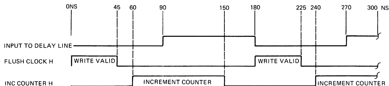
Figure 6-60 Cache Flush Timing Diagram
