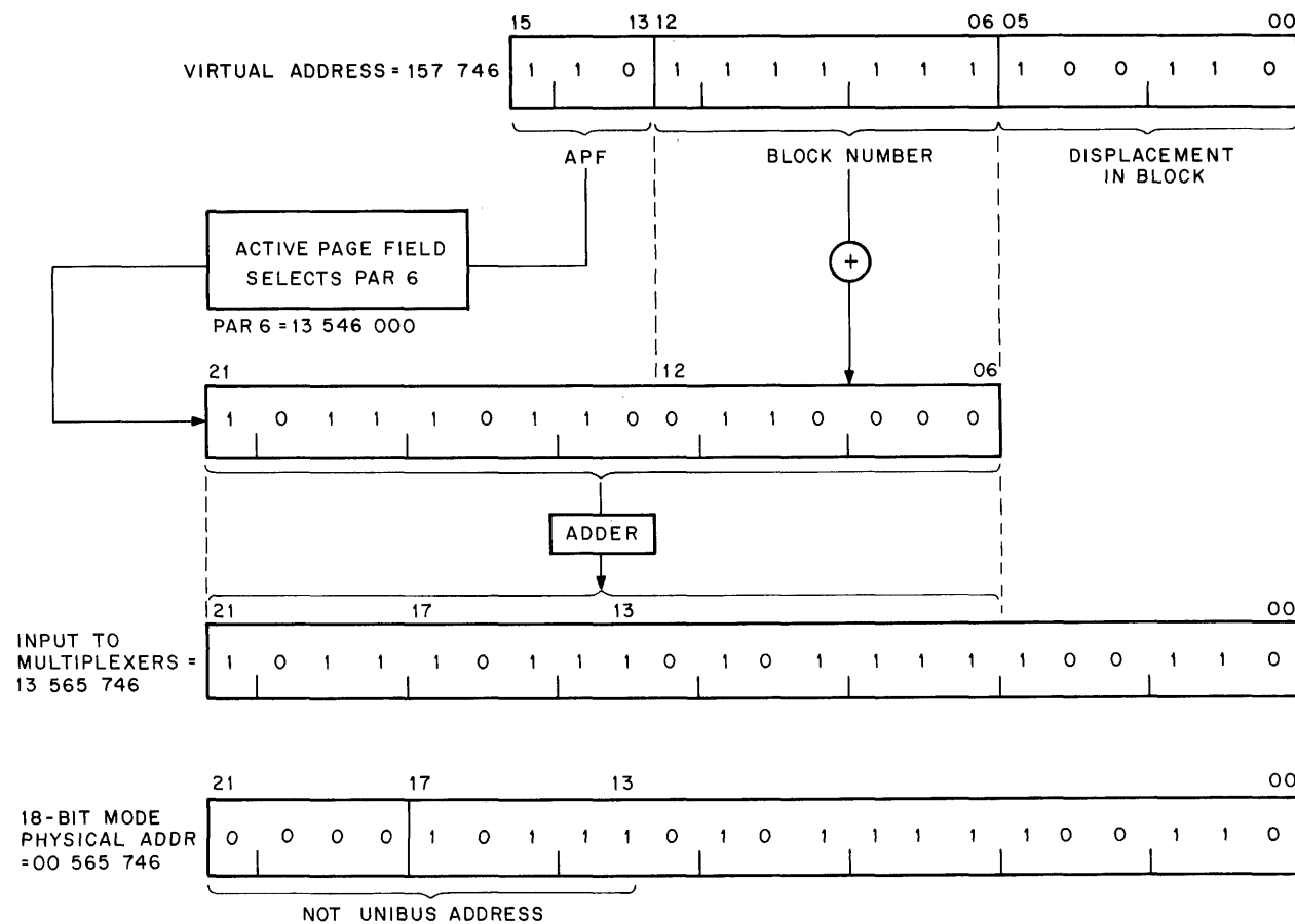
Figure 6-28 18-Bit Mapping: Memory Address
