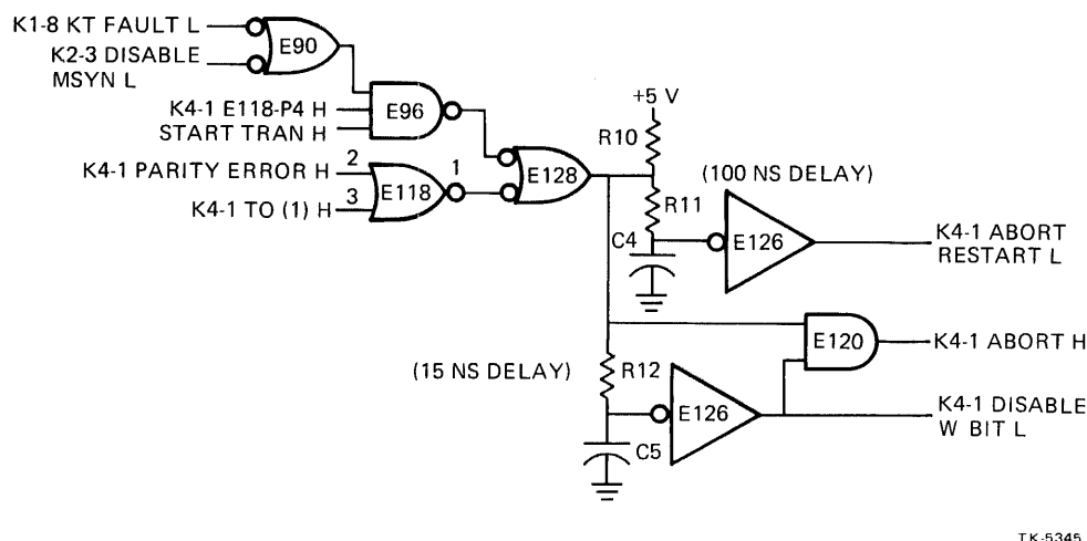
Figure 6-16 Generation of ABORT RESTART L and ABORT H
