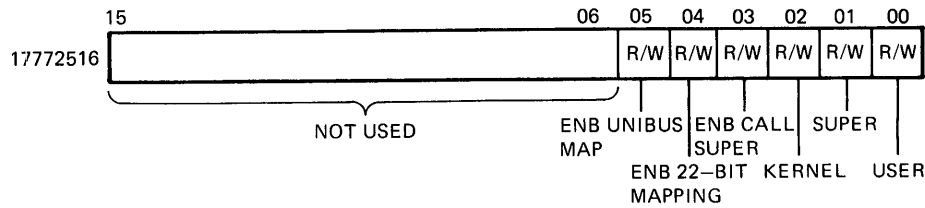
Figure 2-23 Memory Management SR3 Format
