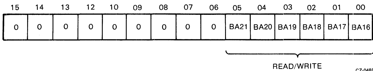
Figure 4-9 BAE Register
