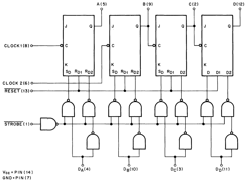
Figure A-3 8281 DC 4-Bit Binary Counter/Storage Element
