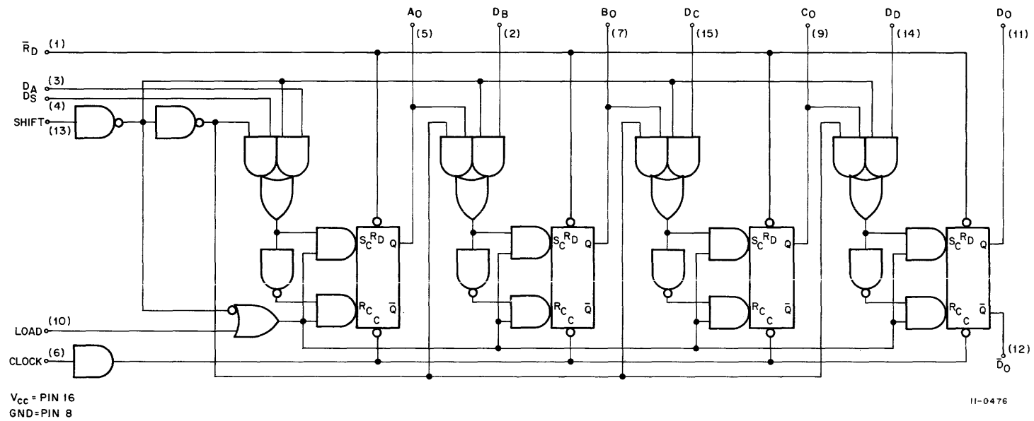
Figure A-2 8271 4-Bit Shift Register
