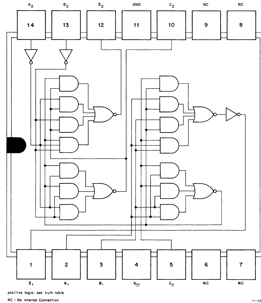
Figure A-1 7482 2-Bit Binary Full Adders
