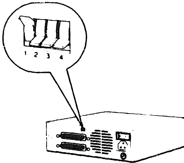
Figure 4-7. ID switch setting for the RRD40 optical compact disc drive
