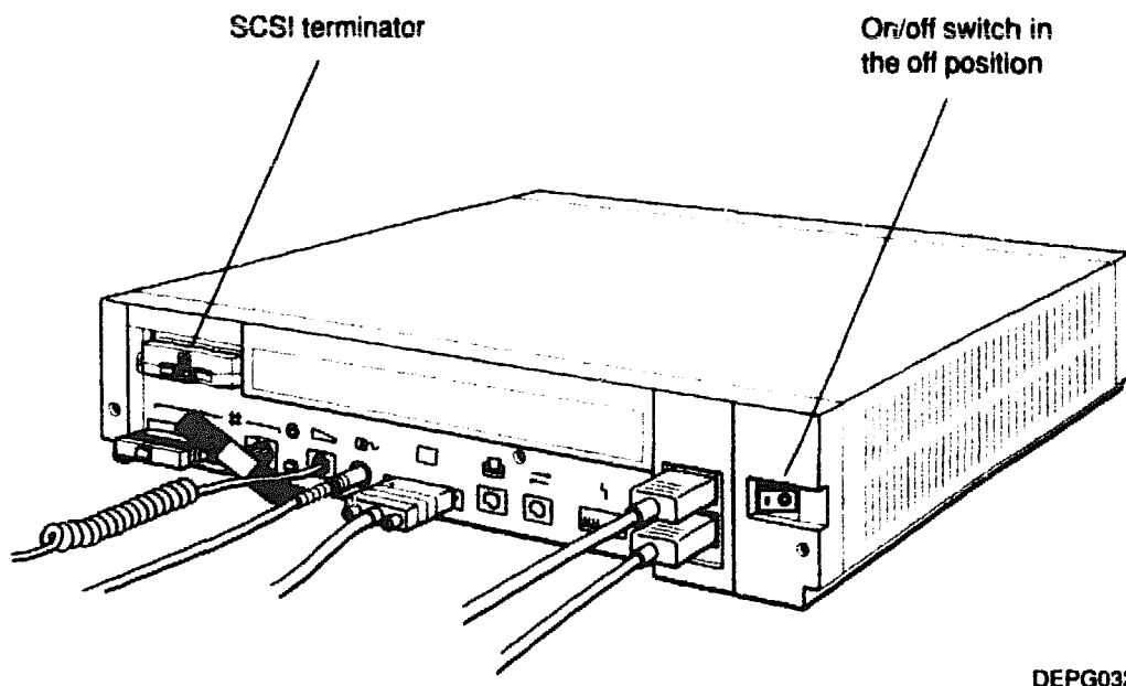
Figure 7-6. Checking the SCSI terminator
