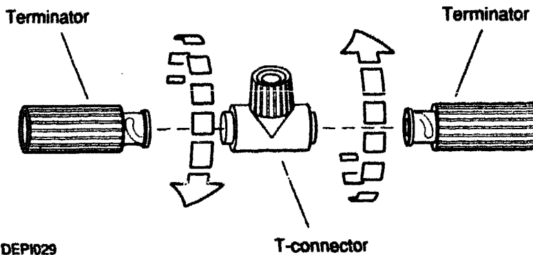
Figure 2-6. Attaching terminators to the T-connector
