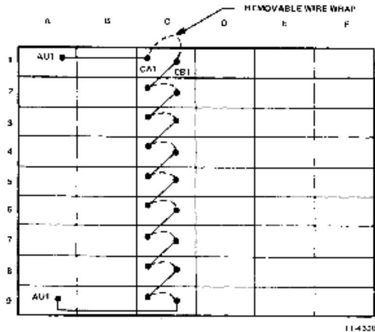
Figure 4-6 NPG Signal Path
