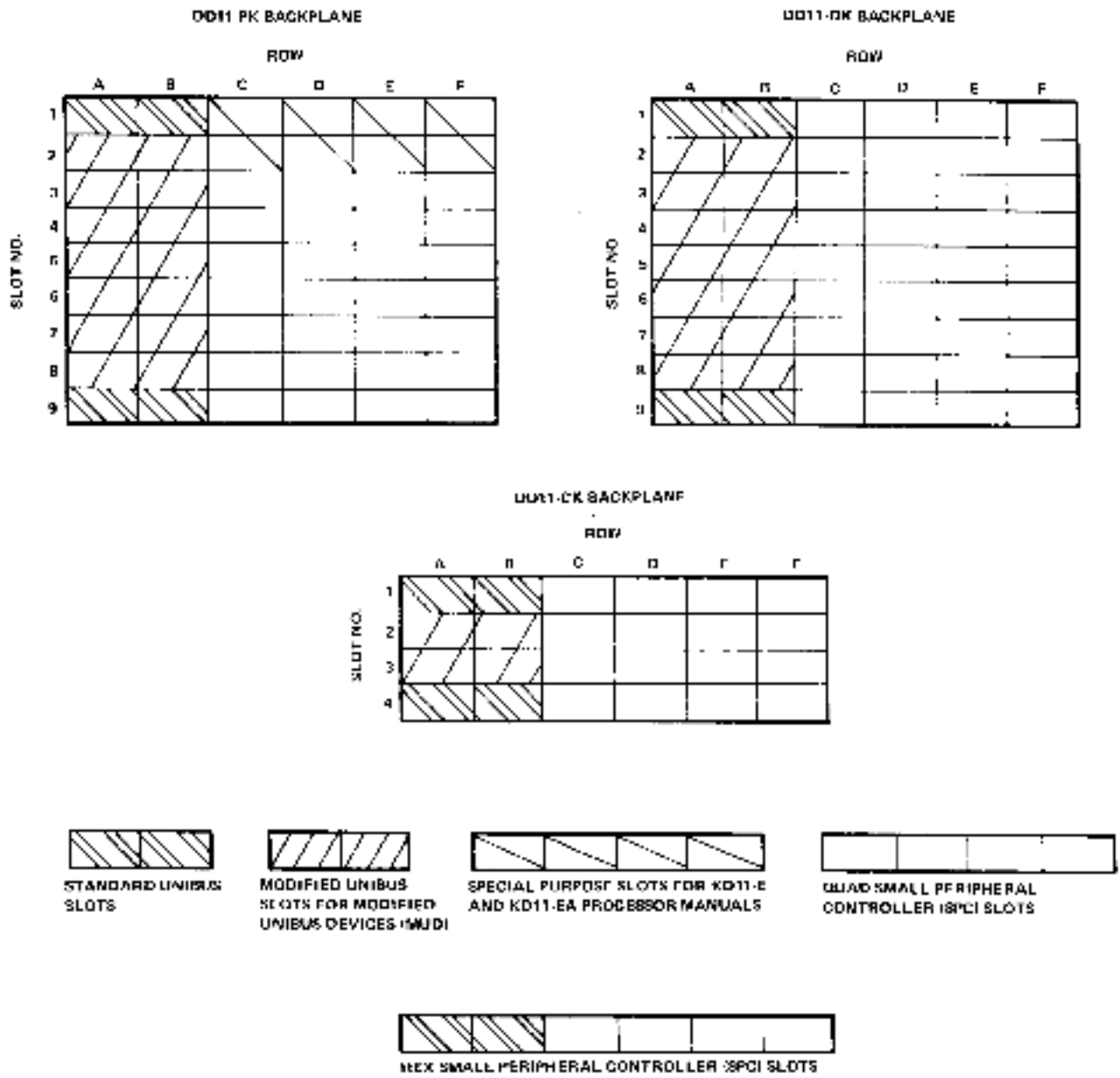
Figure 4-1 PDP-11/34 Backplanes
