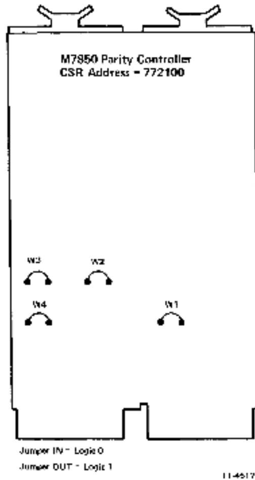
Figure 5-9 Typical Jumper Placement and Switch Settings of Modules (Sheet 1 of 9)
