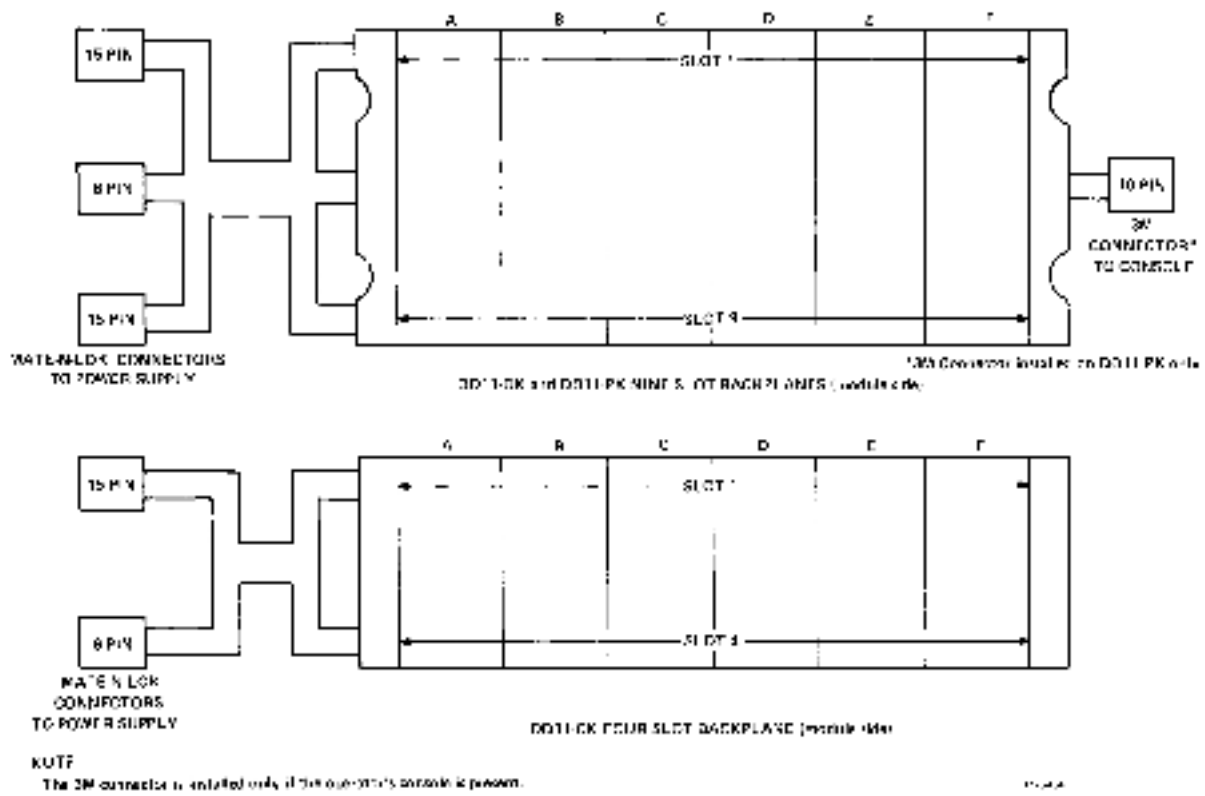
Figure 5-8 Backplane Connectors
