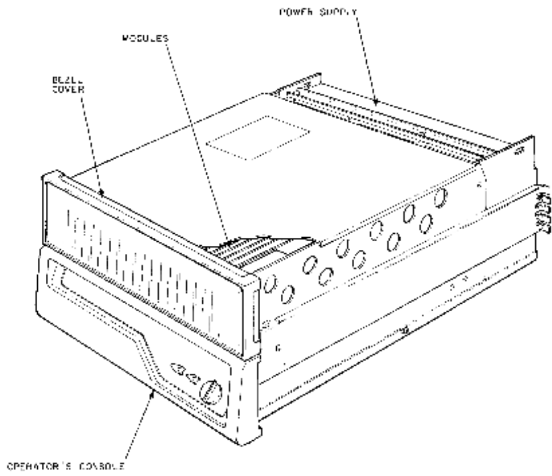
Figure 5-7 Computer Subassemblies of BA11-K Mounting Box
