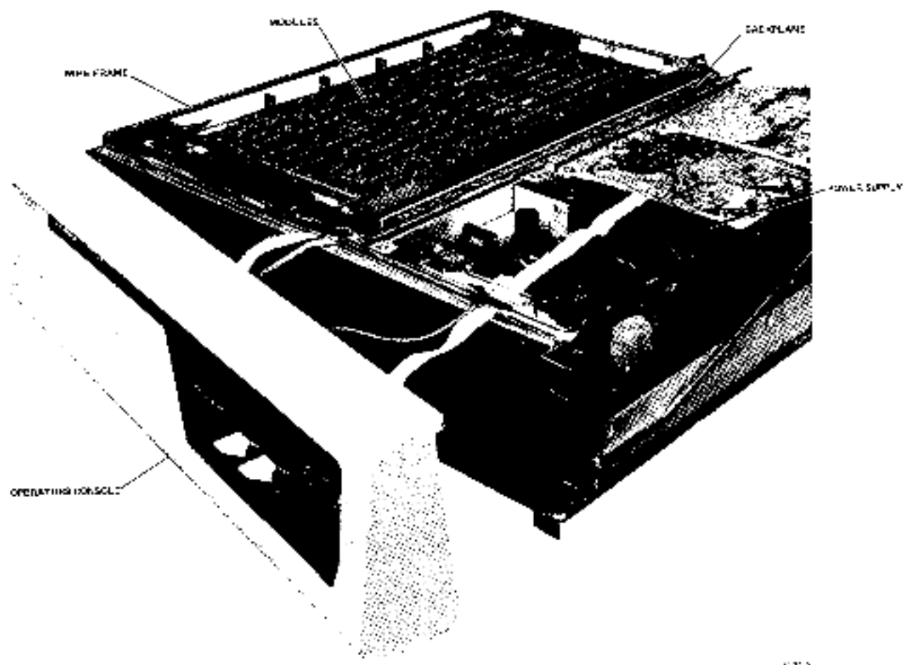
Figure 5-6 Computer Subassemblies of BA11-L Mounting Box
