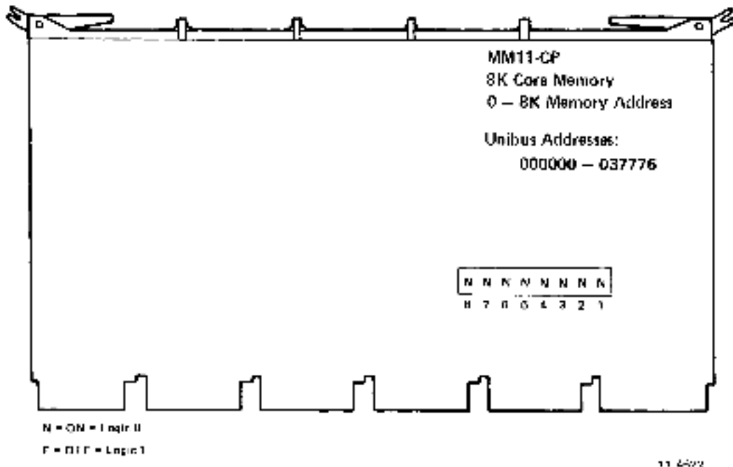
Figure 5-9 Typical Jumper Placement and Switch Settings of Modules (Sheet 7 of 9)
