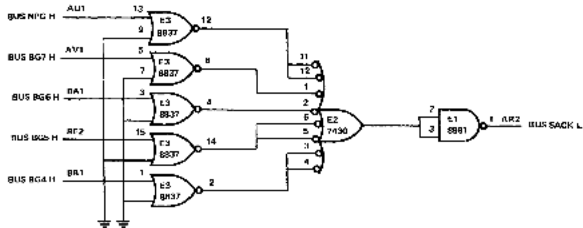
Figure 3-3 M9302 Sack Turnaround Logic
