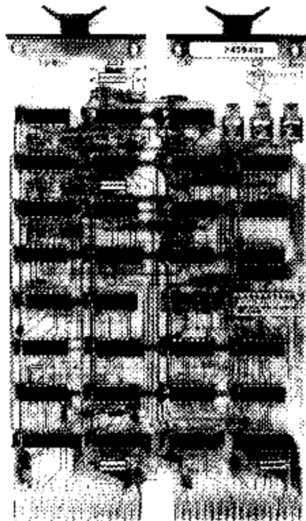
Figure 1-6 M9301 Bootstrap/Terminator Module
