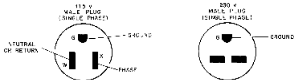
CONNECTOR SPECIFICATIONS
