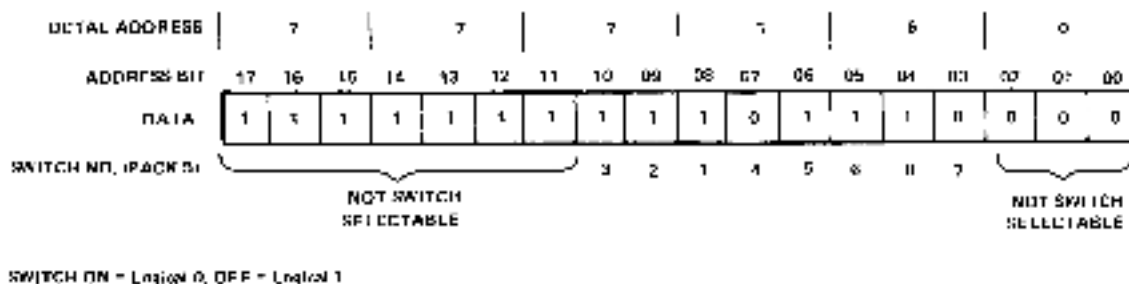
Figure 4-10 DL11-W Device Address Selection
