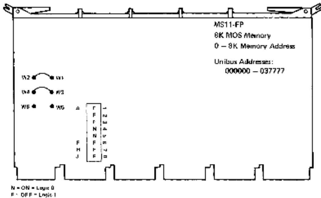
Figure 5-9 Typical Jumper Placement and Switch Settings of Modules (Sheet 5 of 9)
