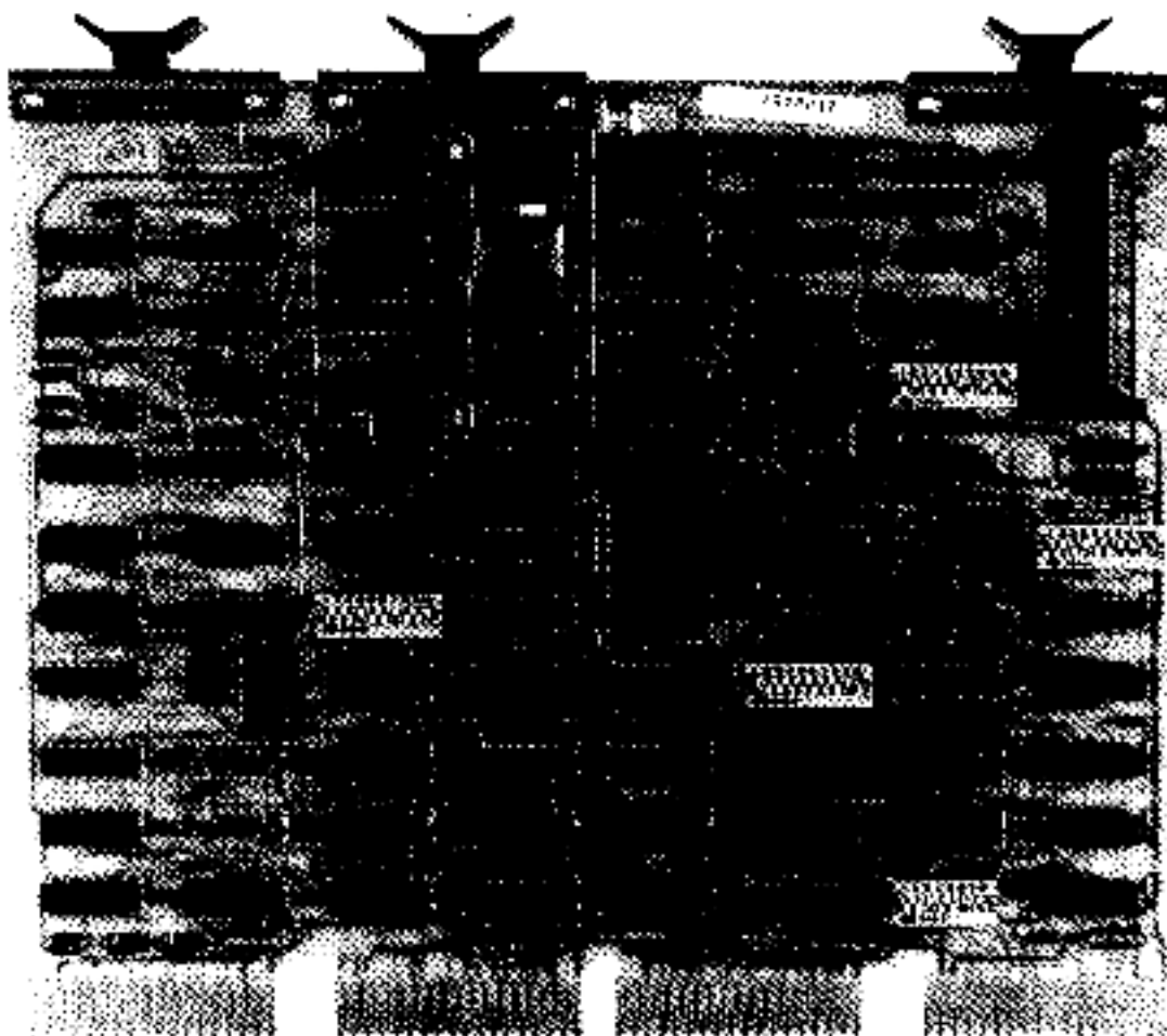
Figure 1-12 DL11-W Serial Line Interface and Real-Time Clock
