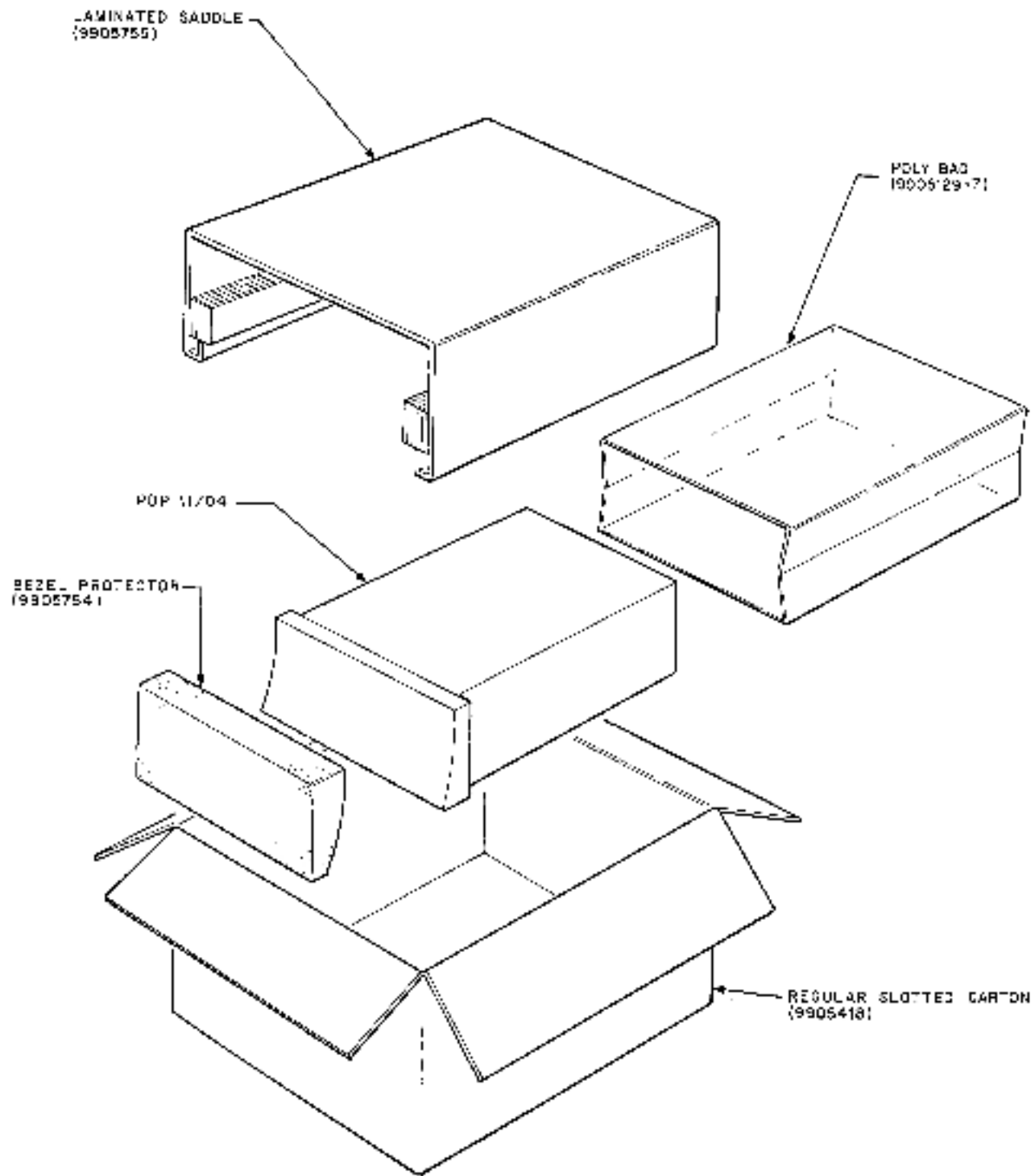
Figure 5-4 Packaging of PDP-11/34 [13.3 cm (5-1/4 inch Box)]
