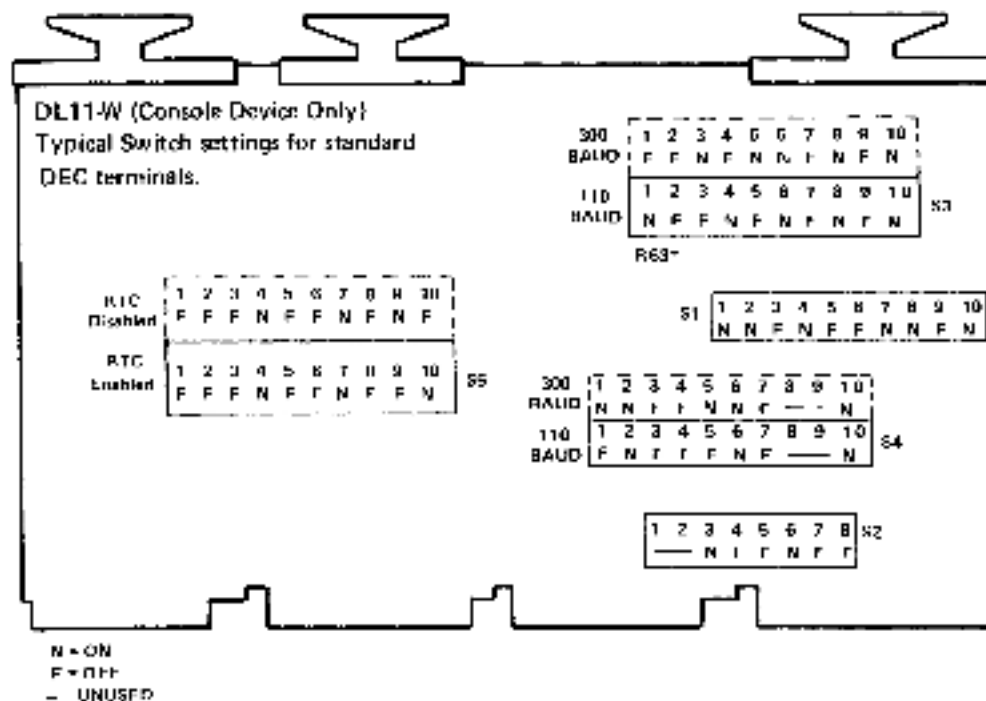
Figure 5-9 Typical Jumper Placement and Switch Settings of Modules (Sheet 9 of 9)
