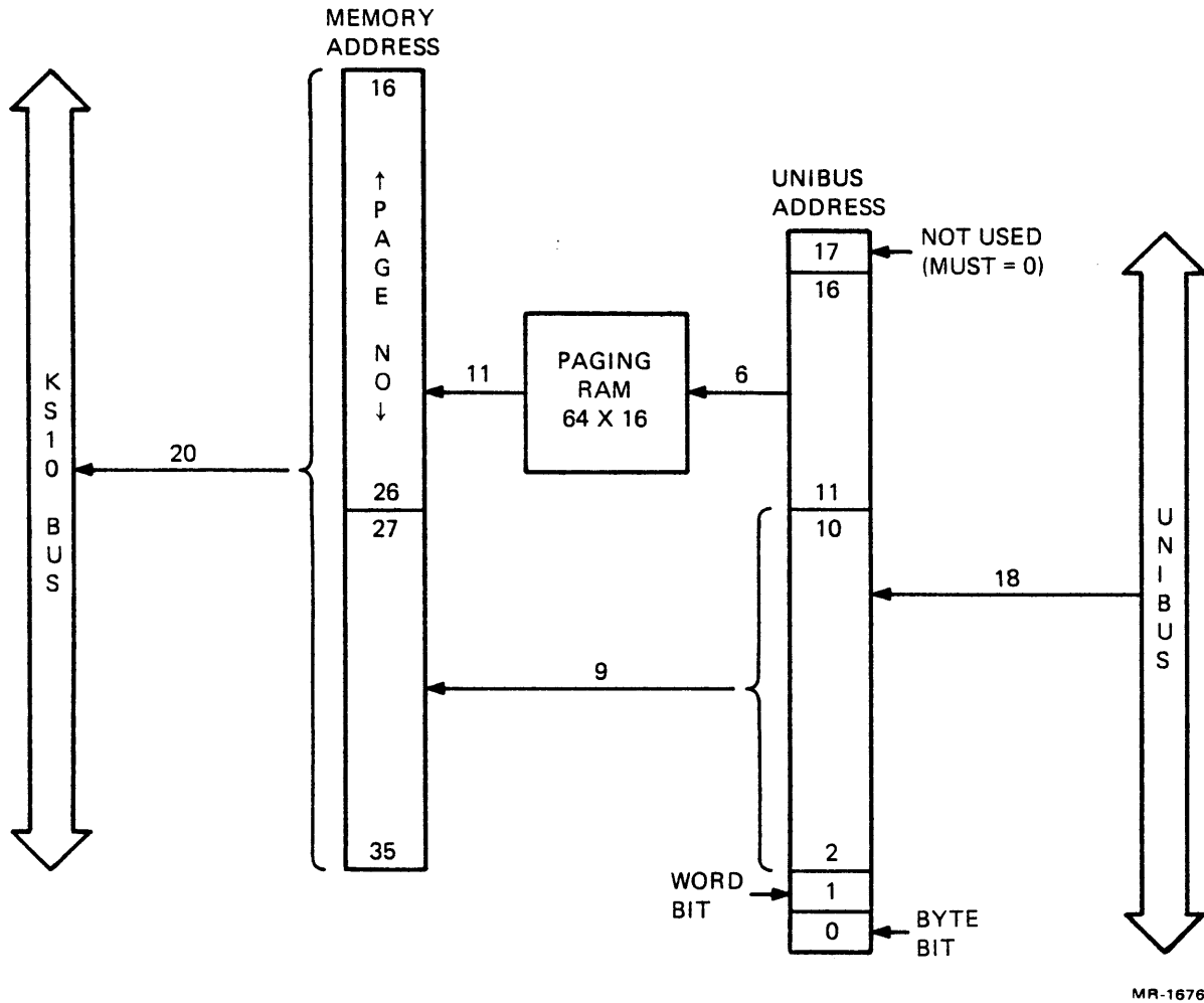
Figure 3-2. KS10 Address Translation
