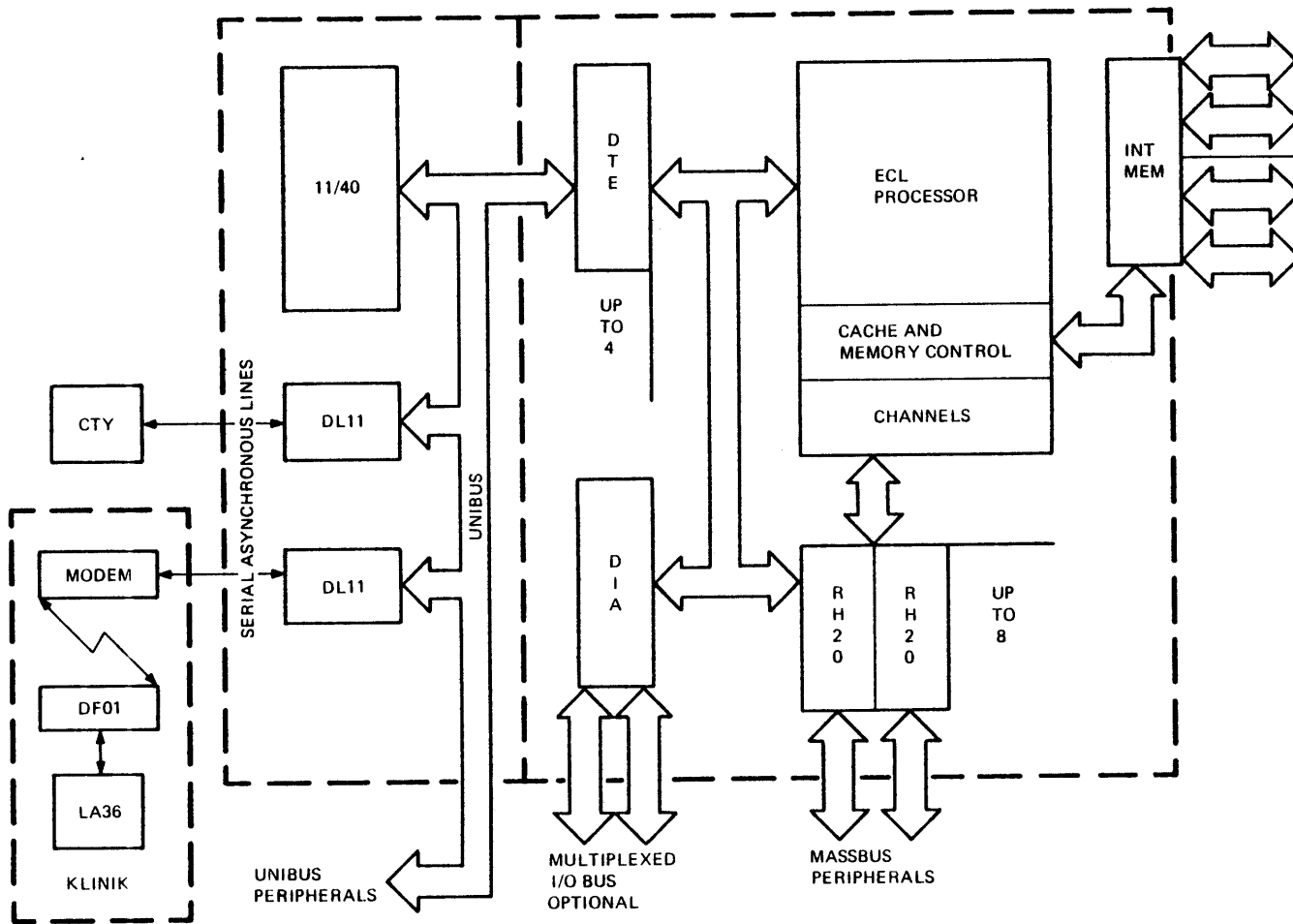
Figure 2-2. Fully Configured KL10-E Central Processing Unit
