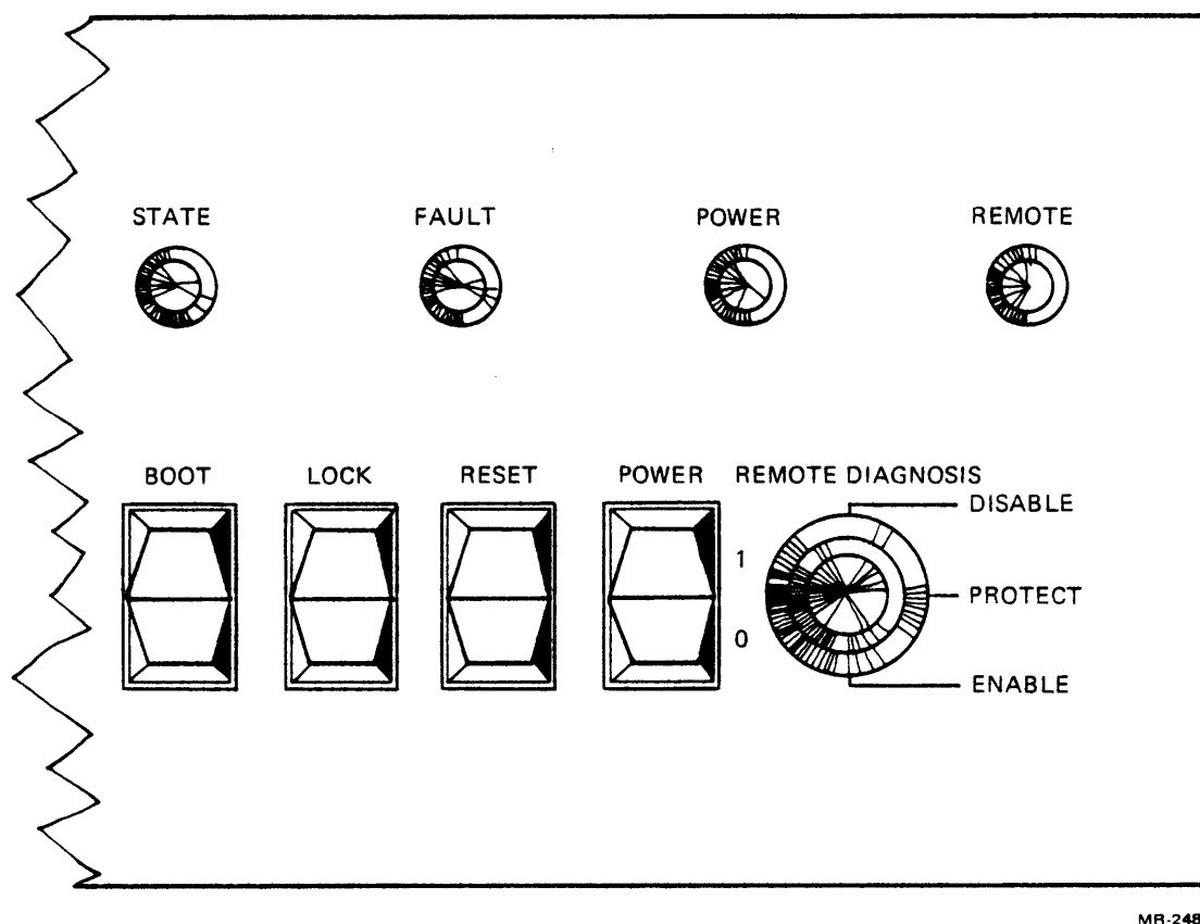
Figure 7-1. KS10 Switch and Indicator Panel
