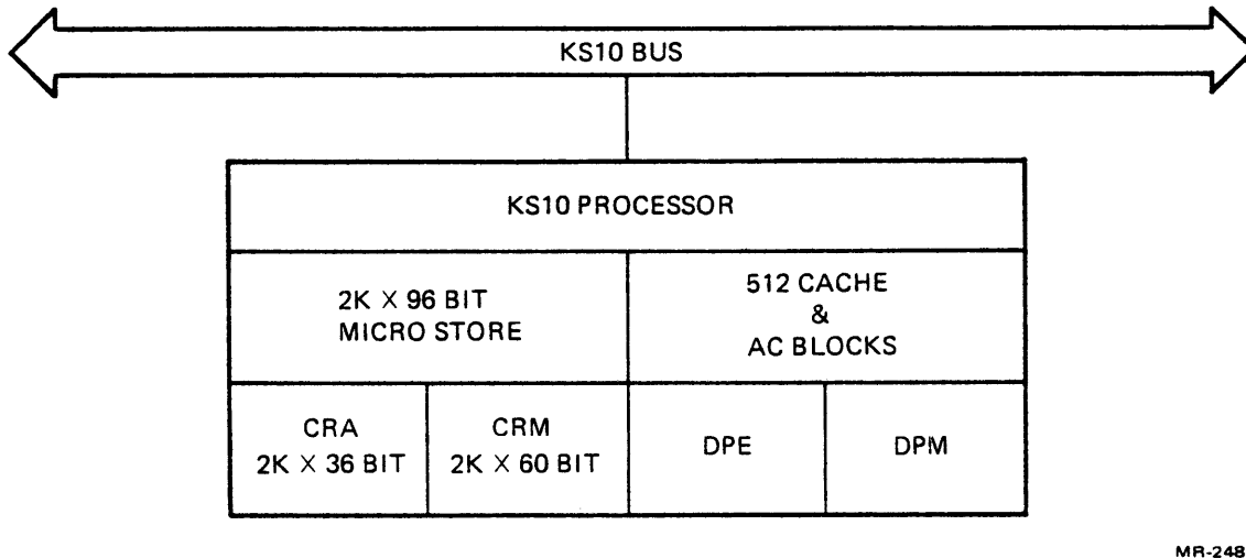
Figure 2-3. KS10 Central Processing Unit
