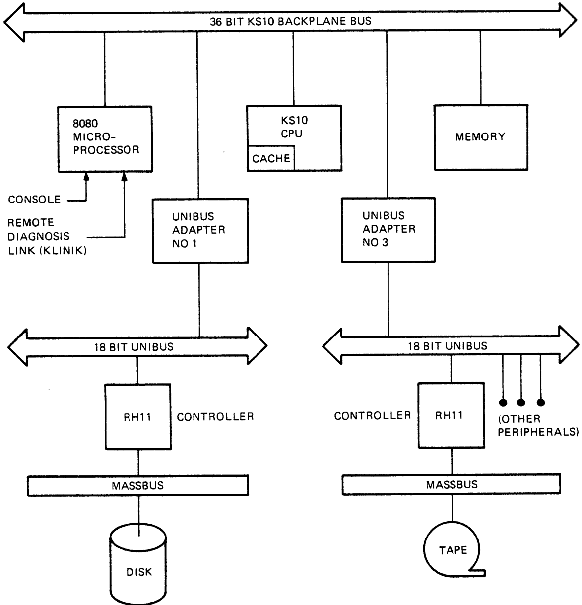
Figure 1-2. 2020 System Architecture
