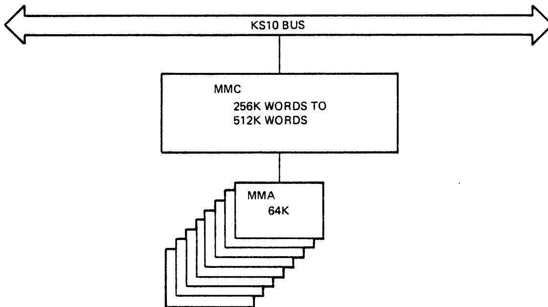
Figure 2-12. Memory Subsystem
