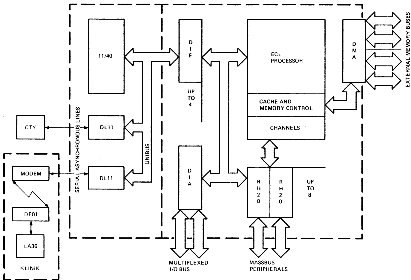
Figure 2-1. Fully Configured KL10-D Central Processing Unit
