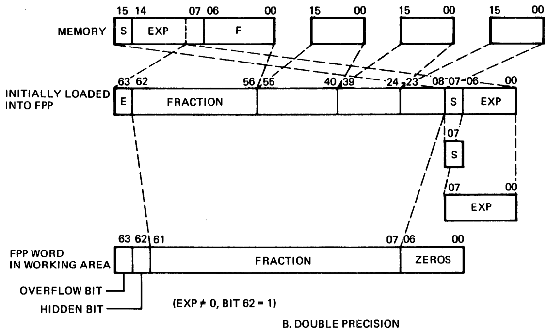
Figure 7-4 Floating-Point Data Words
