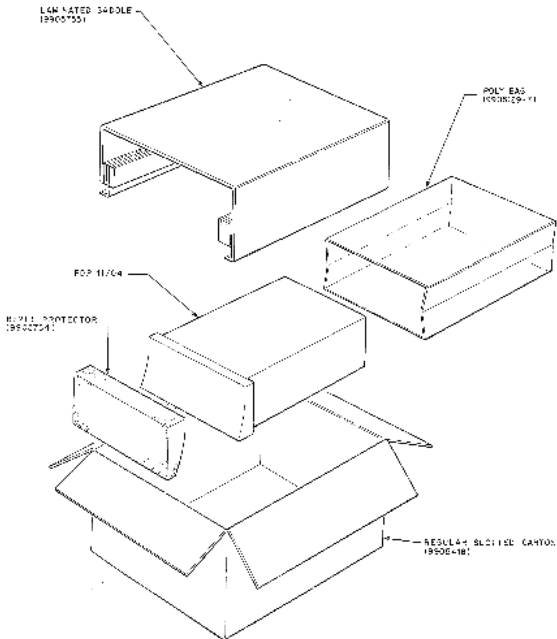
Figure S-4 Packaging of PDP-11/04 [13.3-cm (5-1/4-inch Box)]
