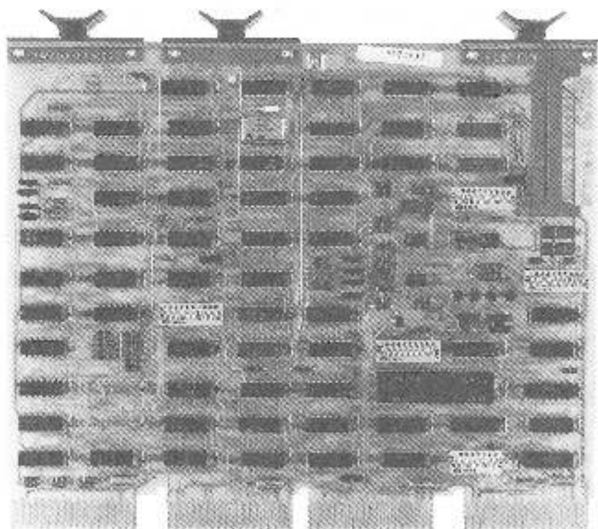
Figure 4-9 DL11-W (M7856) Switch Locations
