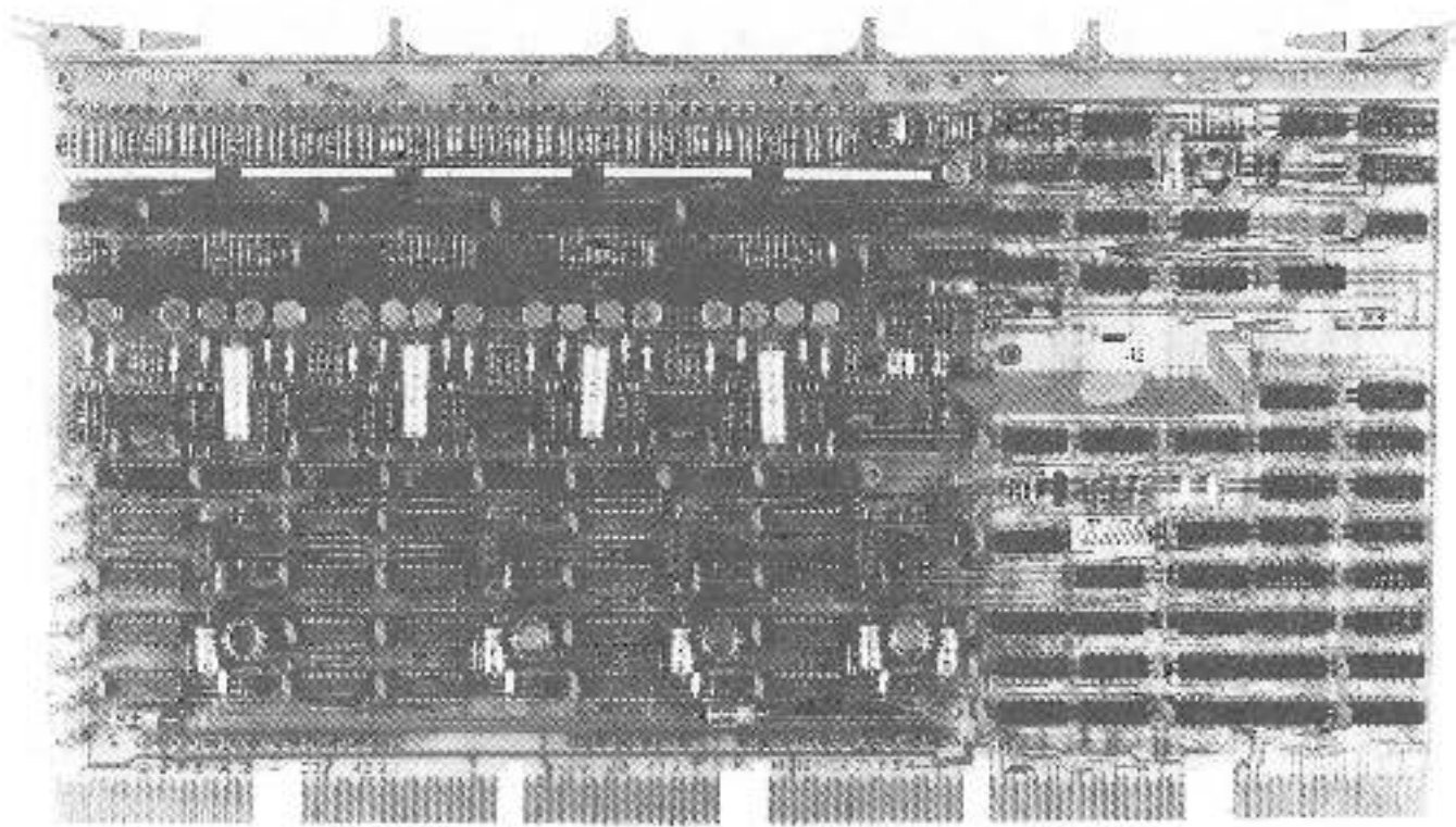
Figure 1-8 MM11-CP Core Memory Module
