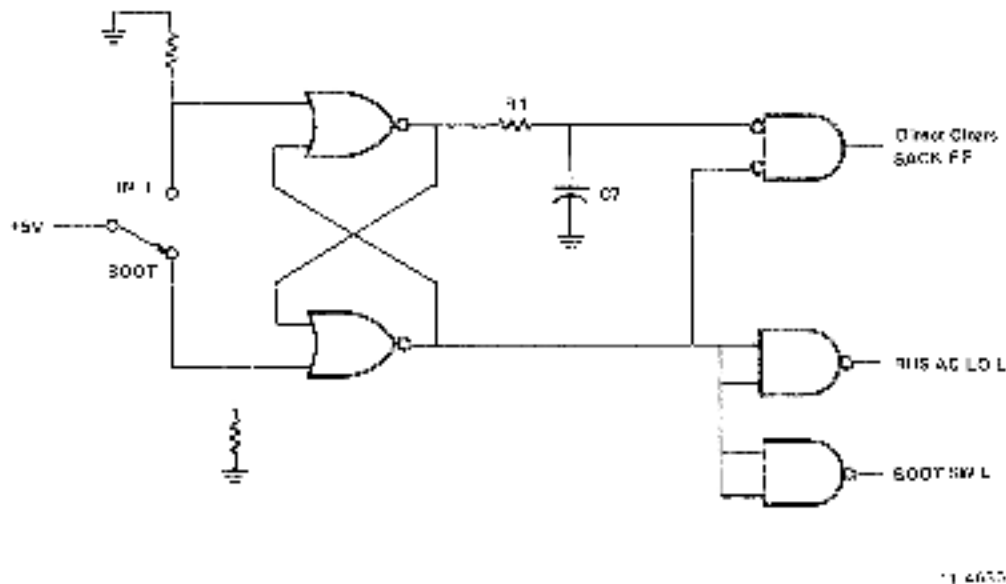
Figure 3-5 BOOT/INIT Switch Logic
