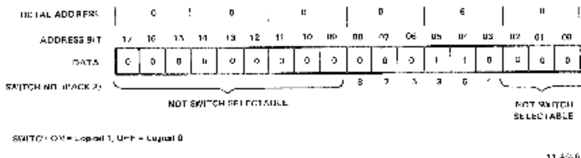
Figure 4-11 DL11-W Vector Address Selection
