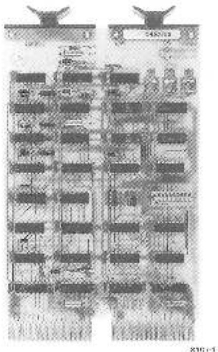
Figure 1-5 M9301 Bootstrap/Terminator Module
