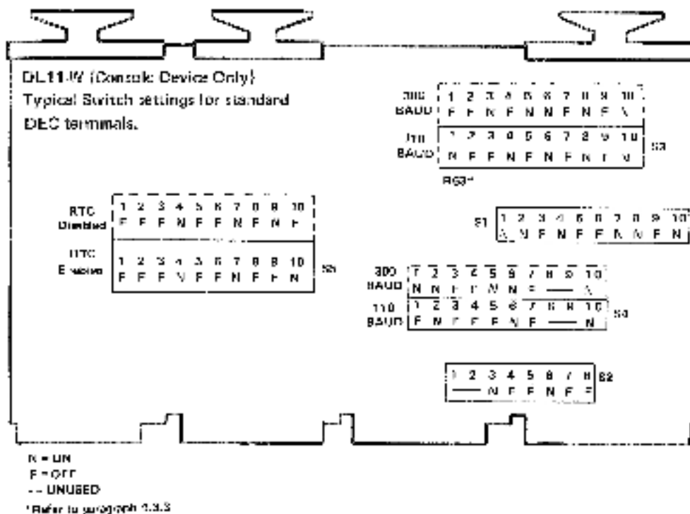
Figure 5-10 Typical Jumper Placement and Switch Settings of Modules (Sheet 3 of 7)
