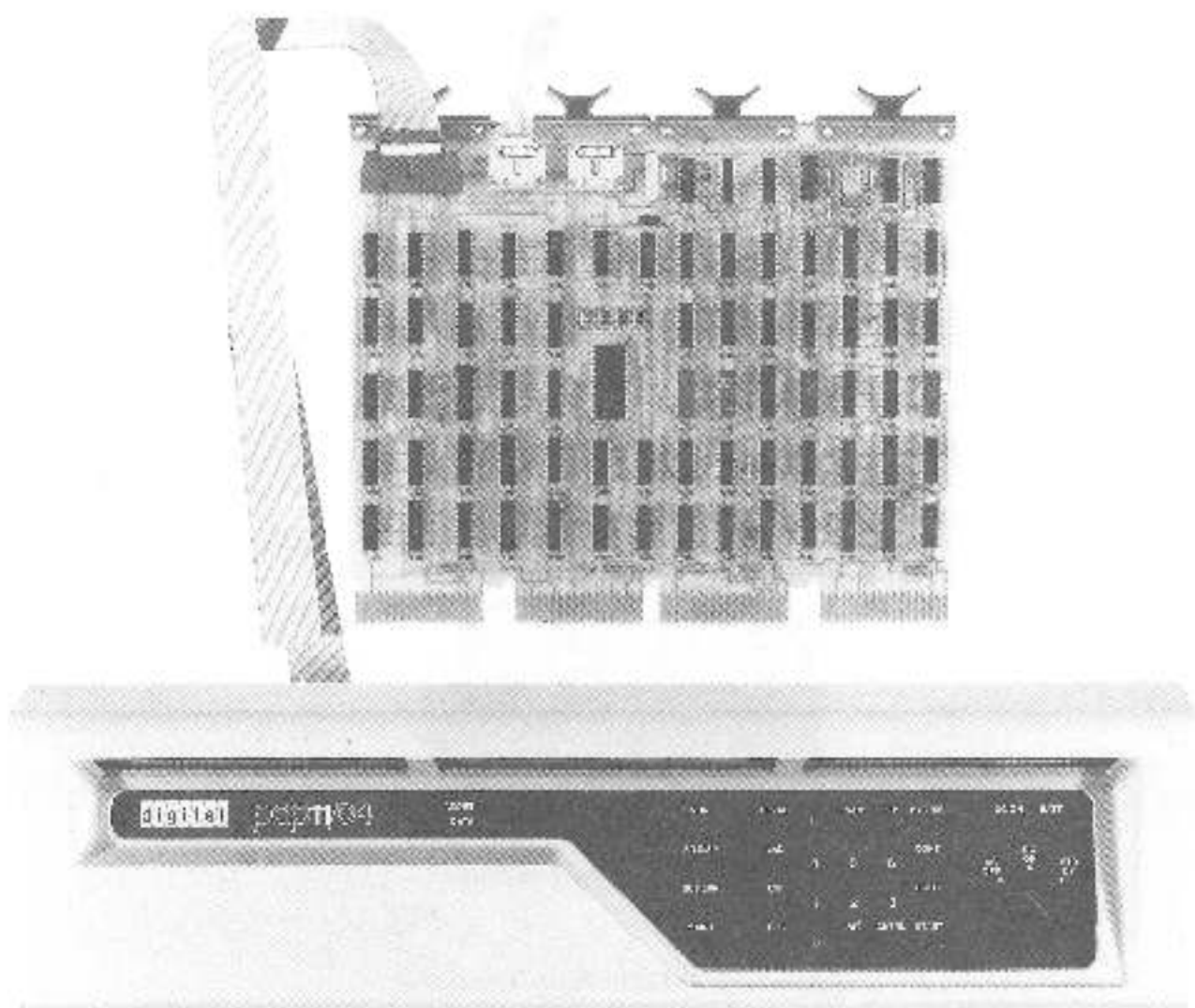
Figure 1-11 KY11-LB Console and Interface Module
