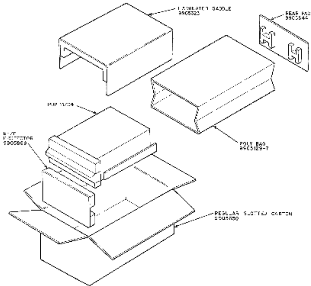
Figure S-3 Packaging of PDP-11/04 [26.3-cm (10-1/2-inch Box)]
