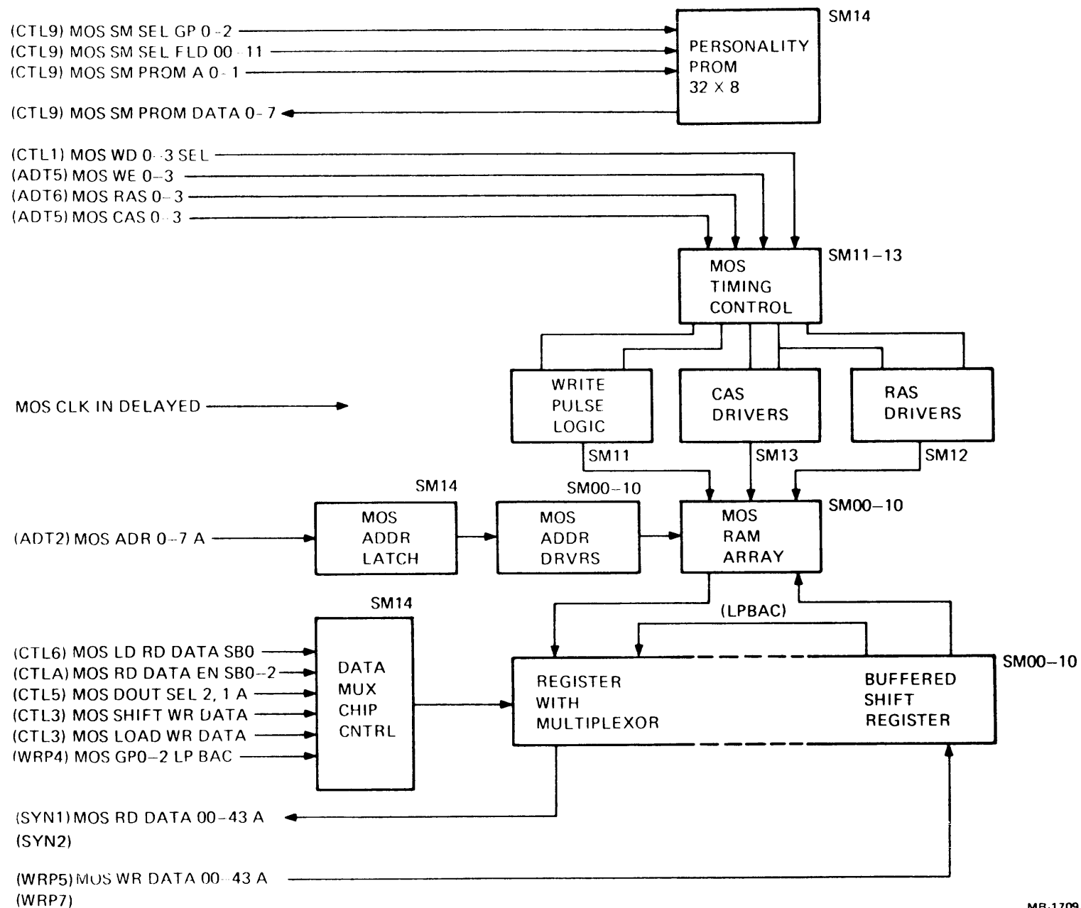
Figure 5-4 M8579 Functional Block Diagram
