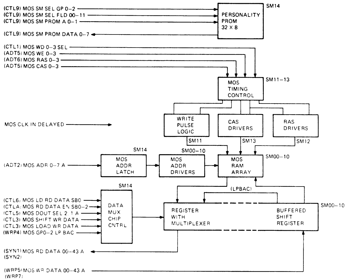
Figure 9-5 M8570 Functional Block Diagram
