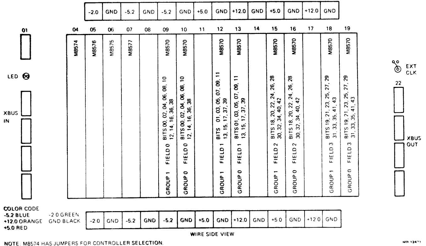
Figure 9-3 MG20 Simplified Module Utilization List
