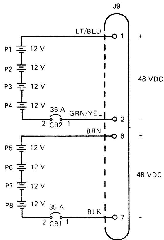
(A) SCHEMATIC
