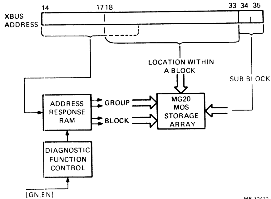
Figure 9-4 Memory Module Access
