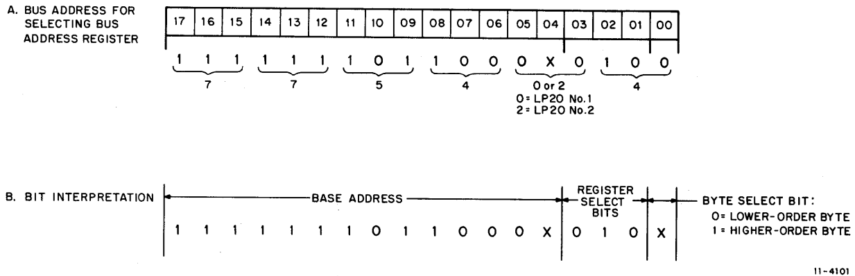
Figure 5-5 Bit Configuration for Bus Address Register
