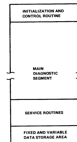
Figure 5 Internal Structure of Diagnostic Programs
