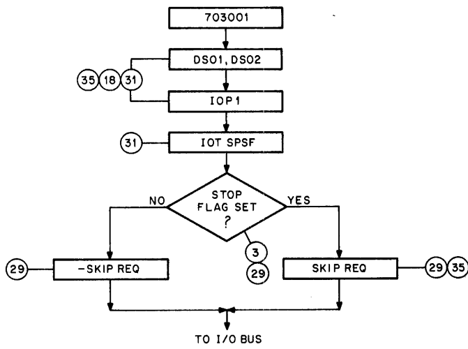
Figure 4-7 Skip On Stop Flag (SPSF) Flow Diagram
