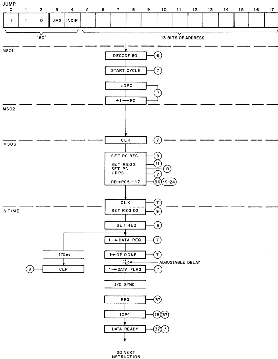
Figure 4-33 Jump Instruction Flow Diagram
