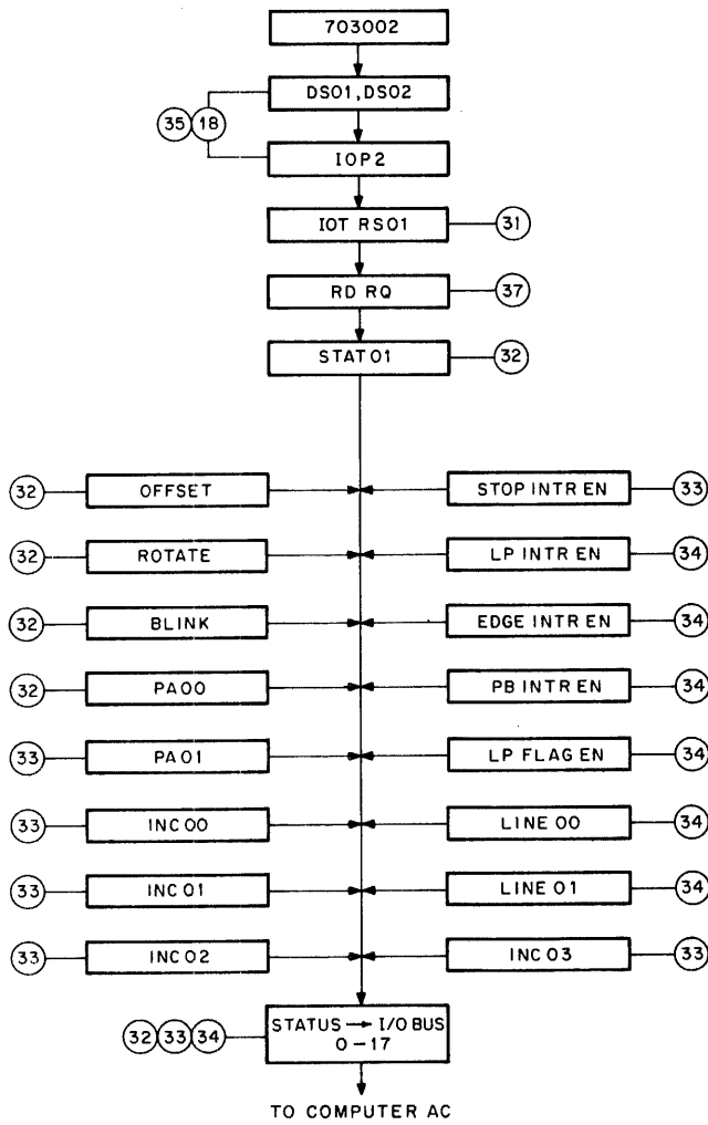
Figure 4-14 Read Status 1 (RS1) Flow Diagram
