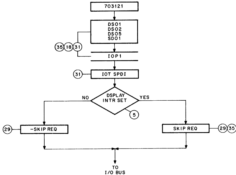
Figure 4-12 Skip On Any Interrupt Flag (SPDI) Flow Diagram
