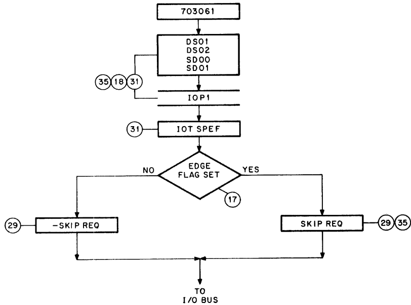
Figure 4-10 Skip On Edge Flag (SPEF) Flow Diagram
