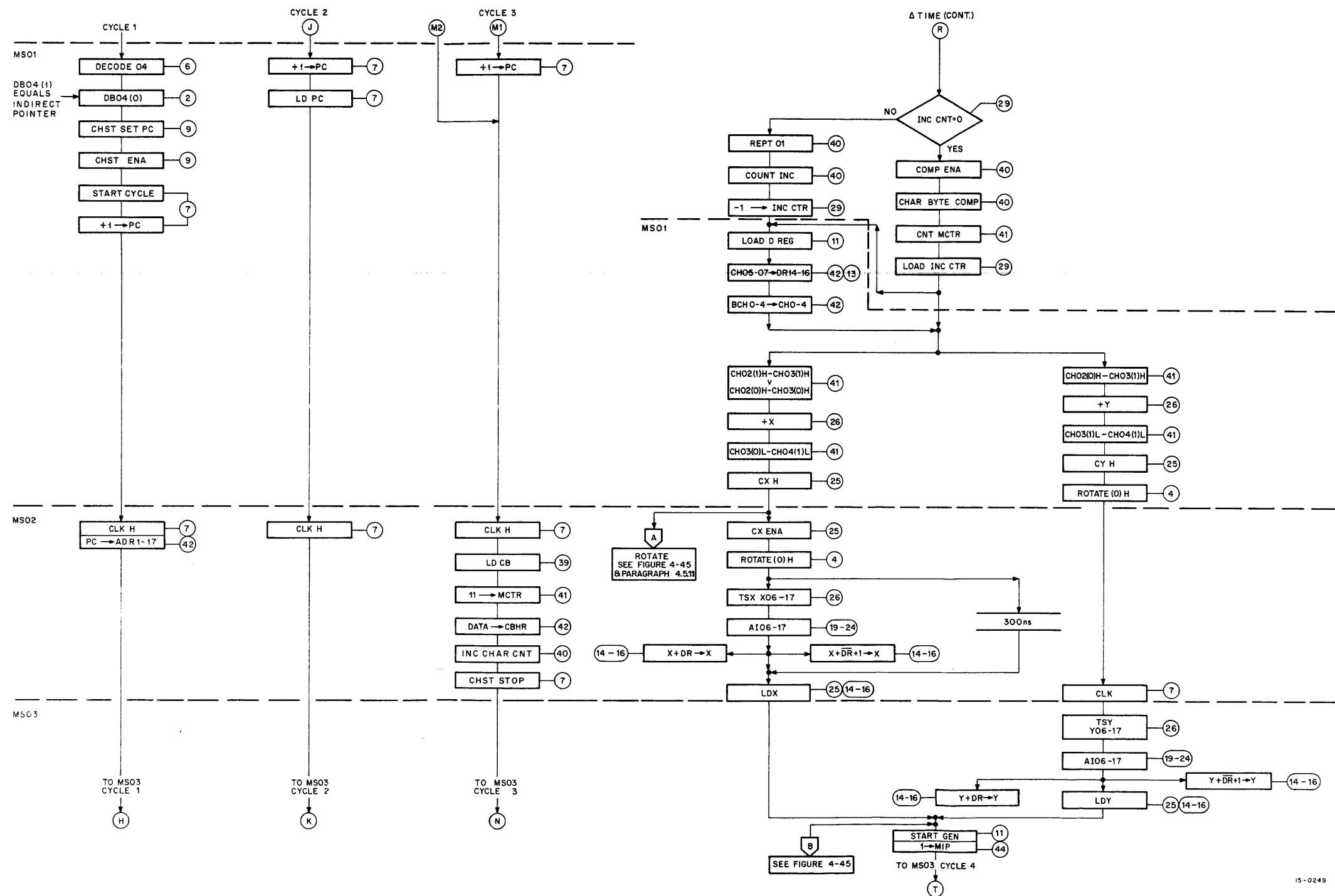
Figure 4-41 Character String Instruction Flow Diagram (Sheet 1 of 3)
