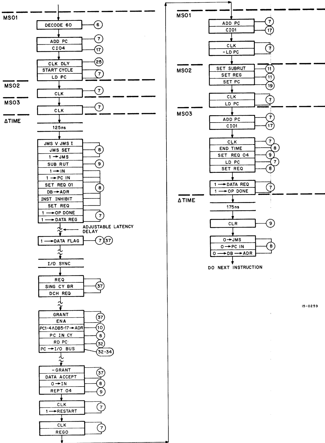
Figure 4-35 DJMS Instruction Flow Diagram
