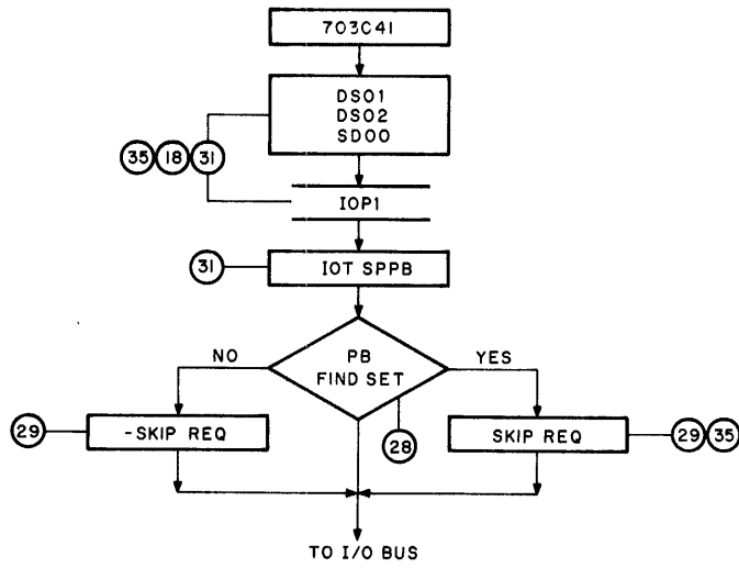
Figure 4-9 Skip On Pushbutton Flag (SPPB) Flow Diagram
