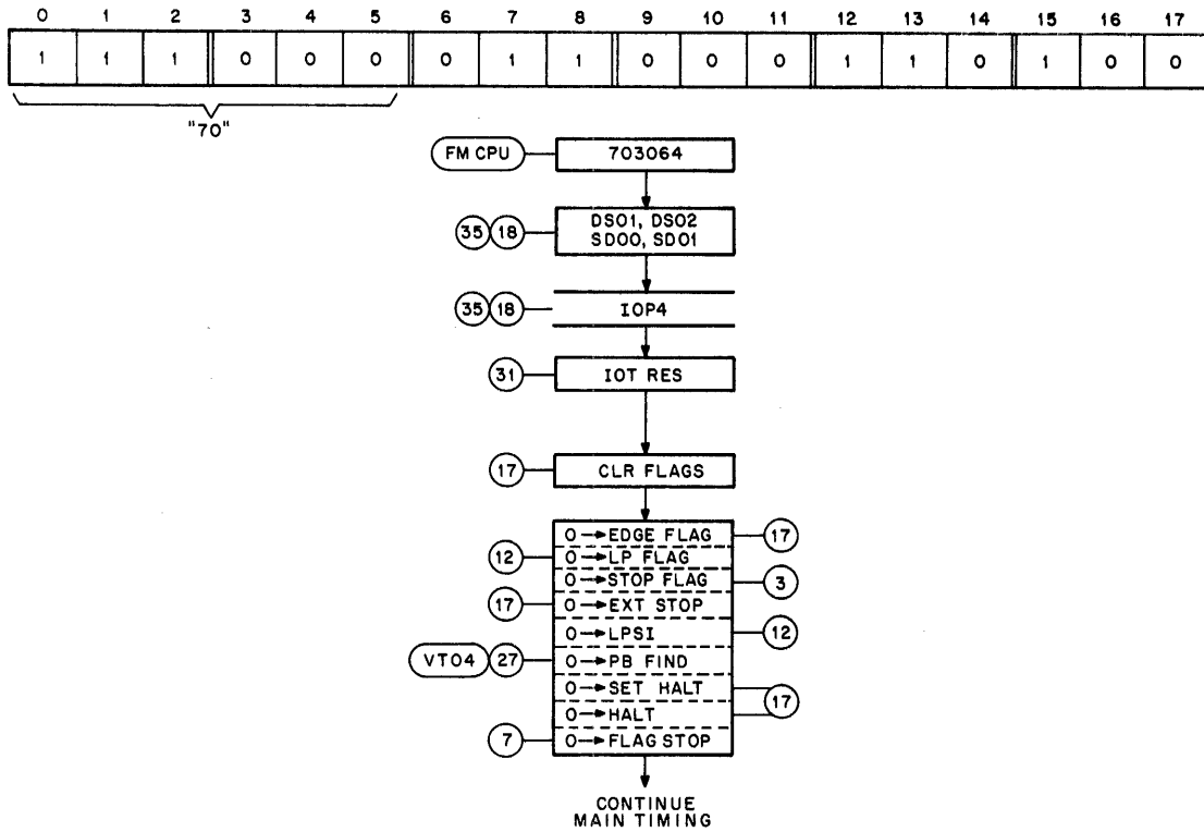
Figure 4-5 Resume Display After Flag (RES) Flow Diagram
