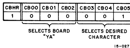
Figure 5-2 Character "YA" Board and Character Selection
