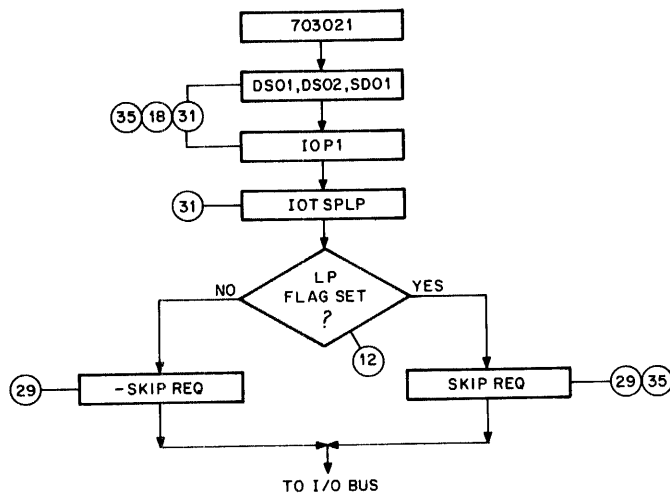
Figure 4-8 Skip On Light Pen Flag (SPLP) Flow Diagram
