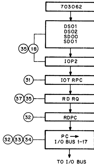
Figure 4-17 Read Program Counter (RPC) Register Flow Diagram
