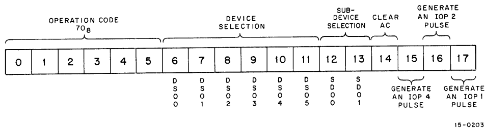
Figure 4-1 Basic IOT Command Format
