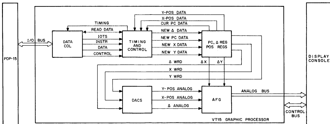
Figure 3-1 Major Functional Groups, Interconnect Diagram
