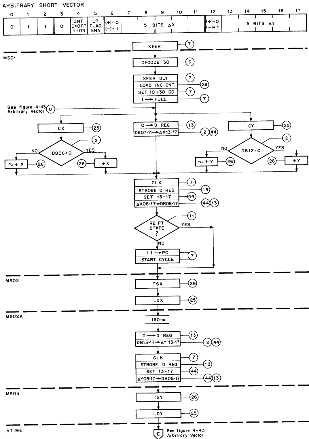
Figure 4-44 Arbitrary Short Vector Flow Diagram
