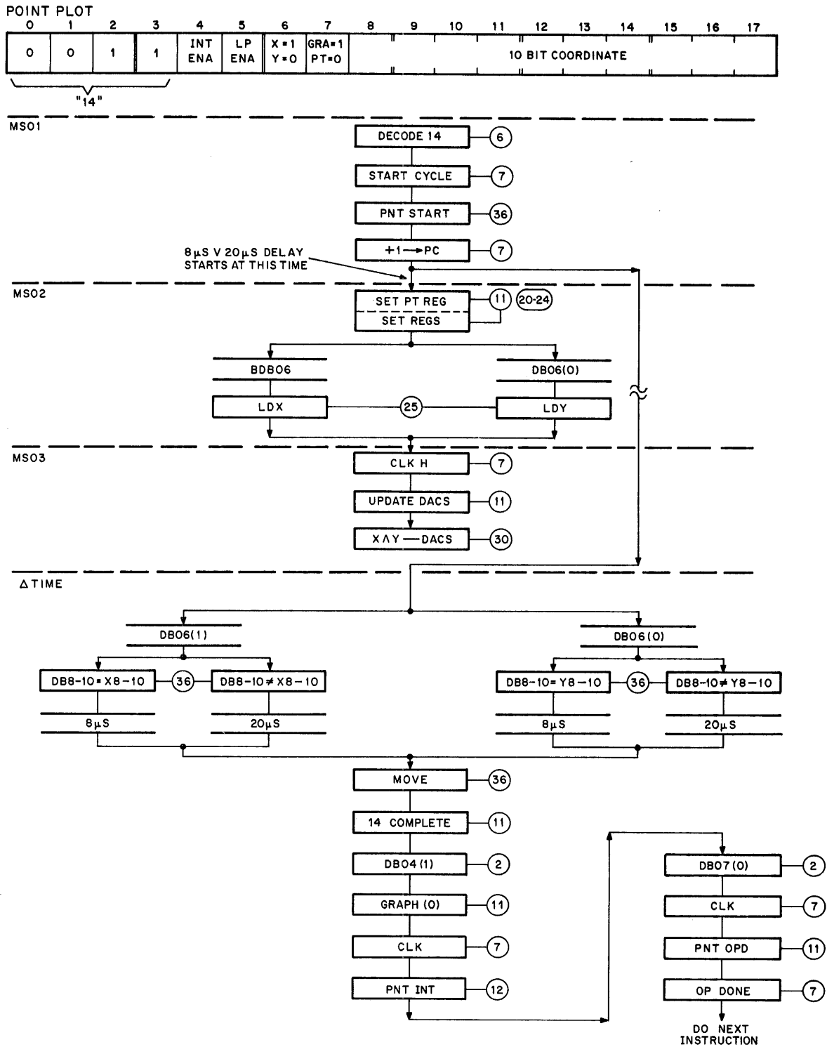
Figure 4-31 Point Plot Instruction Flow Diagram
