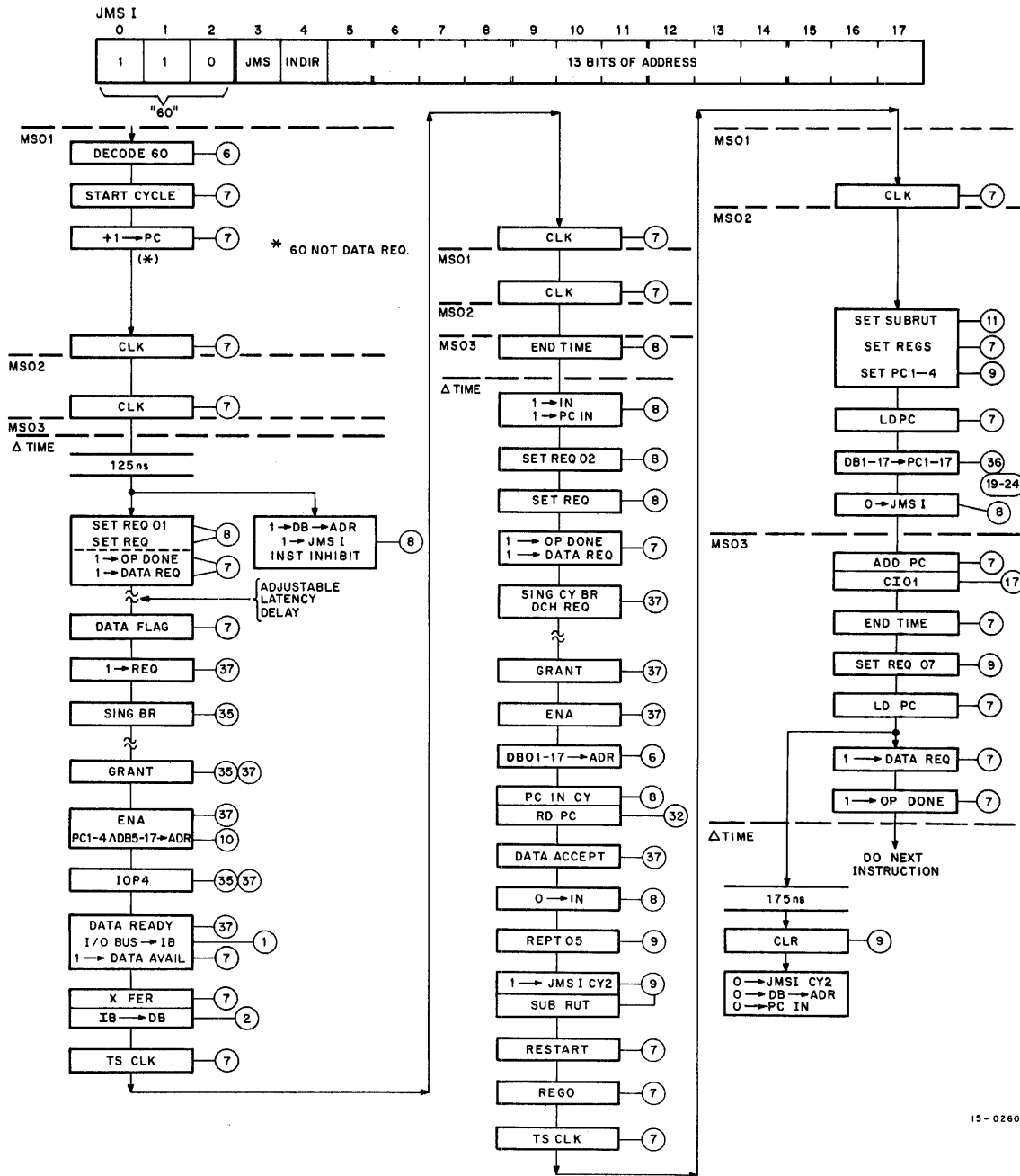
Figure 4-36 JMS Indirect Instruction Flow Diagram
