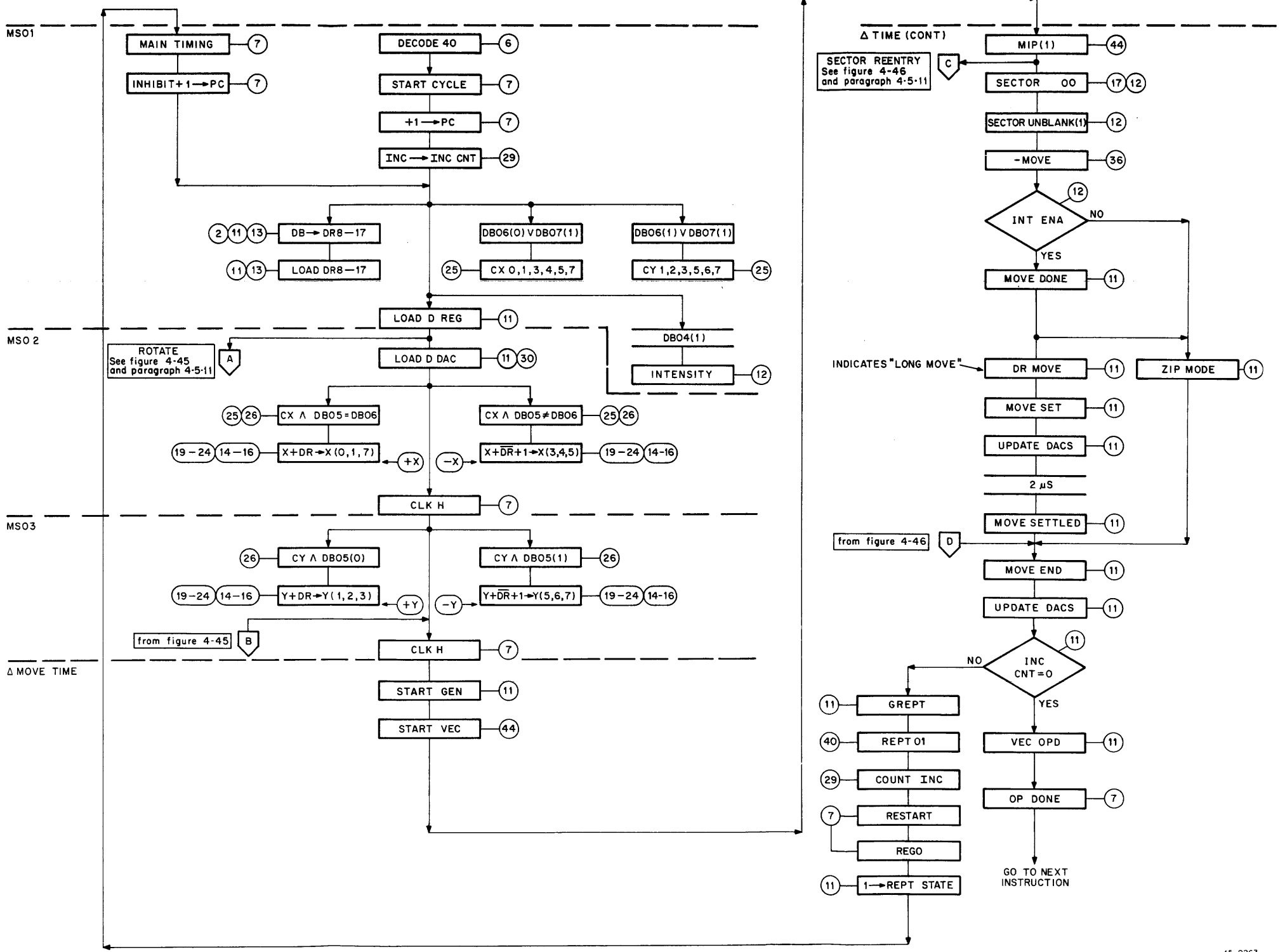
Figure 4-28 Basic Vector Instruction Flow Diagram
