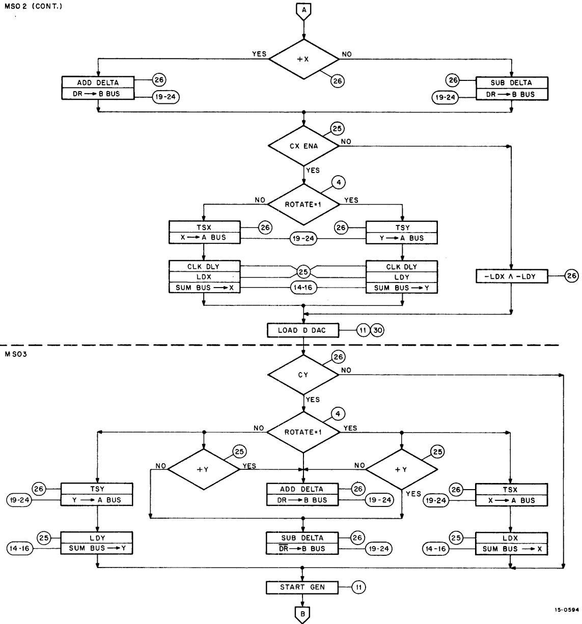
Figure 4-46 Rotate Flow Diagram
