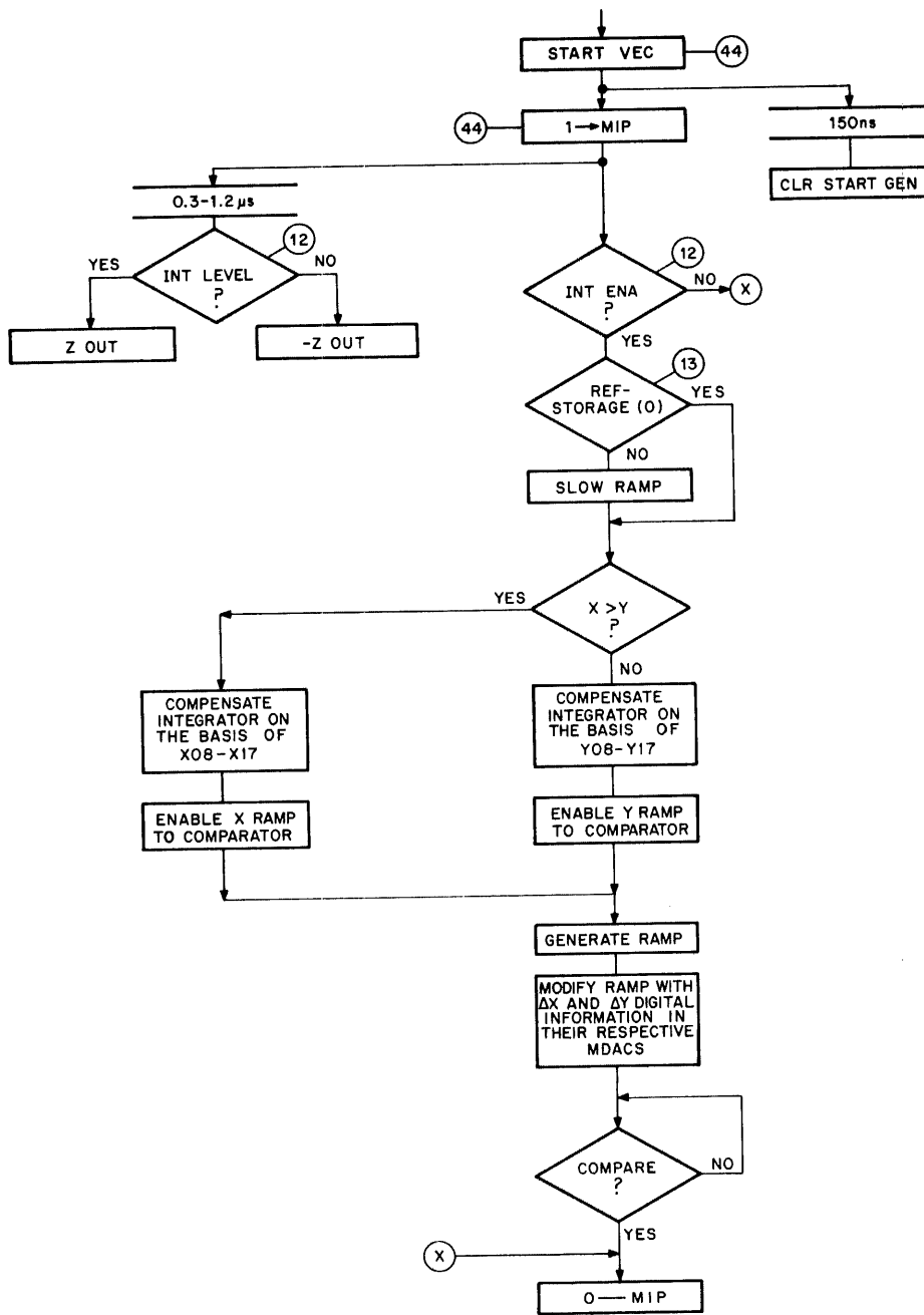
Figure 4-43a Arbitrary Vector Functional Flow Diagram
