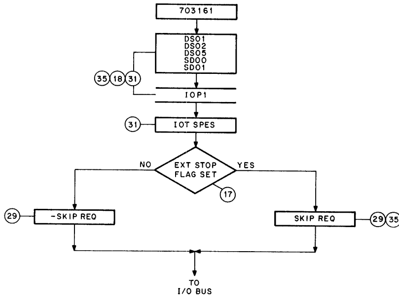
Figure 4-13 Skip On External Stop (SPES) Flow Diagram
