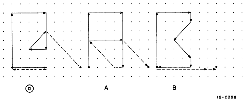
Figure 4-39 ASCII Character Generation
