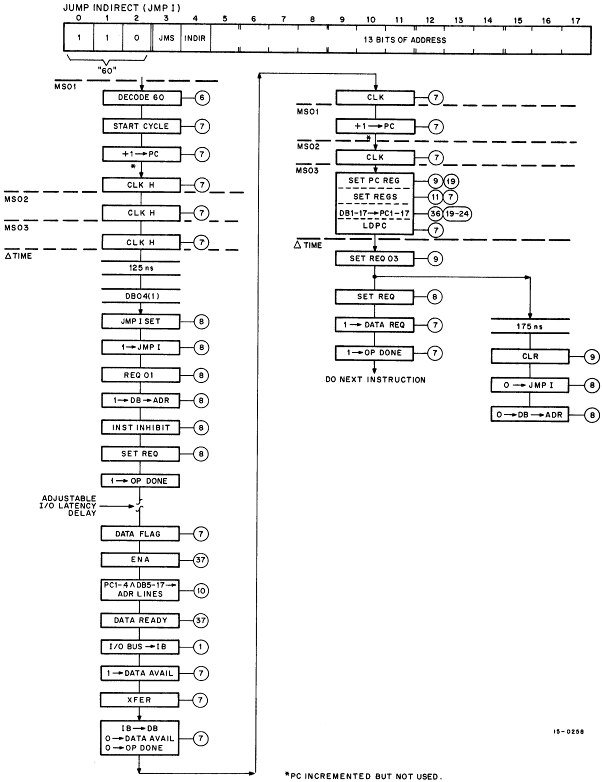
Figure 4-34 Jump Indirect Instruction Flow Diagram
