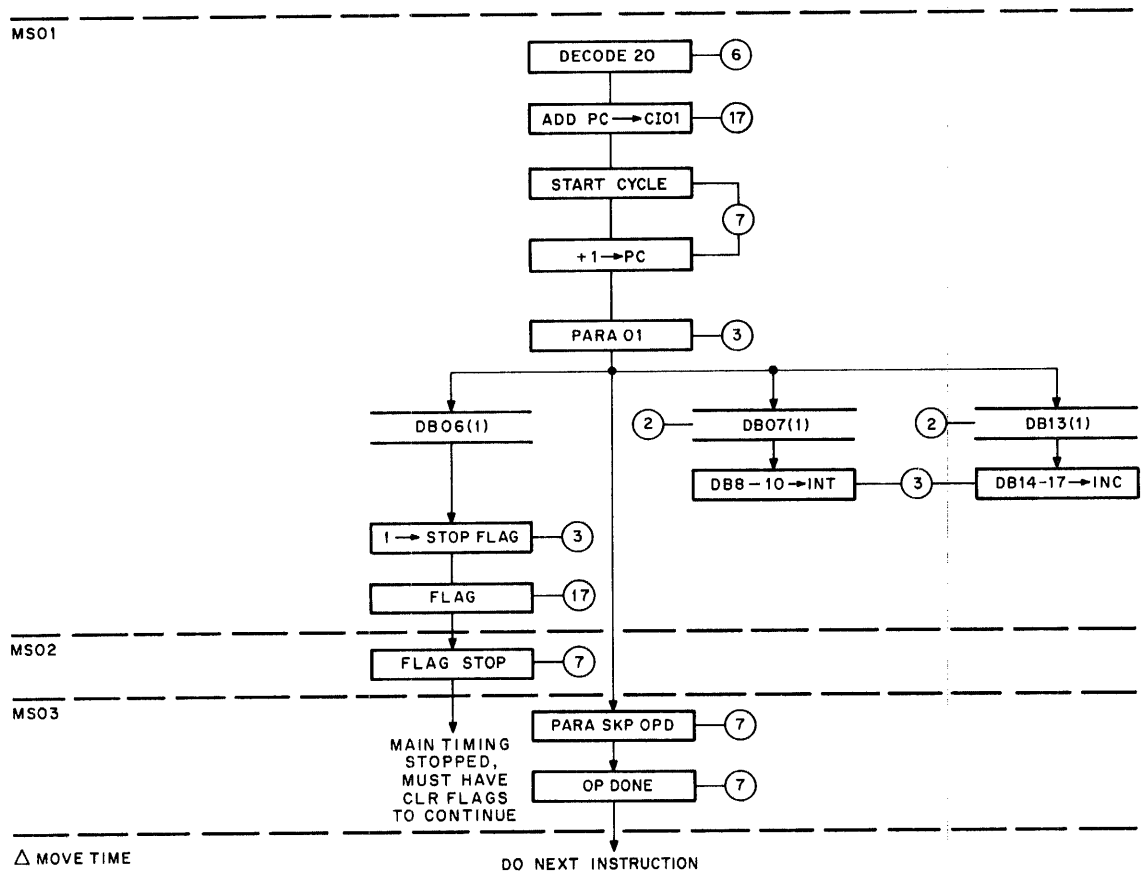
Figure 4-20 Parameter 1 Instruction Flow Diagram
