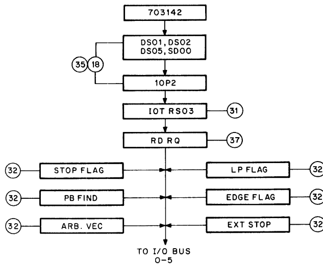
Figure 4-16 Read Status 3 (RS3) Flow Diagram
