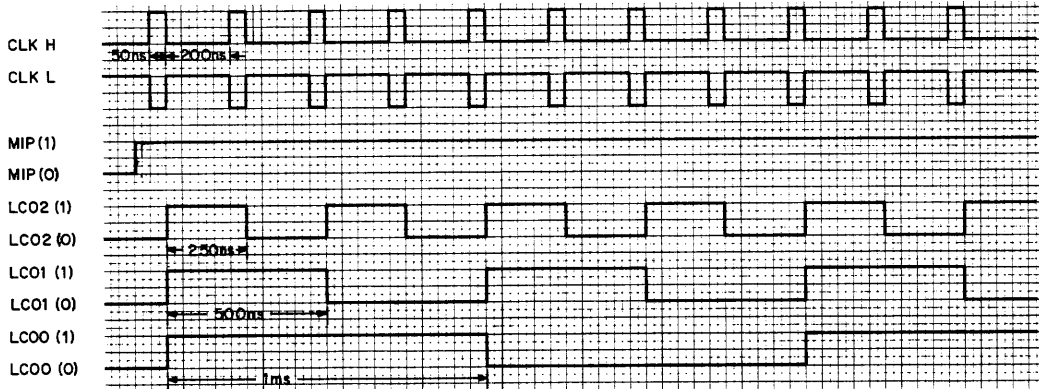
Figure 4-24 Line Function Timing
