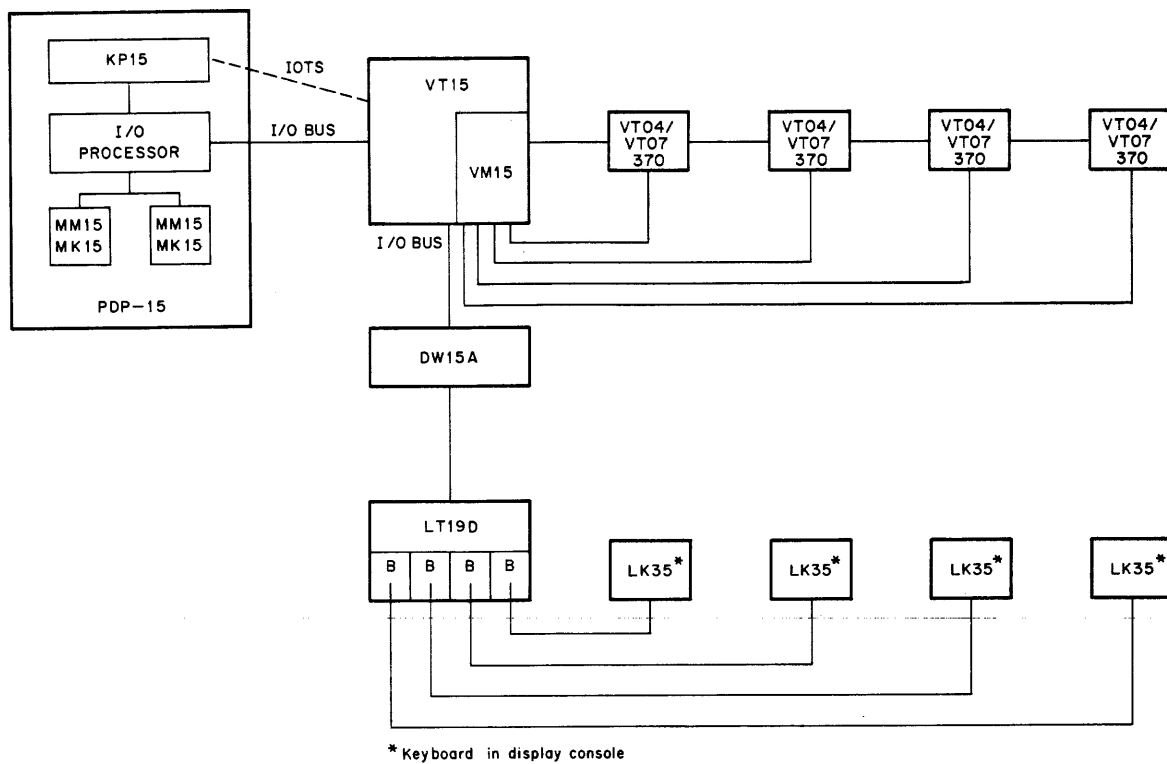
Figure 1-2 Graphic-15 Display System Interconnect Diagram
