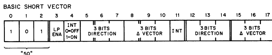
Figure 4-29 Basic Short Vector Instruction Format
