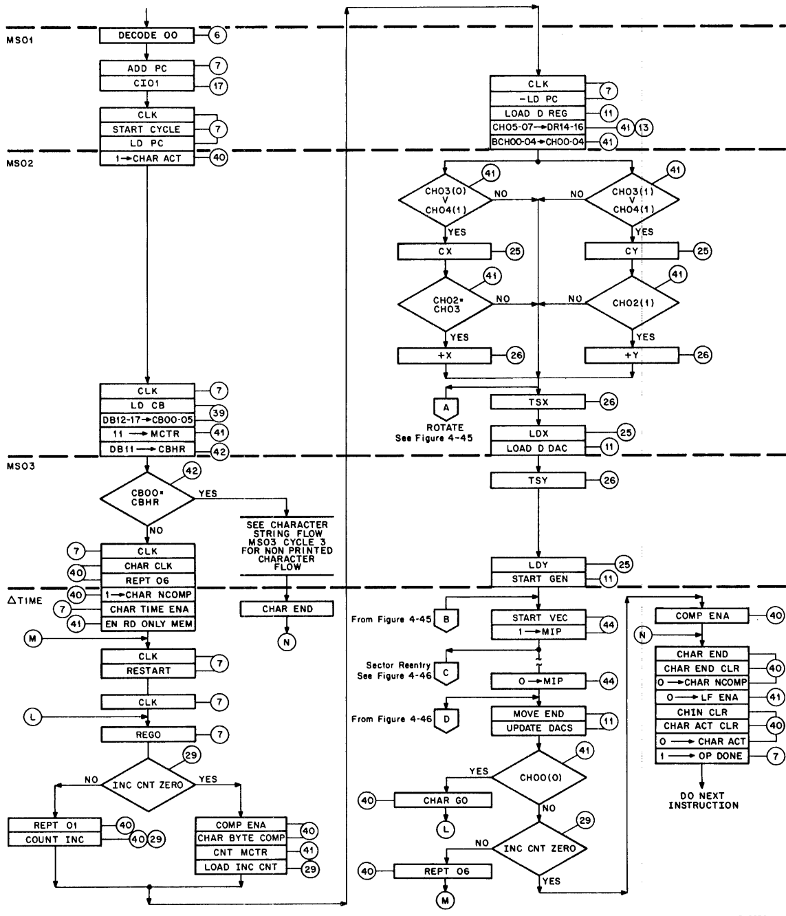
Figure 4-38 Character Input Instruction Flow Diagram
