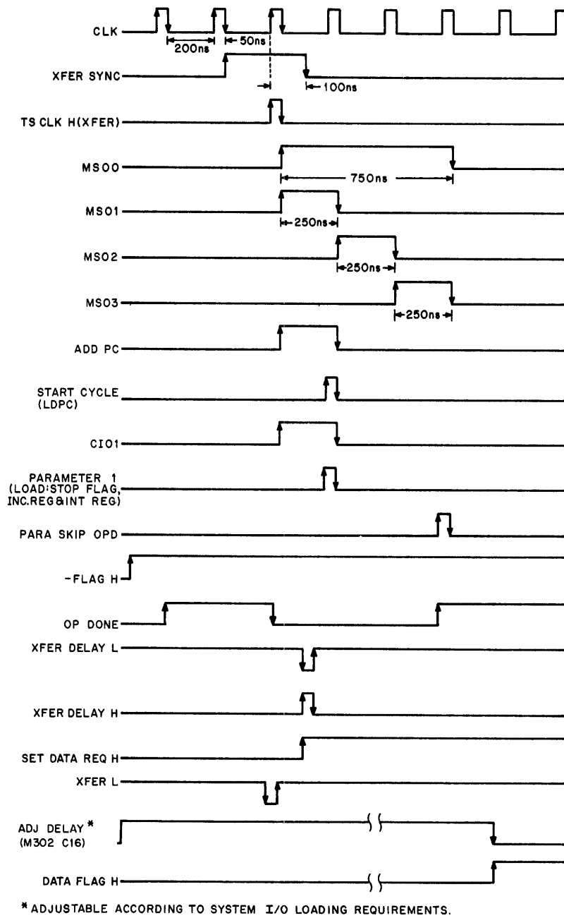
Figure 4-21 Instruction Basic Timing Diagram
