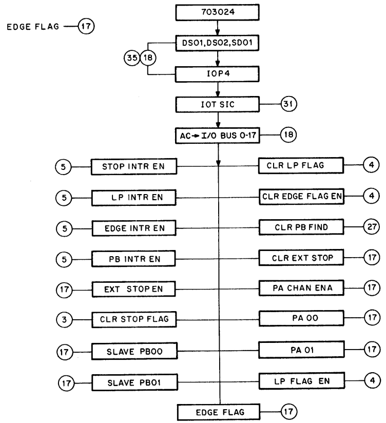
Figure 4-2 Set Initial Conditions (SIC) Flow Diagram
