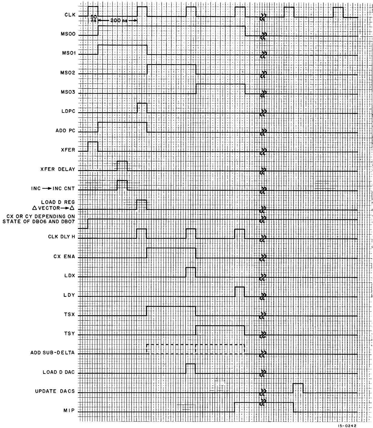
Figure 3-4 VT15 Main Timing Diagram (Sheet 1 of 2)
