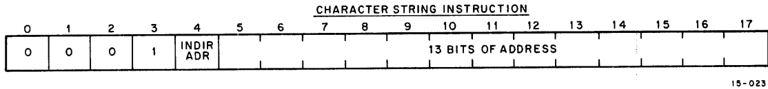
Figure 4-40 Character String Instruction Format
