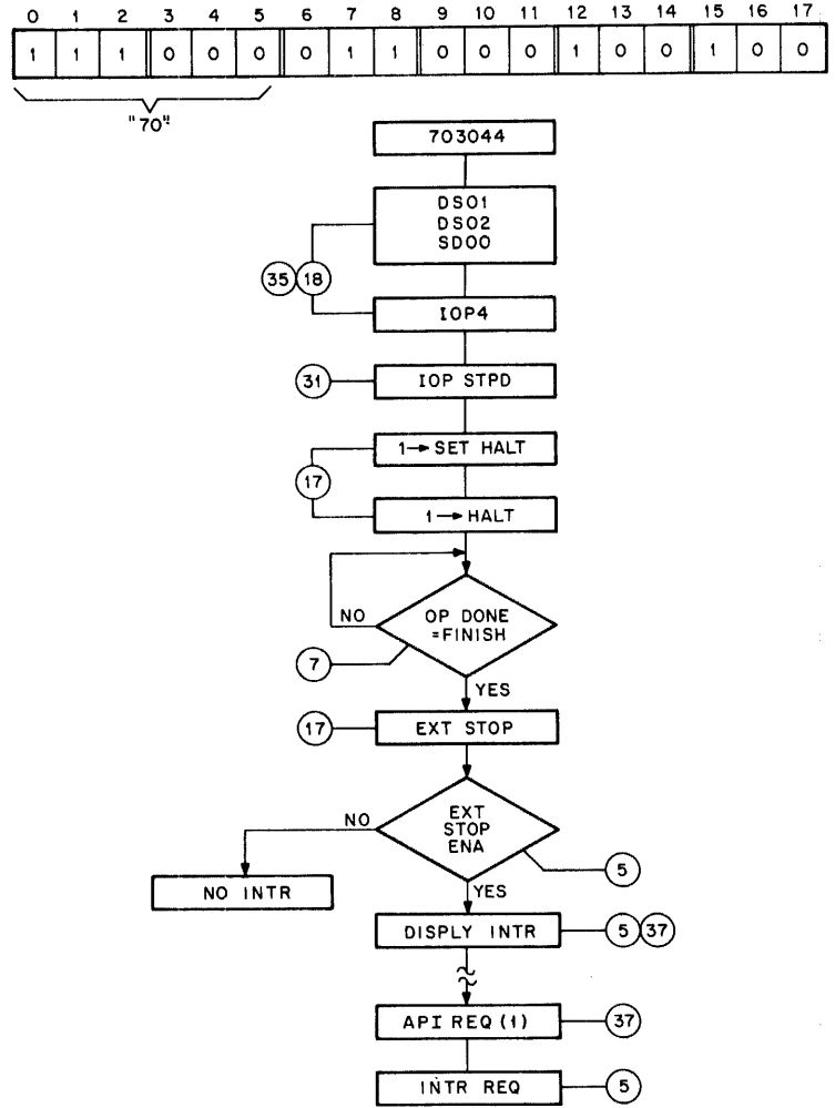
Figure 4-4 External Stop Display (STPD) Flow Diagram
