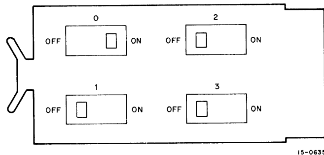
Figure 2-3 W719 Unit Select Module
