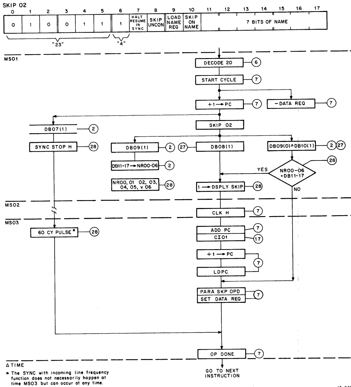
Figure 4-26 Skip 2 Instruction Flow Diagram
