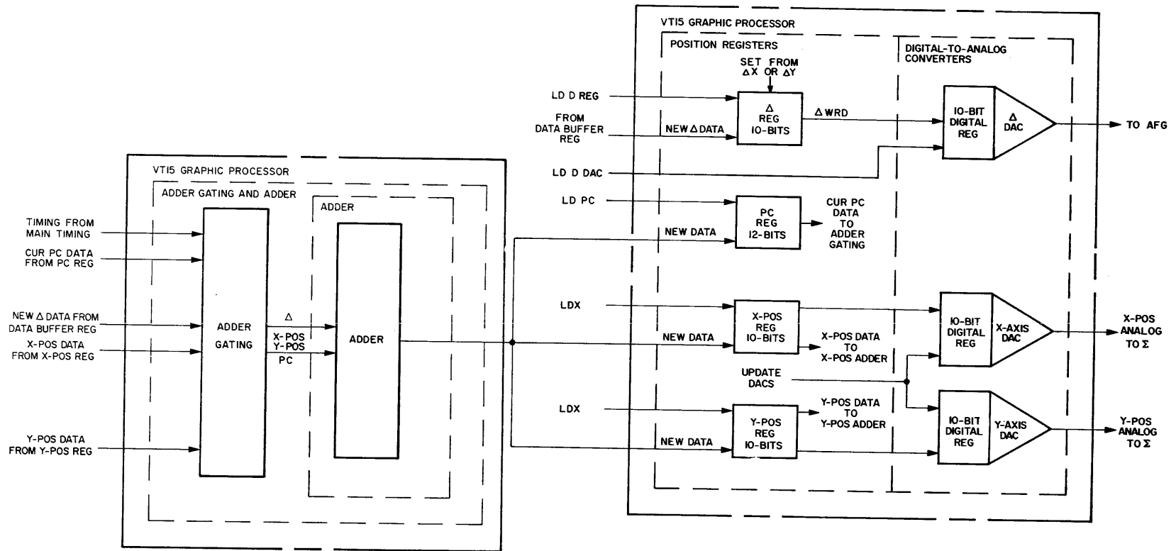
Figure 3-2 VT15 Major Functional Groups, Functional Block Diagram (Sheet 2 of 2)
