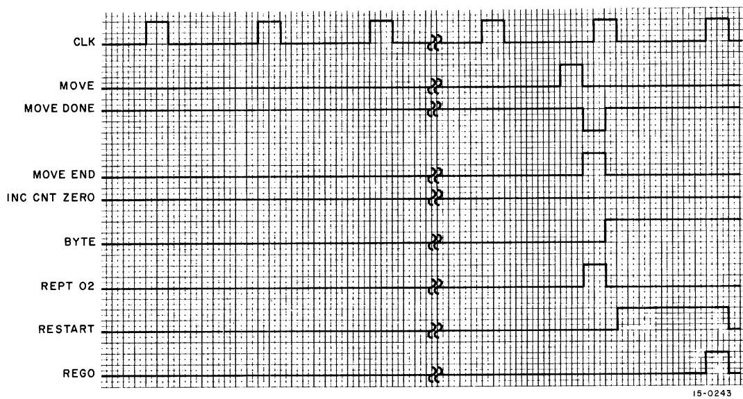
Figure 3-4 VT15 Main Timing Diagram (Sheet 2 of 2)
