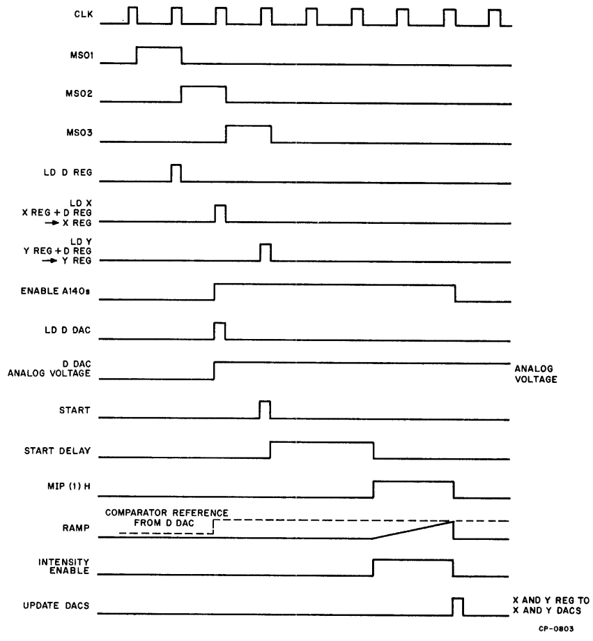
Figure 3-6 Analog Function Timing Diagram (Basic Vector)
