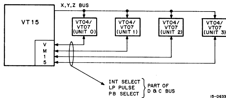
Figure 2-2 VM15 Interconnect Diagram
