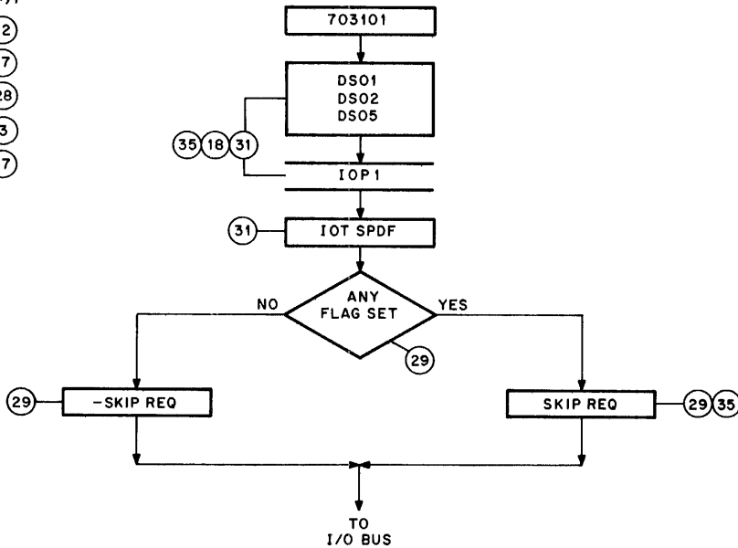
Figure 4-11 Skip On Any Flag (SPDF) Flow Diagram
