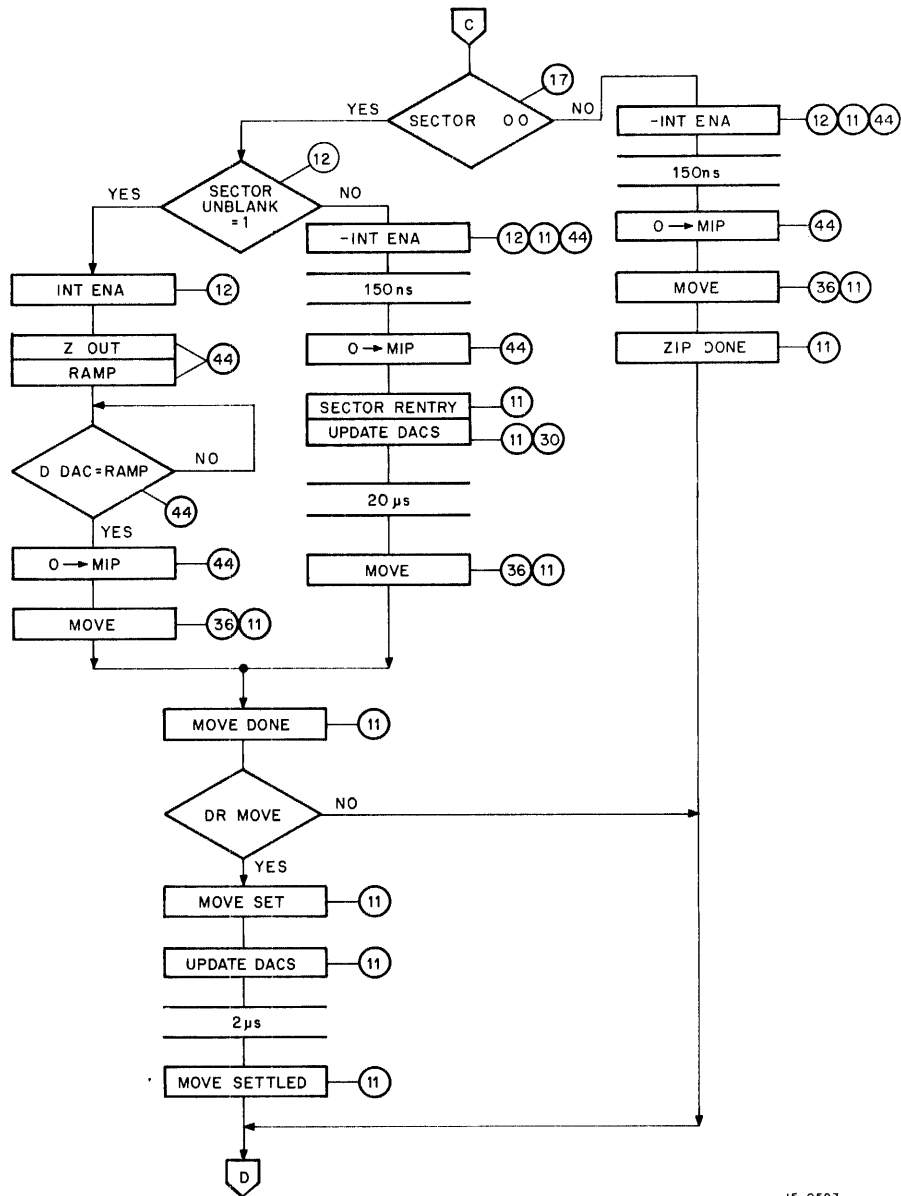
Figure 4-47 Sector Re-Entry Flow Diagram
