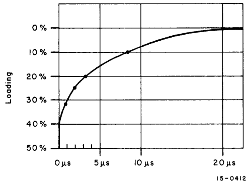
Figure 6-1 I/O Loading Delay Characteristics
