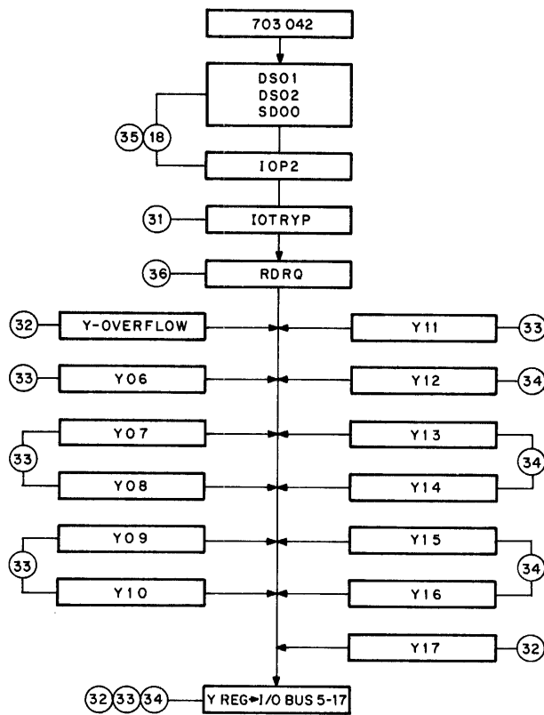
Figure 4-19 Read Y-Position Register (RYP) Flow Diagram
