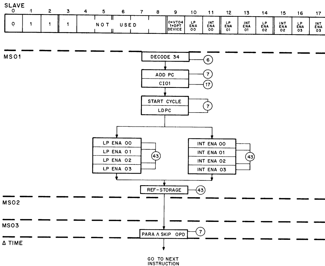
Figure 4-45 Slave Instruction Flow Diagram
