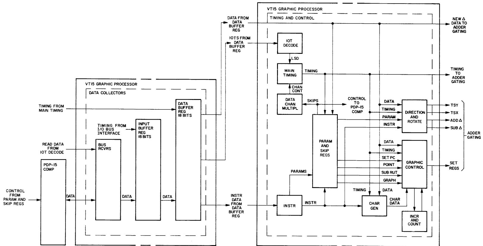
Figure 3-2 VT15 Major Functional Groups, Functional Block Diagram (Sheet 1 of 2)
