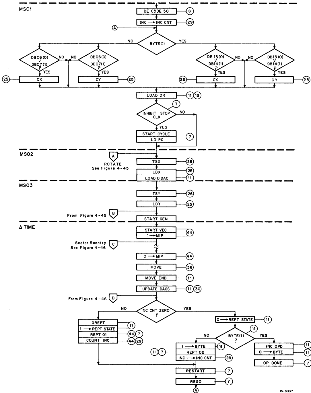
Figure 4-30 Basic Short Vector Instruction Flow Diagram
