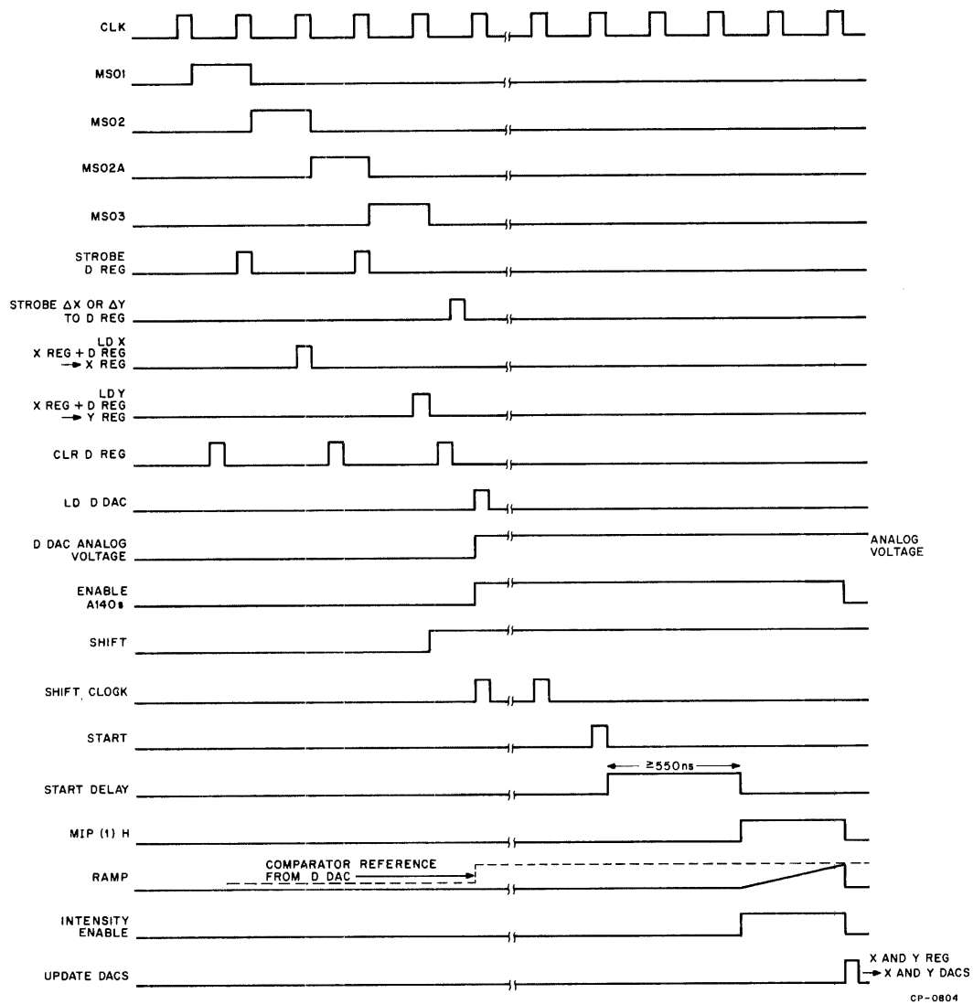
Figure 3-7 Analog Function Timing Diagram (Arbitrary Vector)
