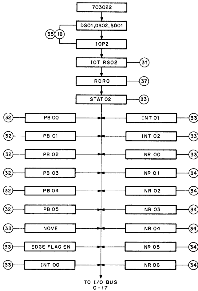
Figure 4-15 Read Status 2 (RS2) Flow Diagram
