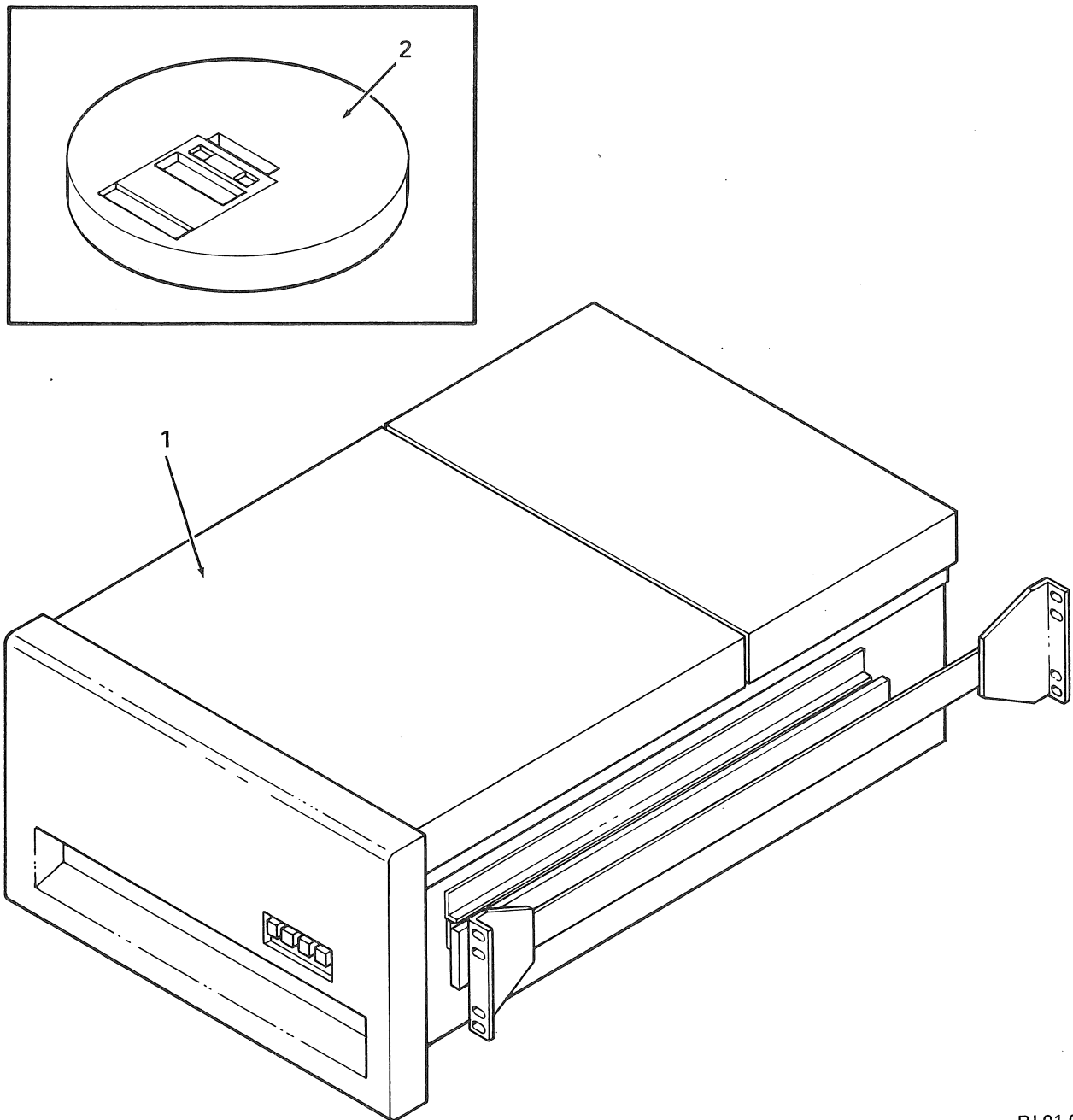
Figure 1. RL01 Disk Drive and Cartridge
