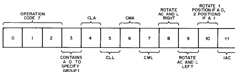
Figure 3-3 Group 1 Operate Microinstruction Format
