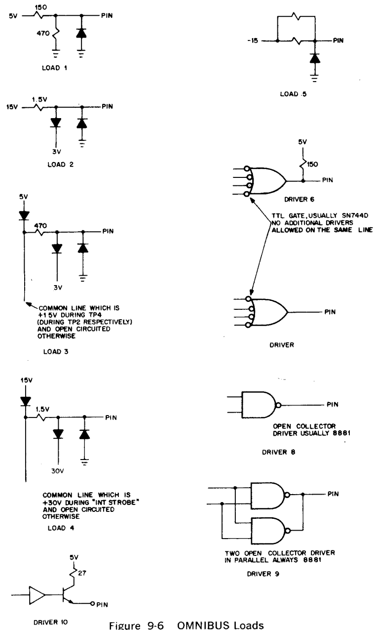
Figure 9-6 OMNIBUS Loads
