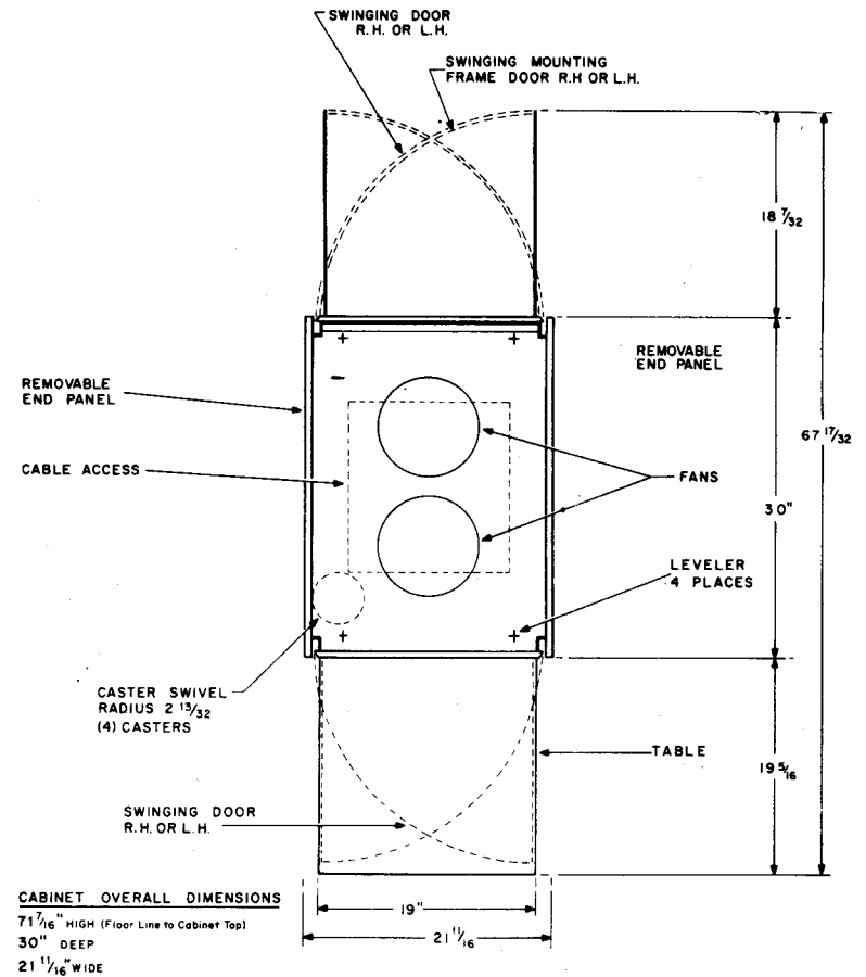
Figure 11-6 Cabinet Layout Dimensions
