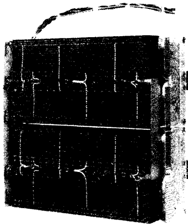
H9190 Mounting Panel —contains M Series connector blocks with 8/E type packaging for standard M Series modules. Also included are the 8/E power wiring harness and power bus board. There is M Series power bussing for all but the four slots in the first column. Four mounting spacers allow the H9190 to be easily mounted in the second half of an 8/E chassis.
