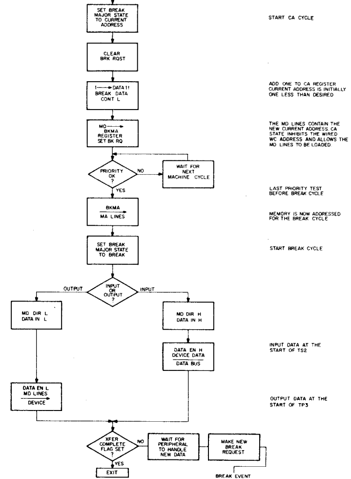
Figure 9-18 3-Cycle Data Break Implementation Flow Diagram (continued)
