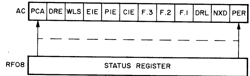
Figure 7-13 DISK TO AC STATUS REGISTER
