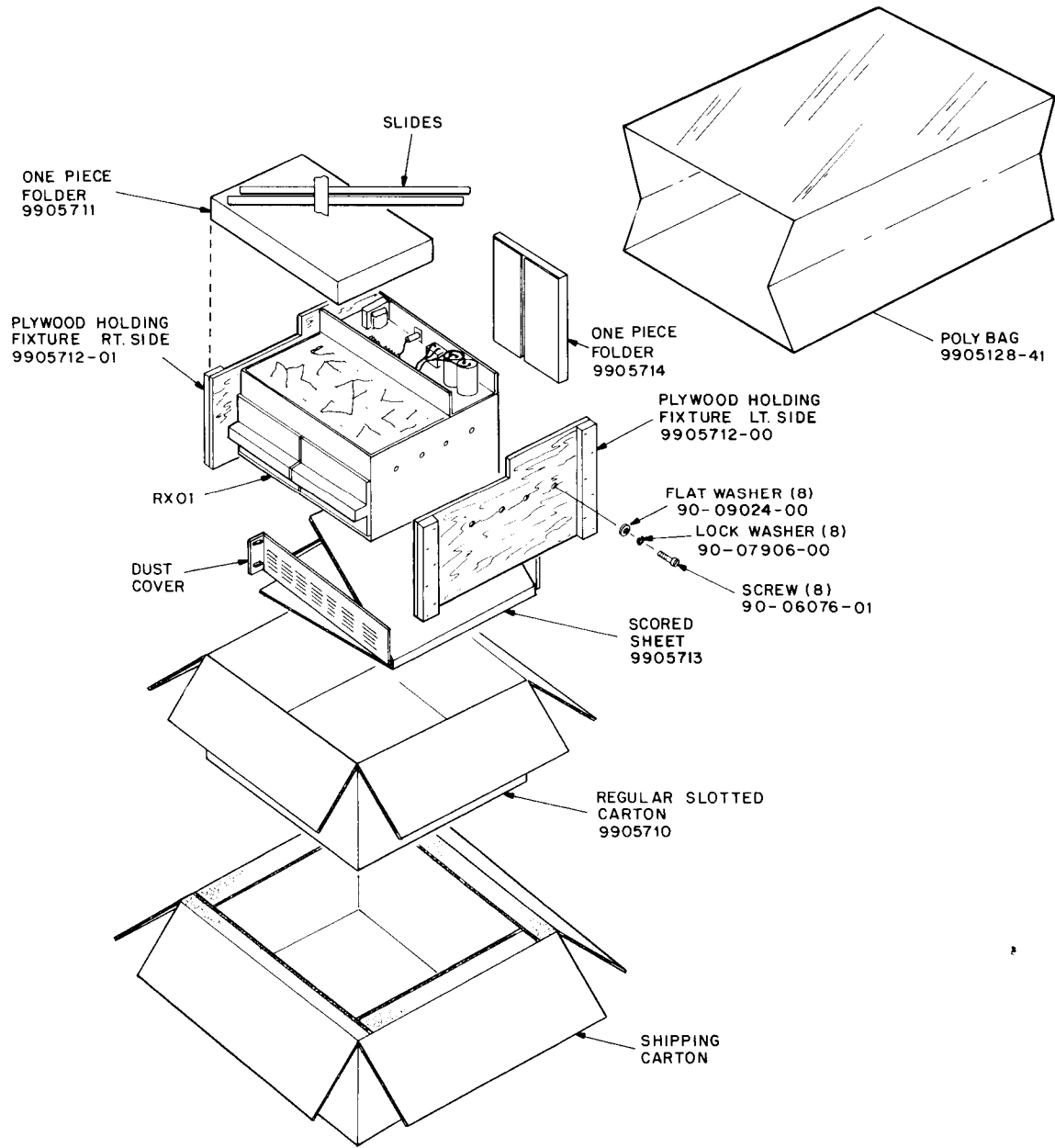
Figure 2-4 RX8/RX11 Unpacking
