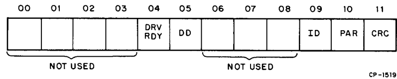
Figure 4-7 RXES Format (RX8E)
