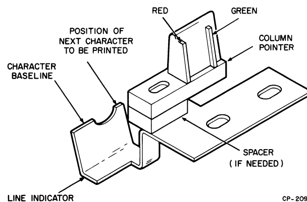
Figure 28 Line Indicator and Column Pointer
