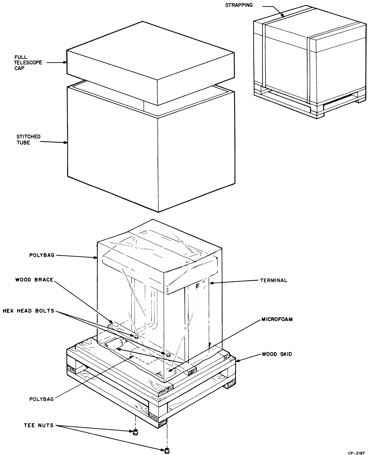
Figure 50 DECwriter Packaging
