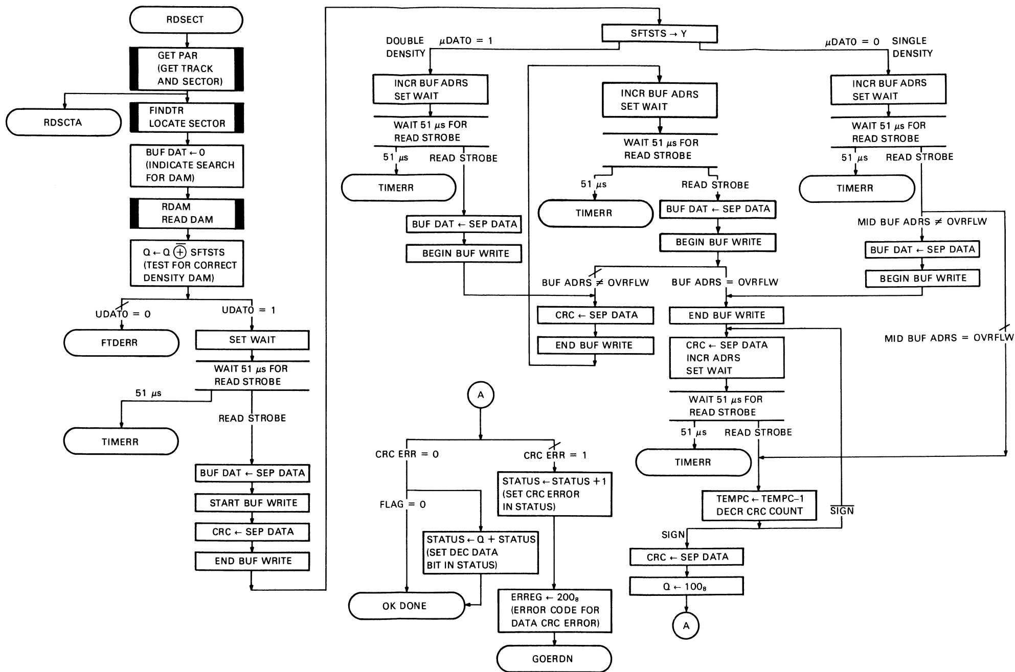
Figure 5-21 Read Sector Subroutine Flowchart
