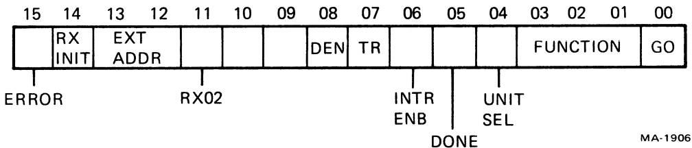
Figure 4-25 RX2CS Format (RX211/RXV21)
