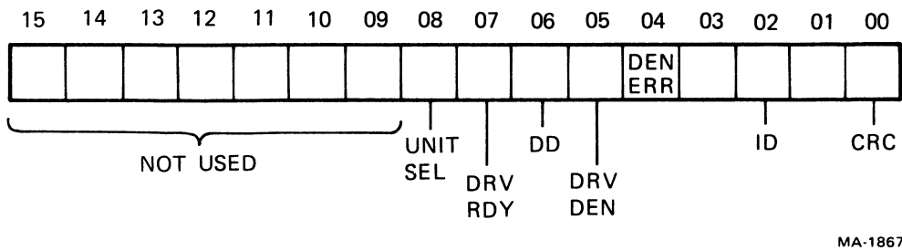
Figure 4-21 RXES Format (RX11, RXV11)
