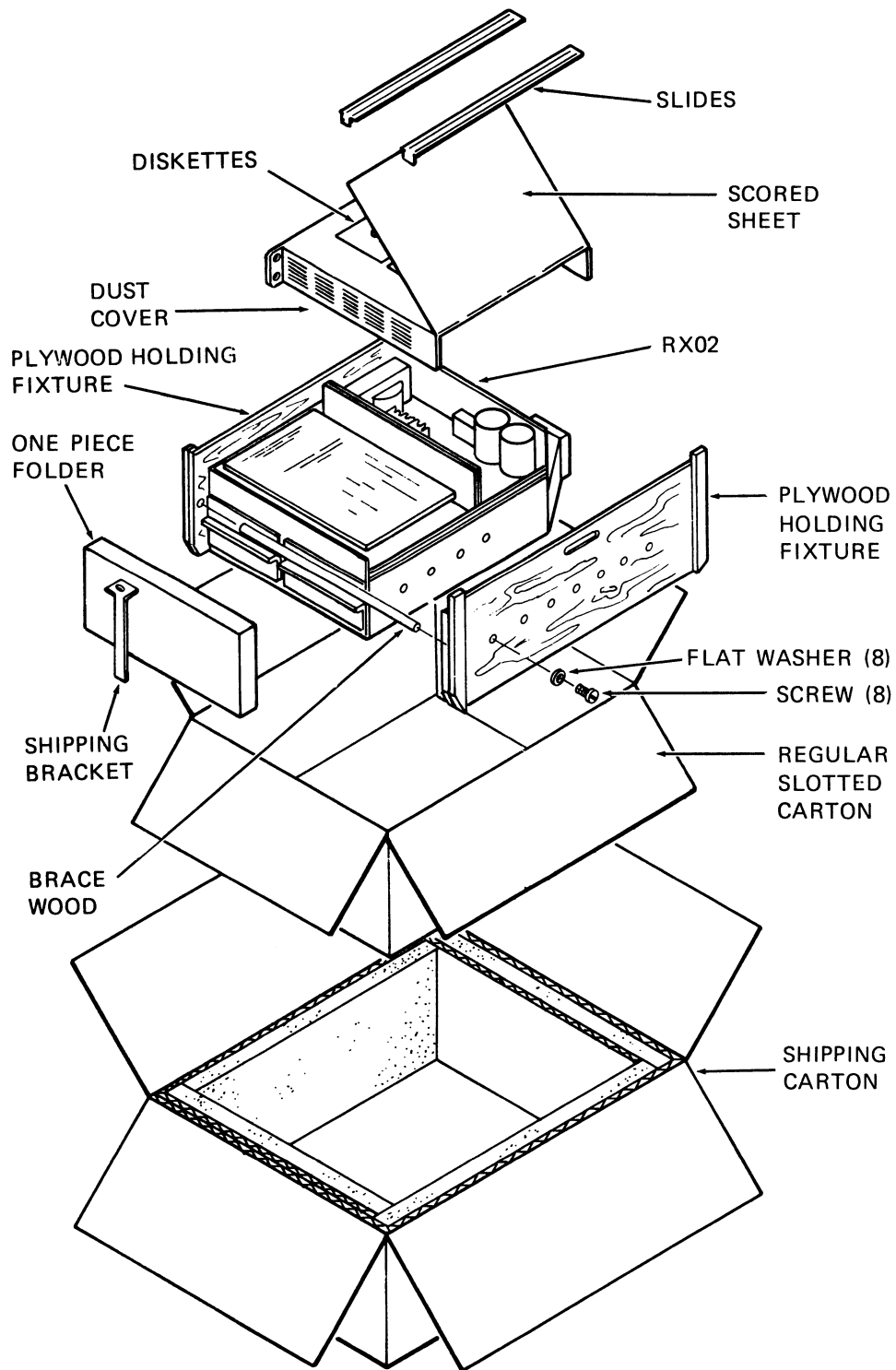
Figure 2-4 RX02 Unpacking
