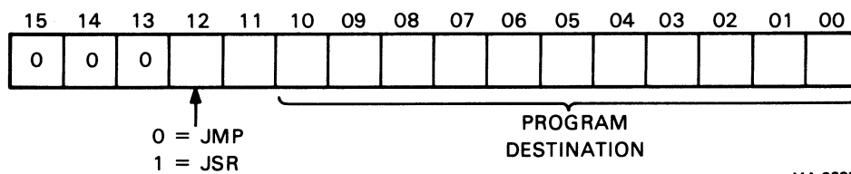
Figure 5-17 JMP/JSR Instruction Format
