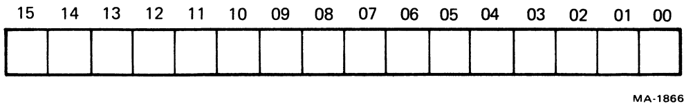
Figure 4-20 RXDB Format (RX11/RXV11)
