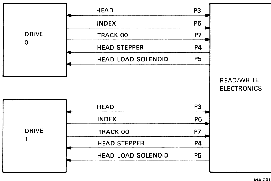
Figure 5-7 Read/Write Electronics to Drive Signals
