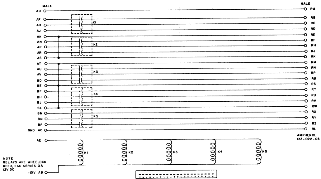
Relay RS-B-G851
