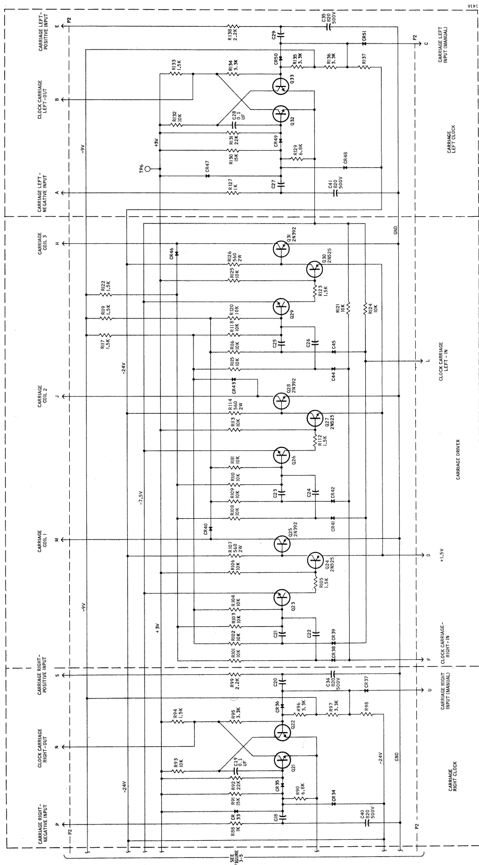
FIGURE 3-6 Schematic Diagram Carriage Step Motor Control Circuits
