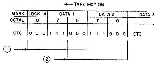
Figure 3-11 Mark-Track Decoding (MK DATA 070)
