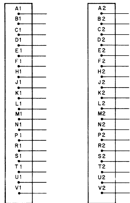
Figure 6-4 The G775 Connector Card Logic Symbol
