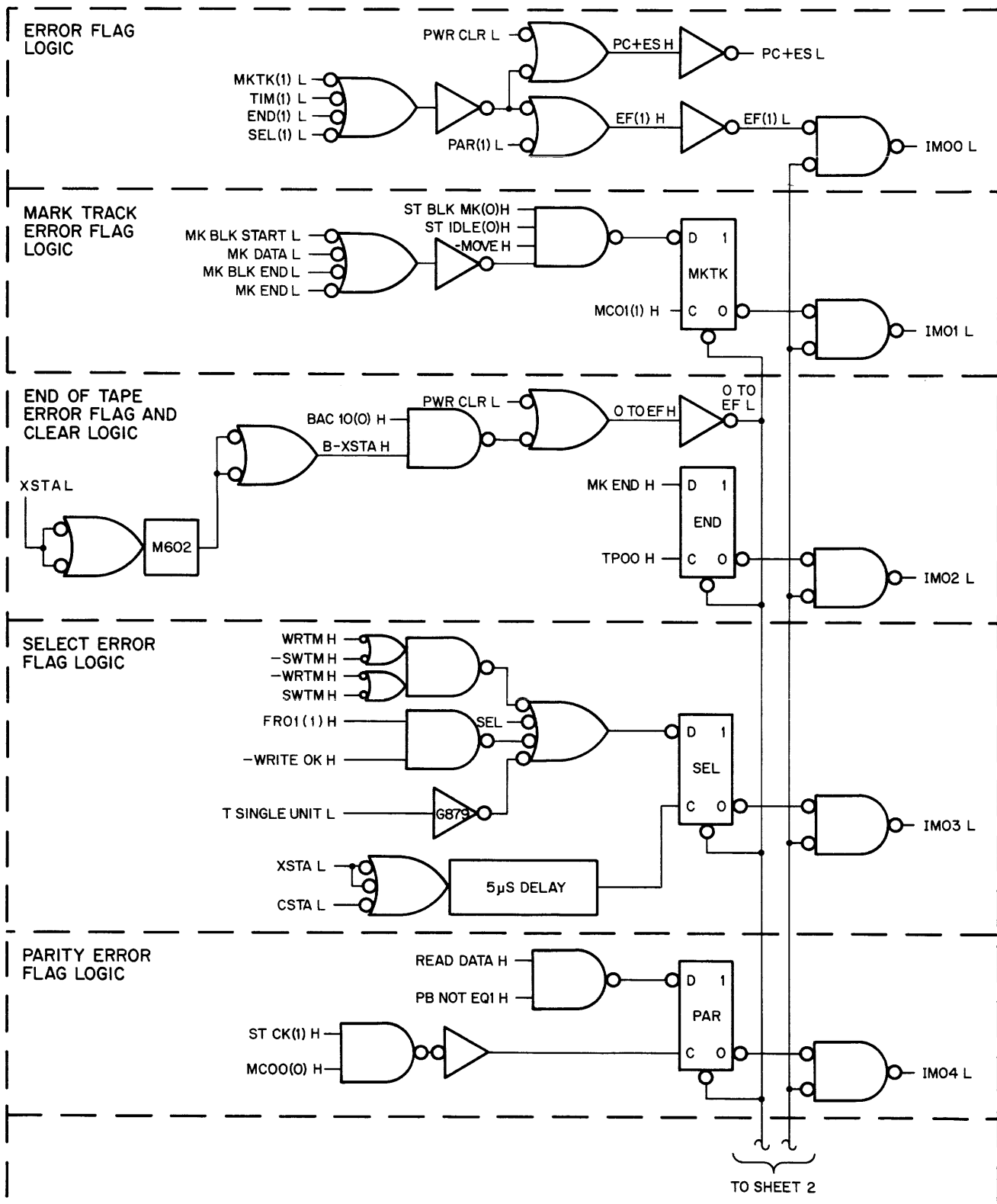
Figure 3-15 Status B Logic of the Error Flags (Sheet 1)
