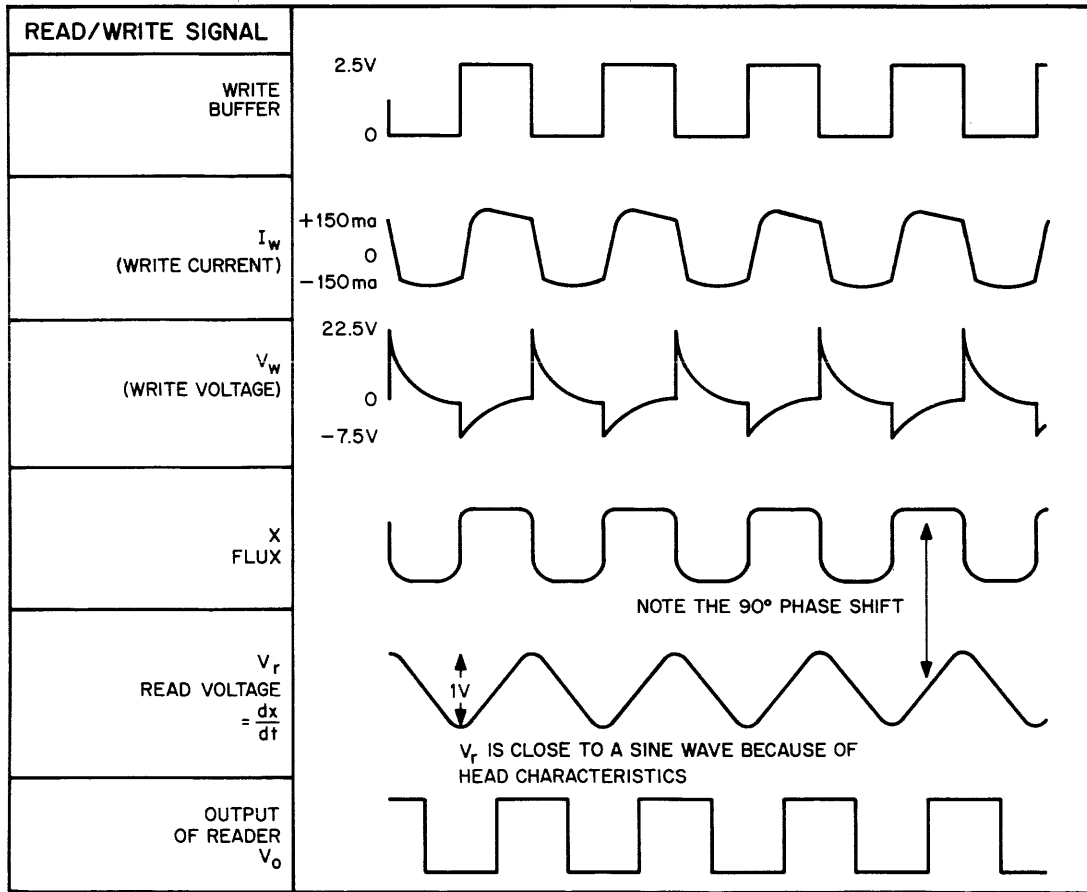
Figure 3-2 DECtape Read/Write Electronics and Waveforms
