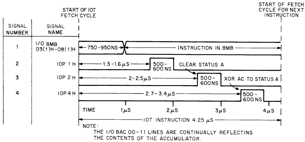
Figure 3-5A Command Register Timing with PDP-8/L
