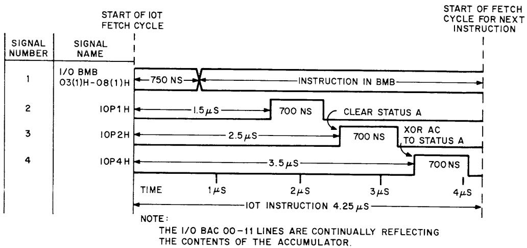
Figure 3-5B Command Register Timing with PDP-8
