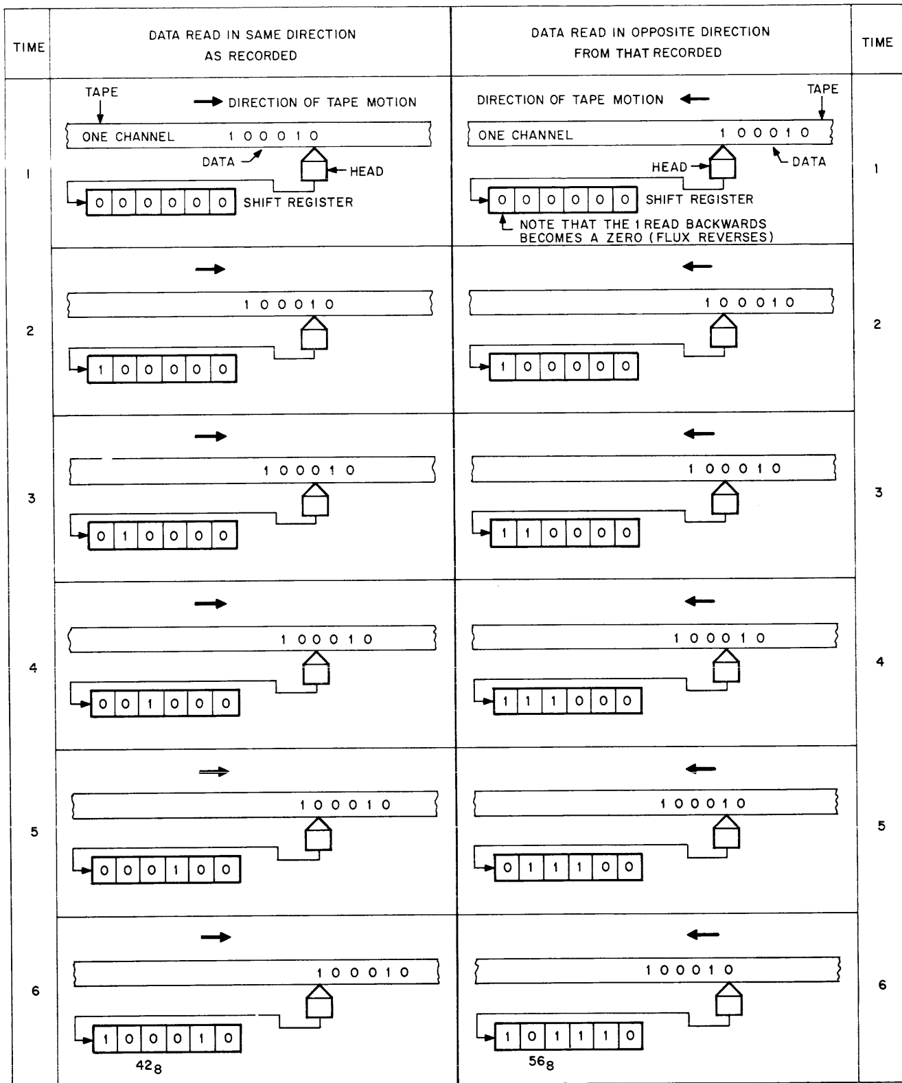
Figure 2-4 Bidirectional Reading and Writing
