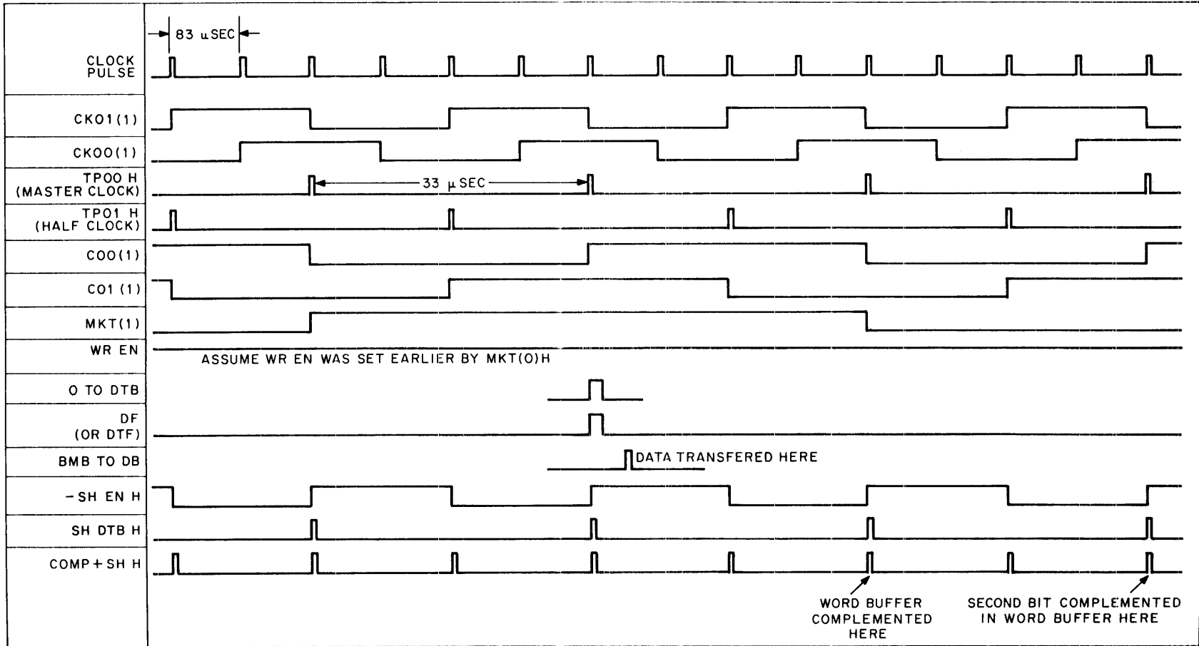
Figure 3-16 Write Timing and Mark Track Timing Diagram
