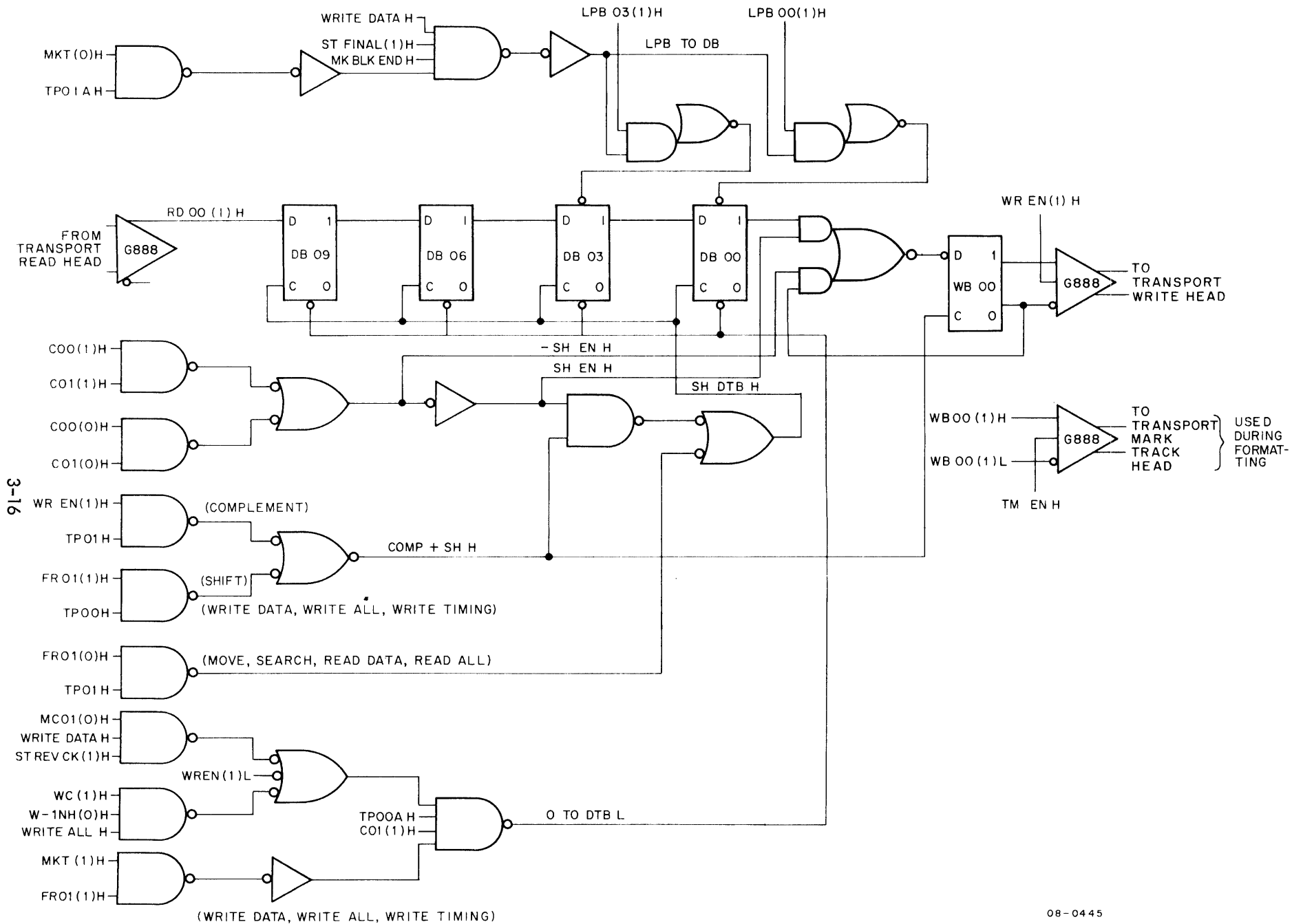
Figure 3-9 Data Buffer
