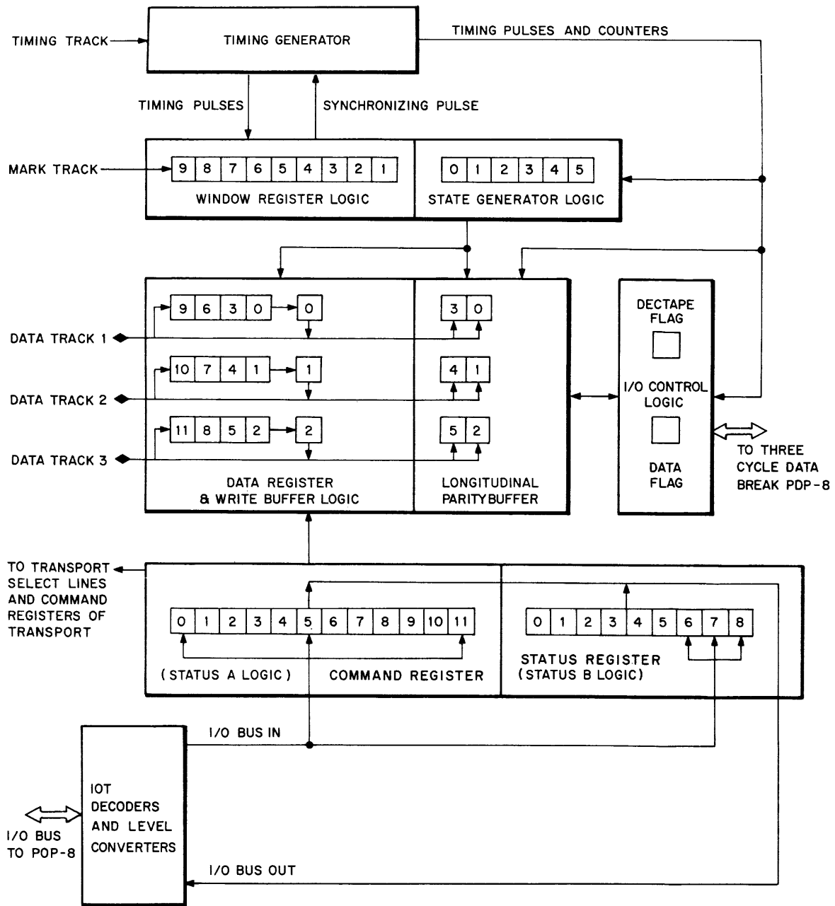
Figure 3-3 The TC08 DEctape Controller Block Diagram
