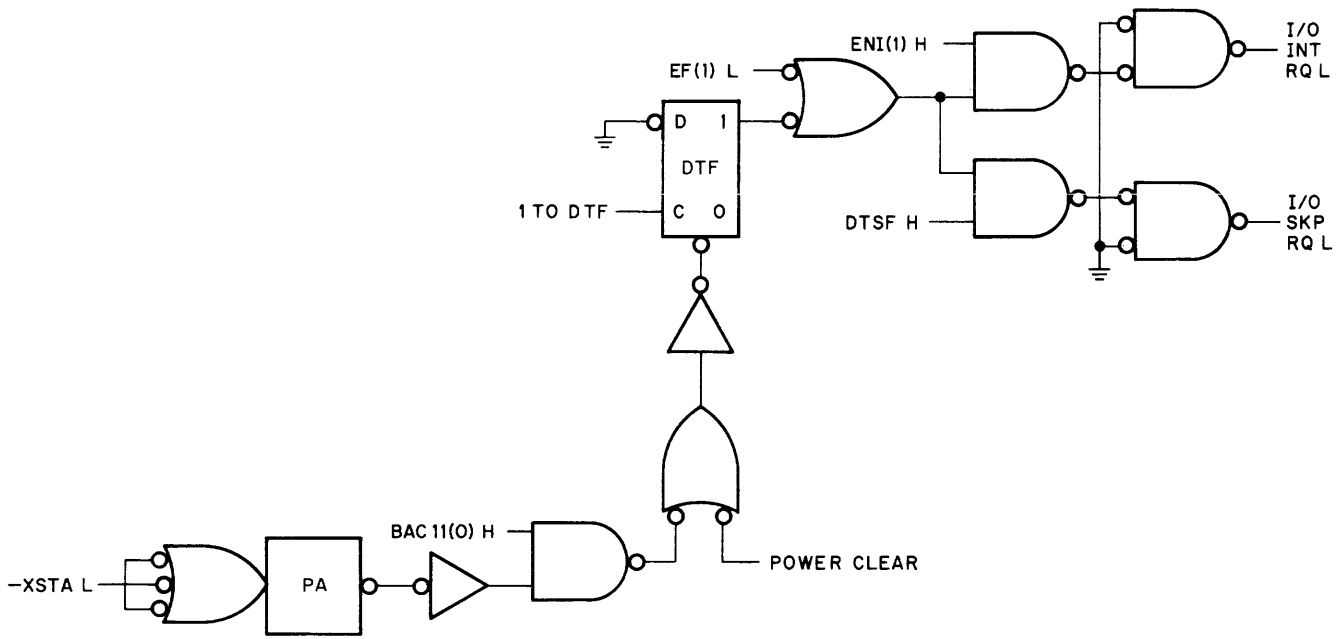
Figure 3-13 The DECTape Flag
