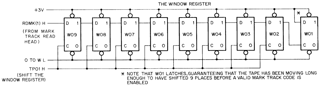
Figure 3-8 The Window Register and State Generator
