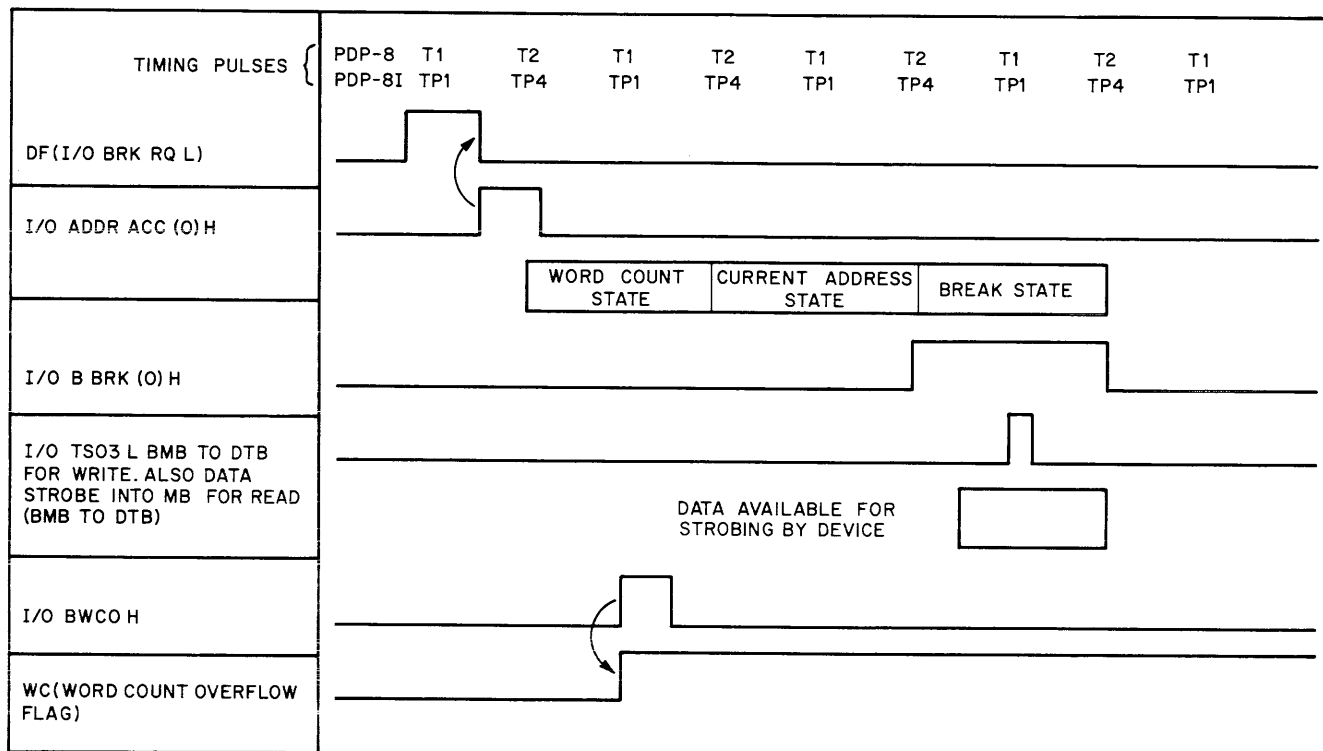
Figure 3-12 The I/O Control Timing
