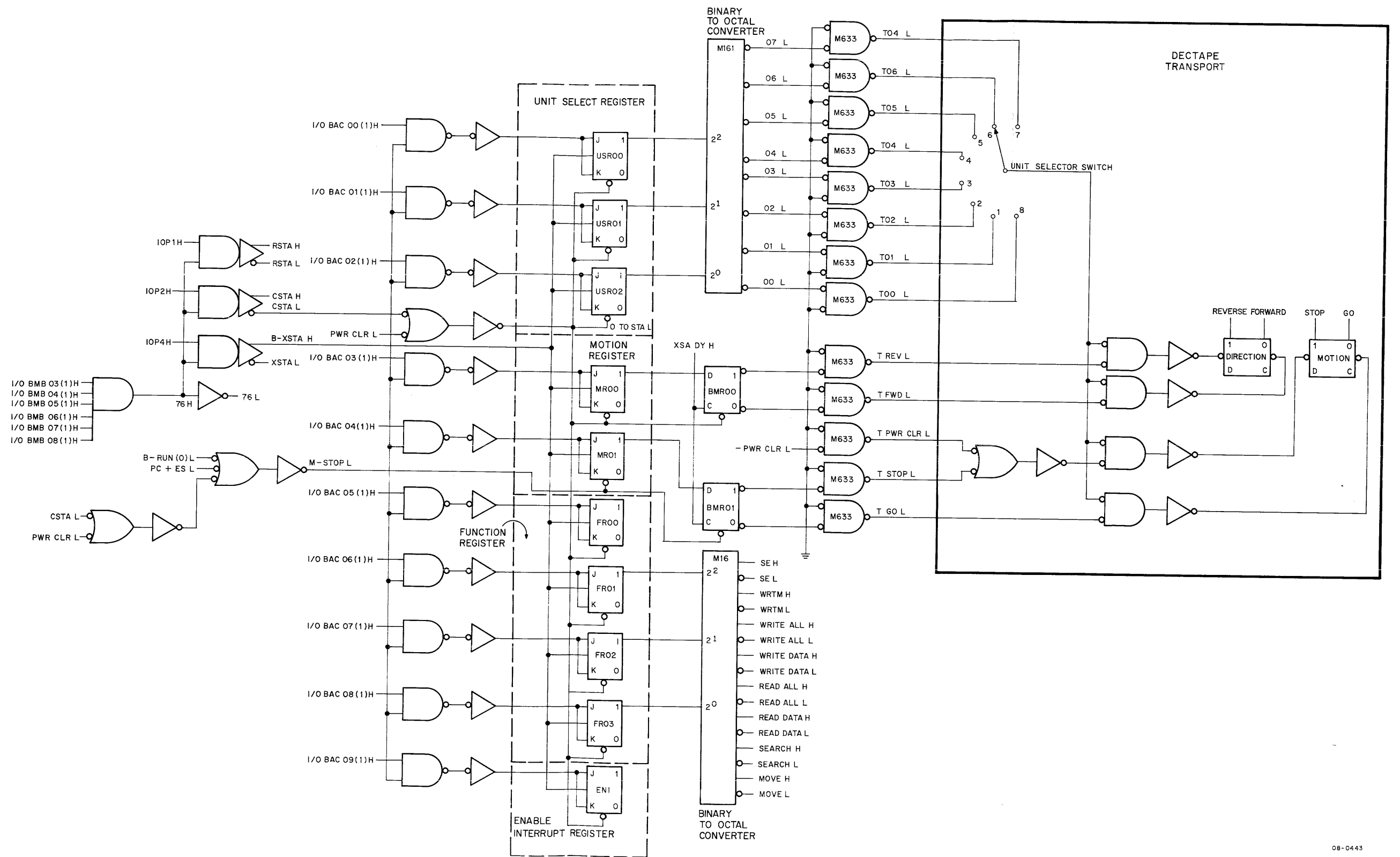
Figure 3-4 Command Register
