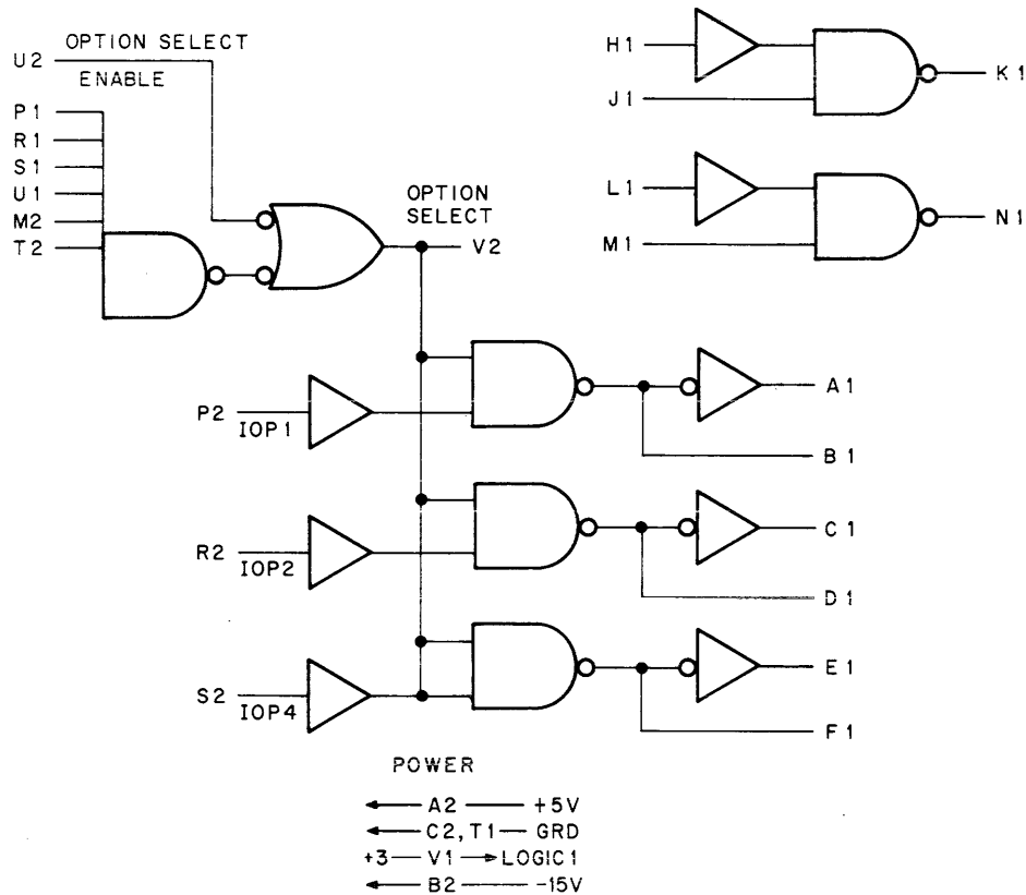
Figure 6-9 The M102 Device Selector
