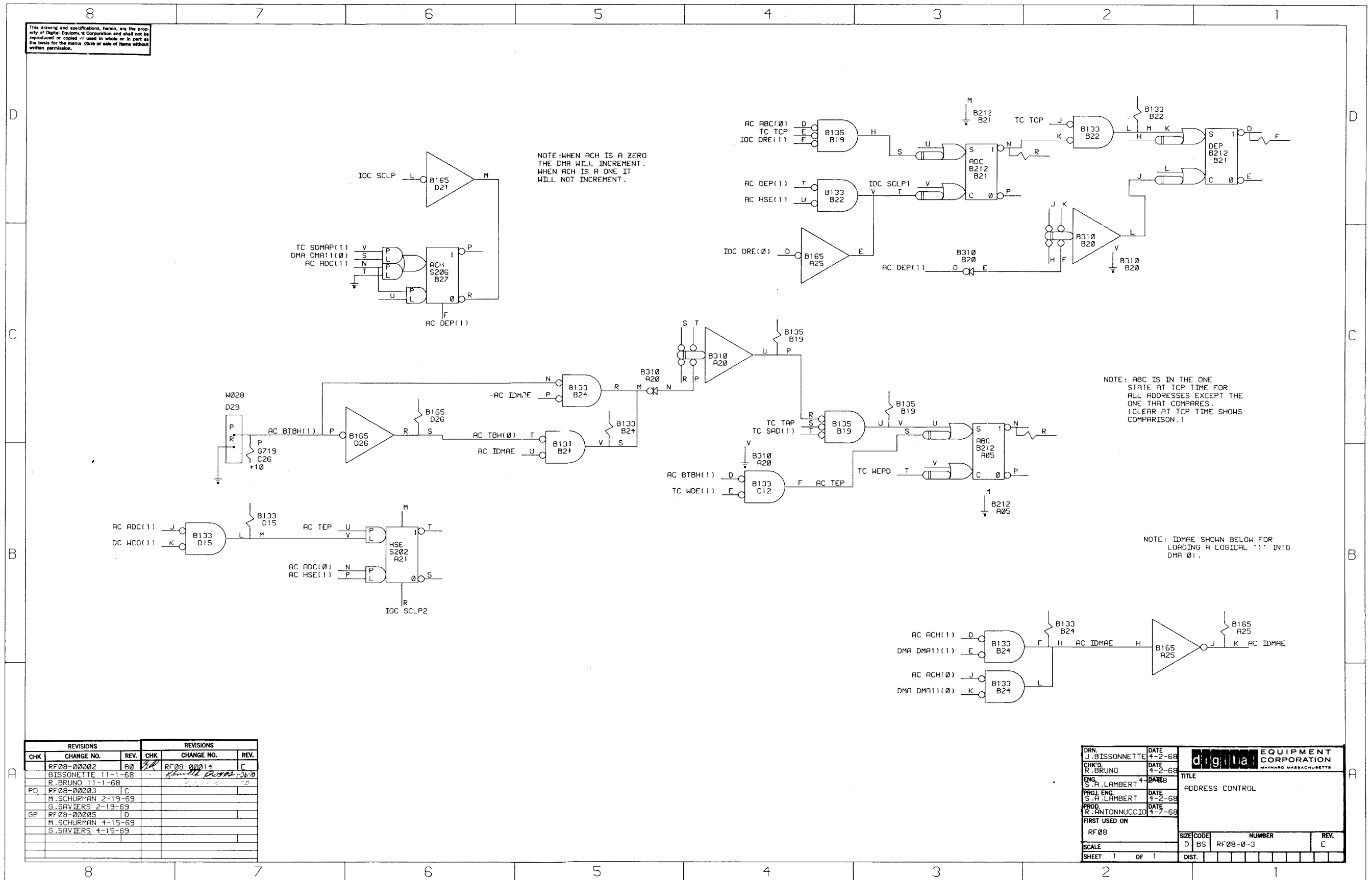
Figure 6-30 Address Control
