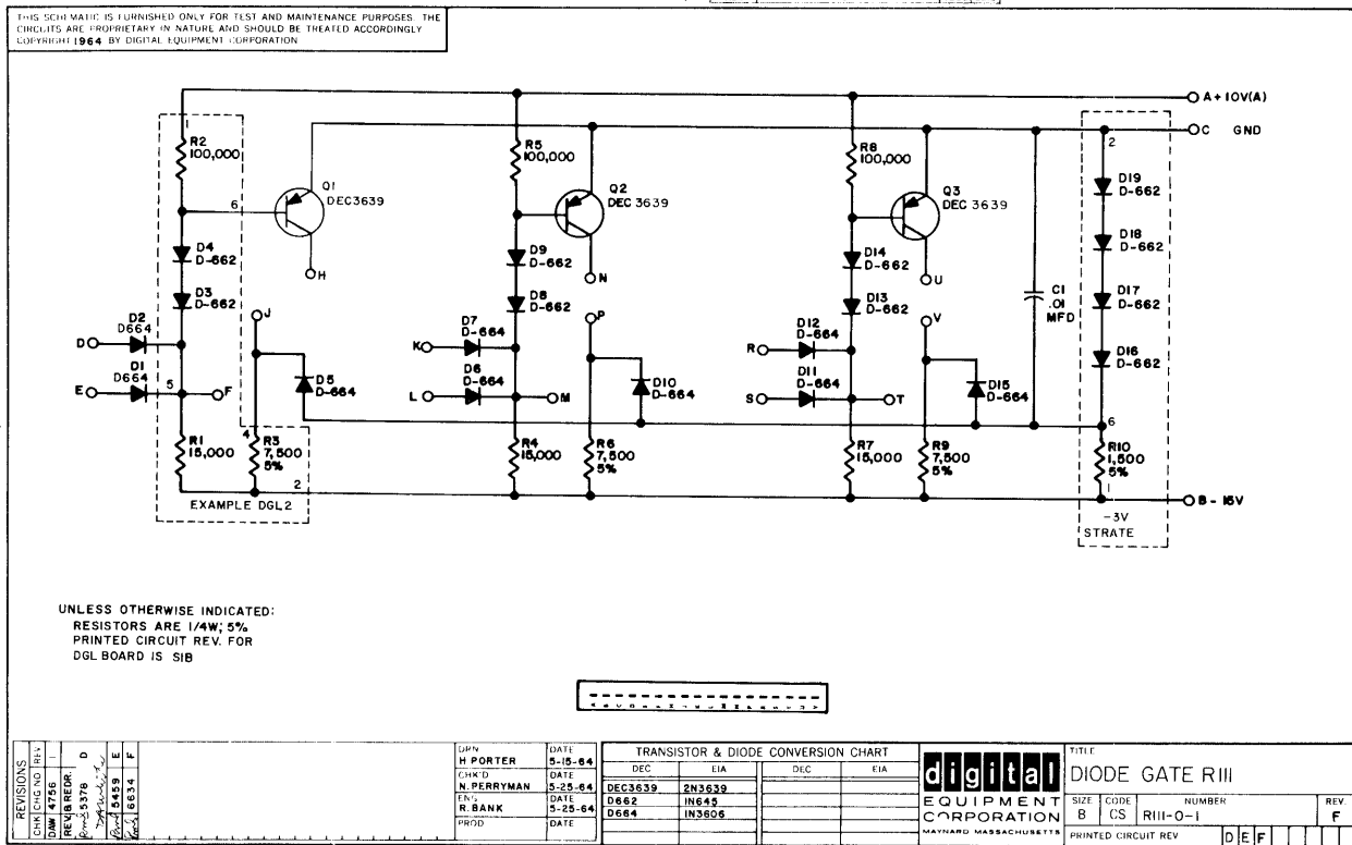
Figure 6-25 Diode Gate R111
