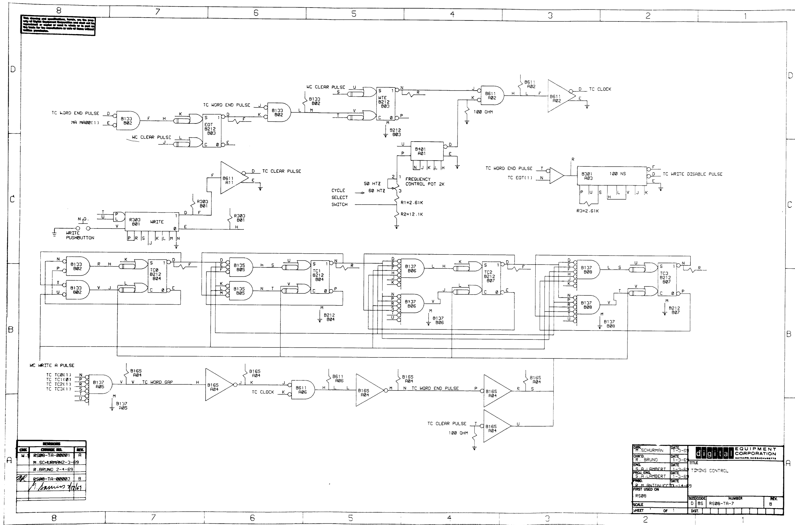
Figure 6-47 Timing Control
