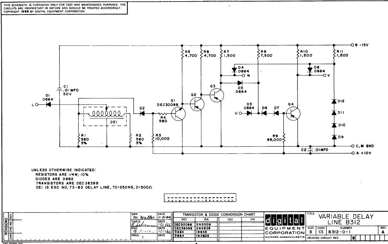
Figure 6-9 Variable Delay Line B312
