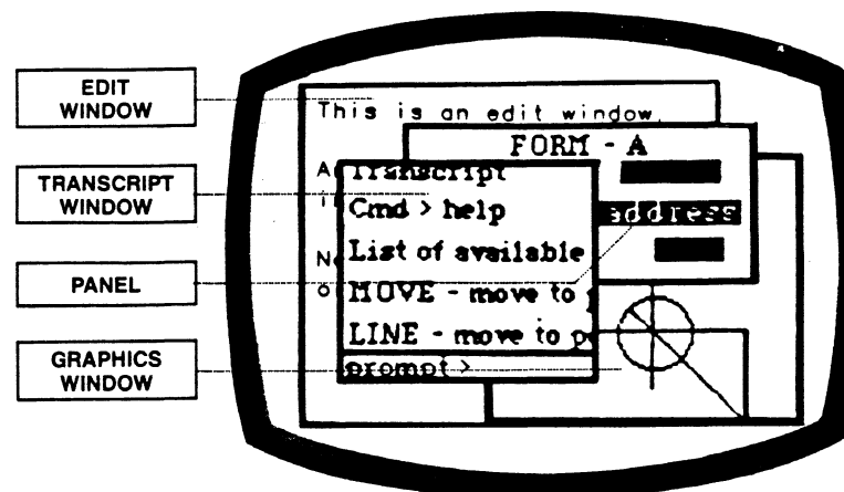
Figure 1. A multi-window display showing windows of several different types. Windowing systems are a widely used software tool where a portion of the user interface has been separated from application specific software.
