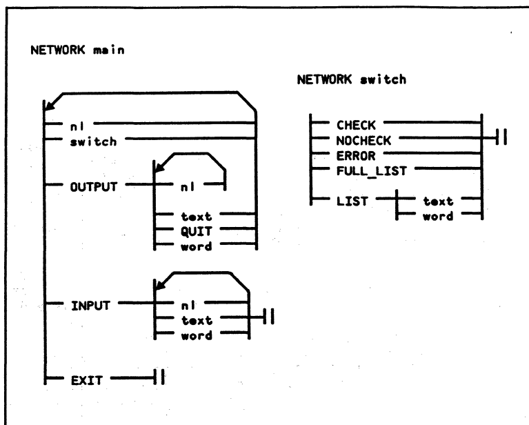
Figure 9. A command network diagram allows developers to define a command language using visual concepts that help prevent poor interface designs.
