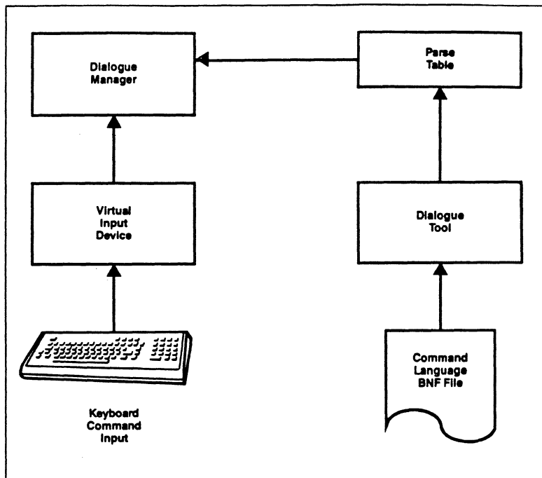
Figure 5. An example of a dialogue development tool. BNF grammar files are created which the development tool converts to a parse table. The parse table is used at run time by the Dialogue Manager to recognize valid command input.
