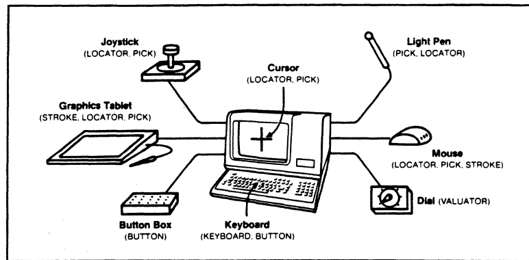
Figure 2. Many different physical devices can be supported by a given logical device. The logical device concept is part of all modern device independent graphics packages.
