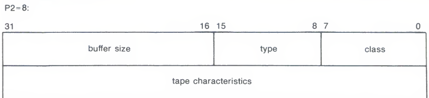
Figure 6-5 Set Characteristics Buffer
