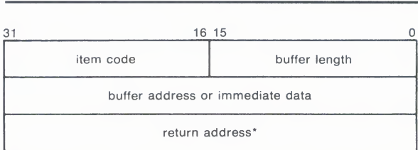
Figure 8-4 Itemlist Read Descriptor
