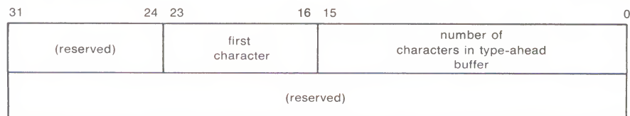
Figure 8–11 Sense Mode Characteristics Buffer (type-ahead)
