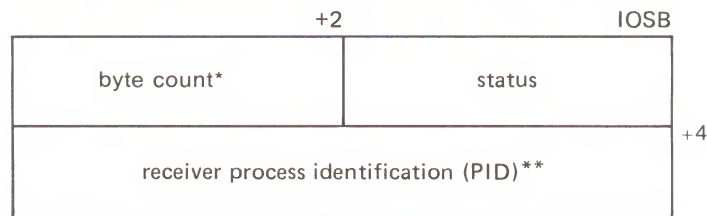
Figure 7-8 IOSB Contents - Write Function
