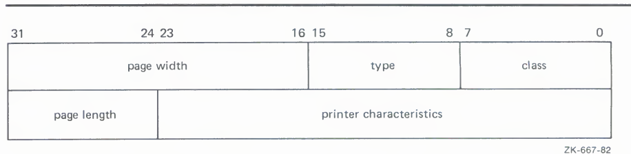
Figure 5-4 Set Characteristics Buffer
