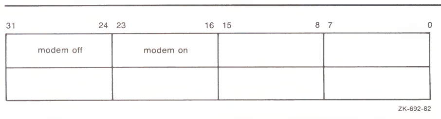
Figure 8-8 Set Mode P1 Block
