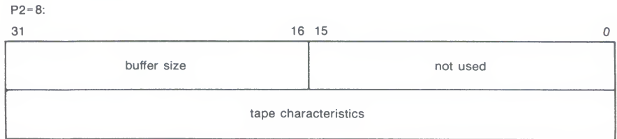
Figure 6-4 Set Mode Characteristics Buffer
