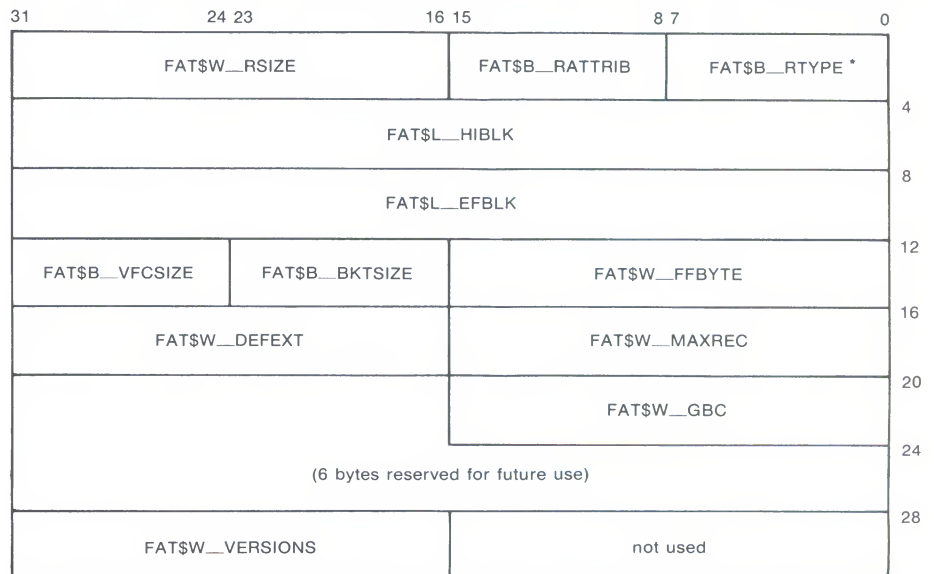
Figure 1-7 ACP-QIO Record Attributes Area
