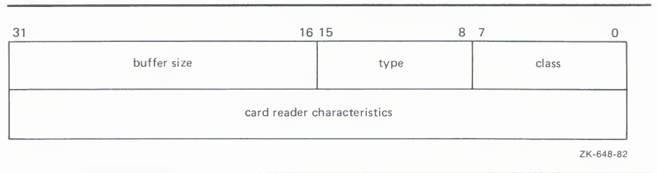
Figure 2-3 Set Characteristic Buffer
