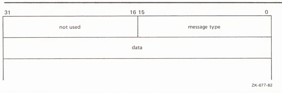
Figure 7-2 Typical Mailbox Message Format
