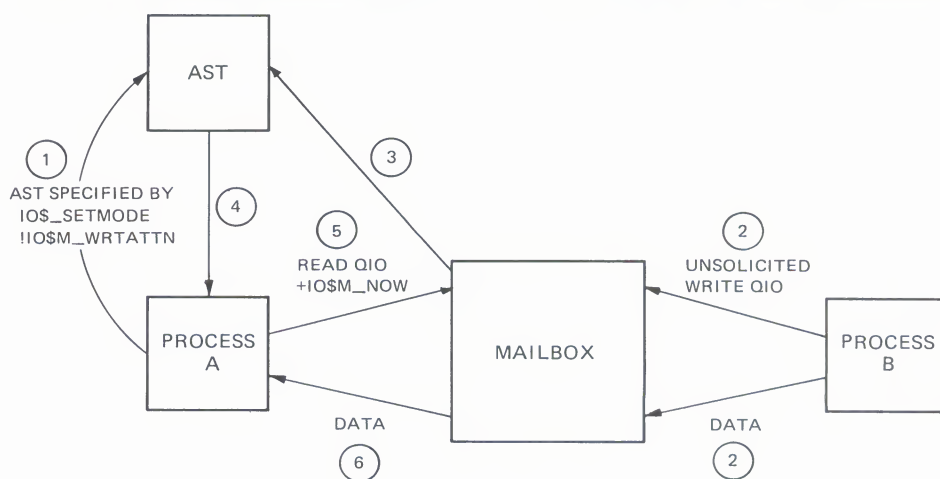
Figure 7-5 Write Attention AST (Read Unsolicited Data)
