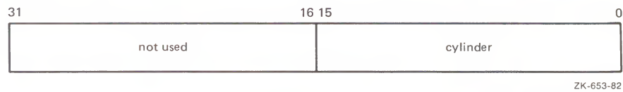
Figure 3-3 Physical Cylinder Number Format
