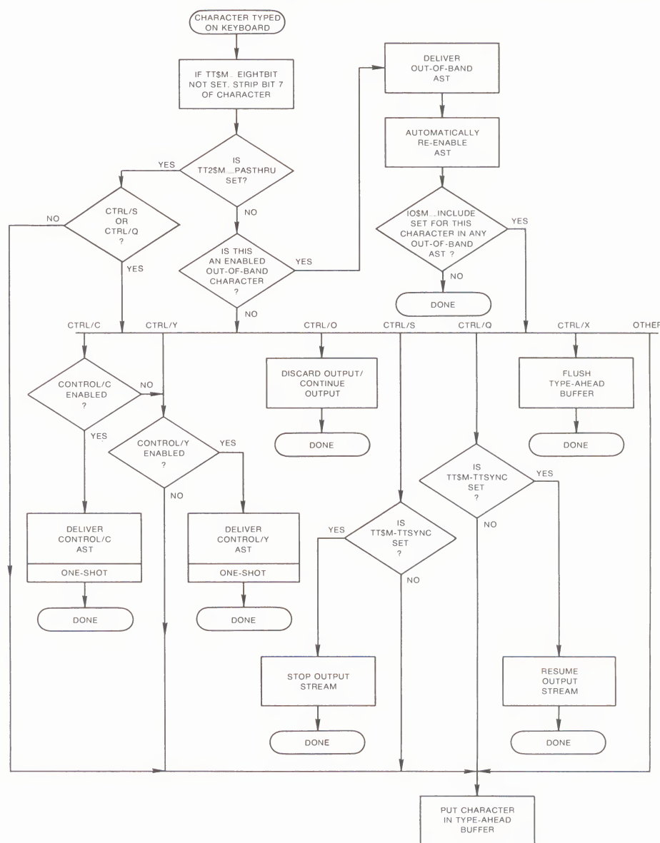
Figure 8-9 Relationship of Out-of-Band Function with Control Characters
