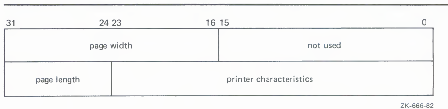
Figure 5-3 Set Mode Buffer
