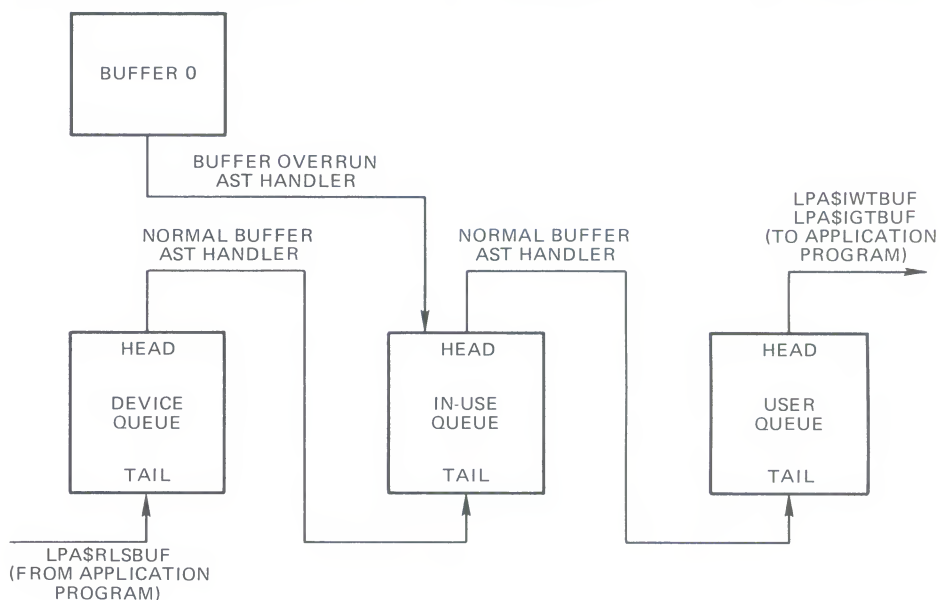
Figure 4-3 Buffer Queue Control
