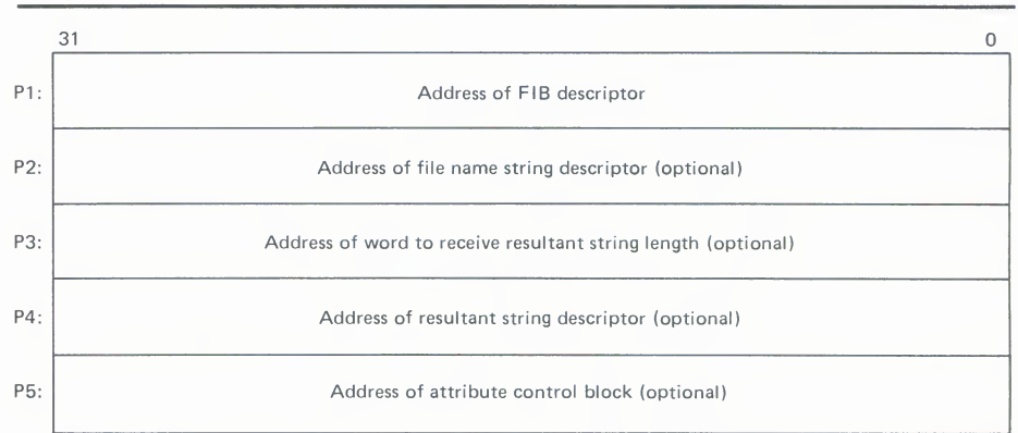
Figure 1-2 ACP Device/Function-Dependent Arguments
