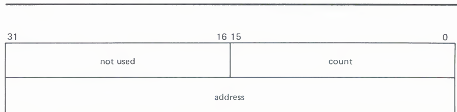
Figure 1-3 ACP Device/Function Argument Descriptor Format
