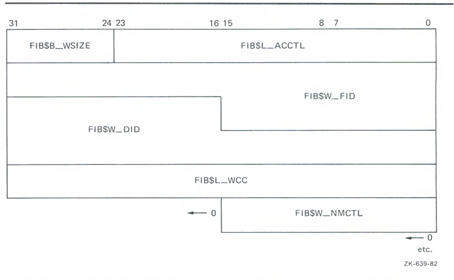
Figure 1-5 Typical Short File Information Block
