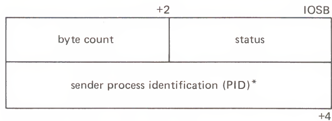
Figure 7-7 IOSB Contents - Read Function
