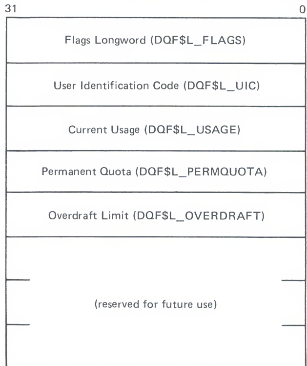
Figure 1-9 Quota File Transfer Block
