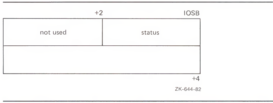
Figure 1-10 IOSB Contents - ACP-QIO Functions
