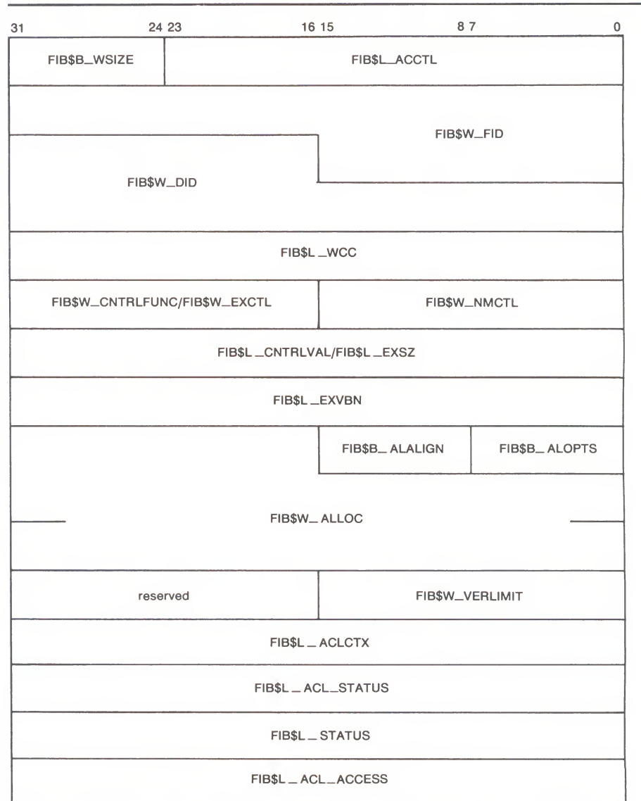
Figure 1-4 File Information Block Format
