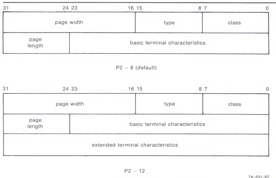
Figure 8–7 Set Mode and Set Characteristics Buffers
