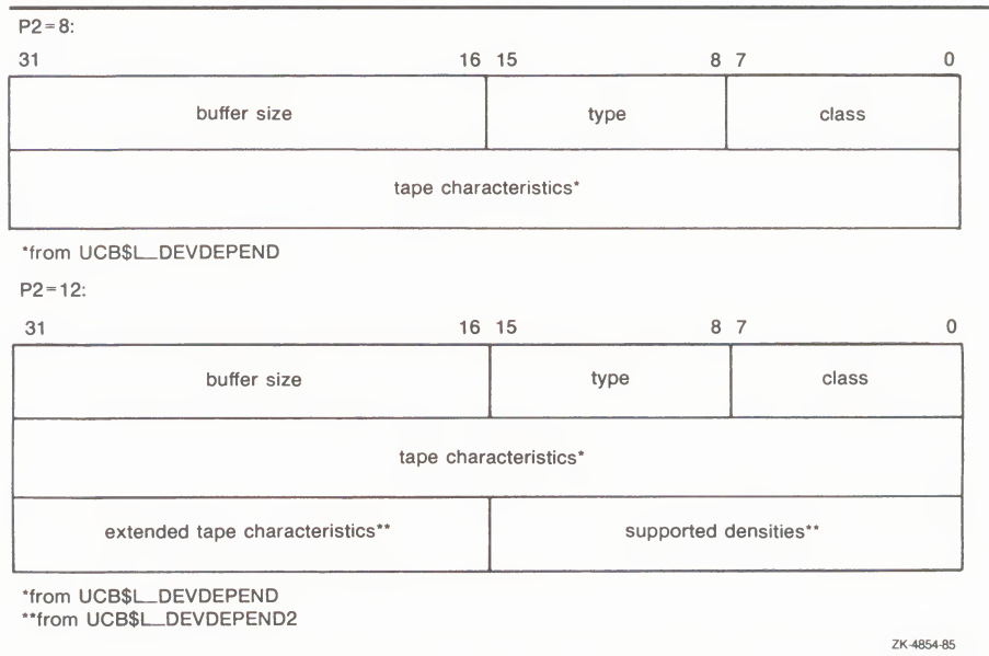
Figure 6-3 Sense Mode P1 Buffer
