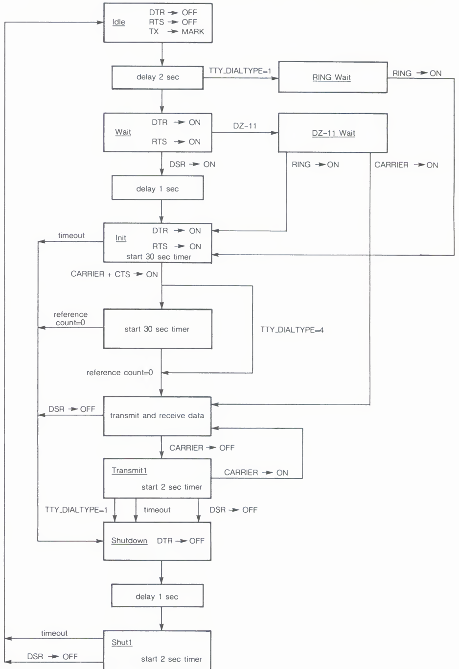
Figure 8-1 Modem Control - Two-Way Simultaneous Operation
