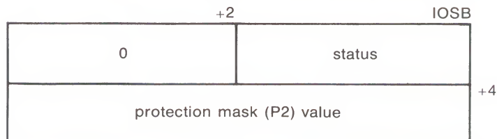
Figure 7-9 IOSB Contents - Set Protection Function
