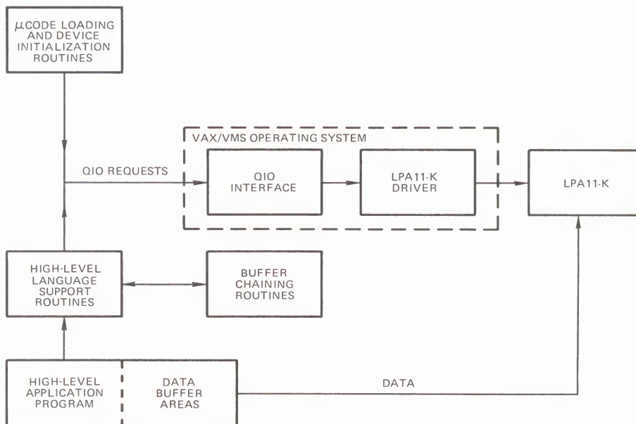
Figure 4-1 Relationship of Supporting Software to LPA11-K
