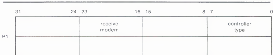
Figure 8–12 Sense Mode P1 Block
