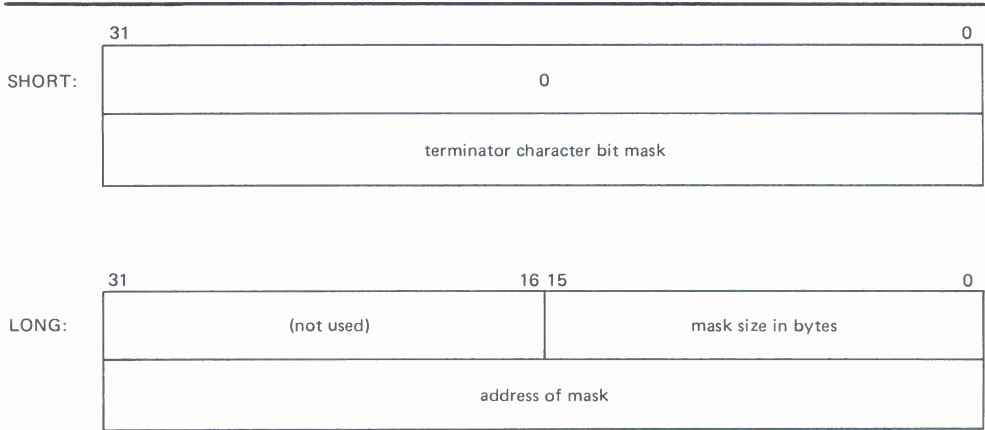
Figure 8-3 Short and Long Forms of Terminator Mask Quadwords
