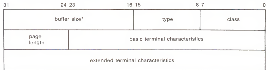
Figure 8–10 Sense Mode Characteristics Buffer
