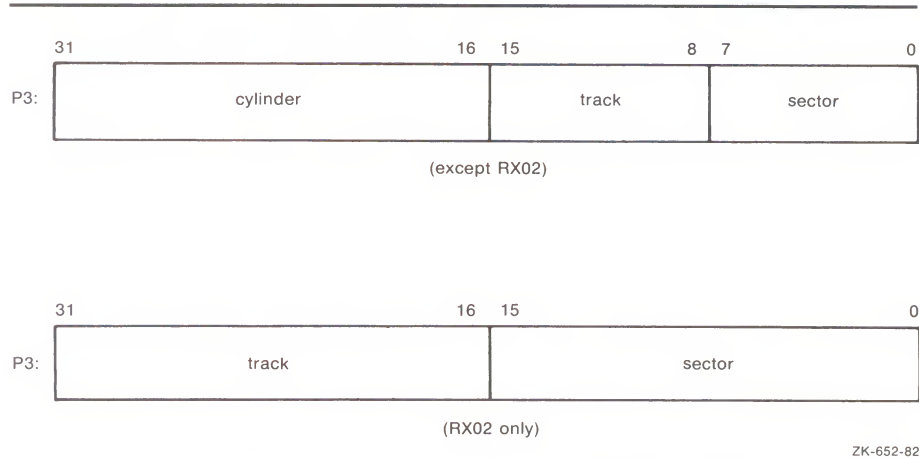
Figure 3-2 Starting Physical Address
