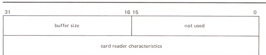
Figure 2-2 Set Mode Characteristics Buffer
