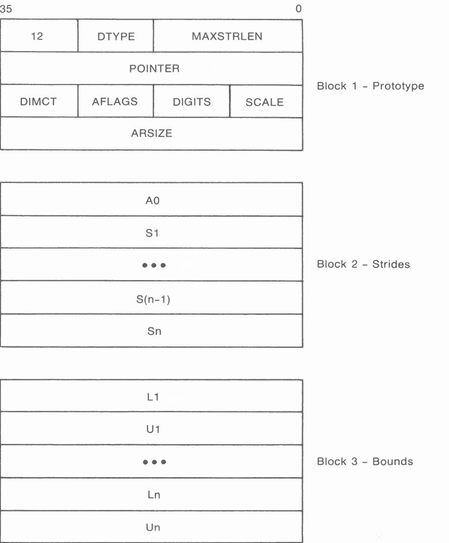
Figure 2-12 Varying String Array Descriptor Format
