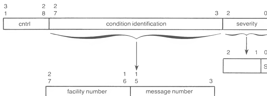
Figure 2-2 Format of the Condition Value
