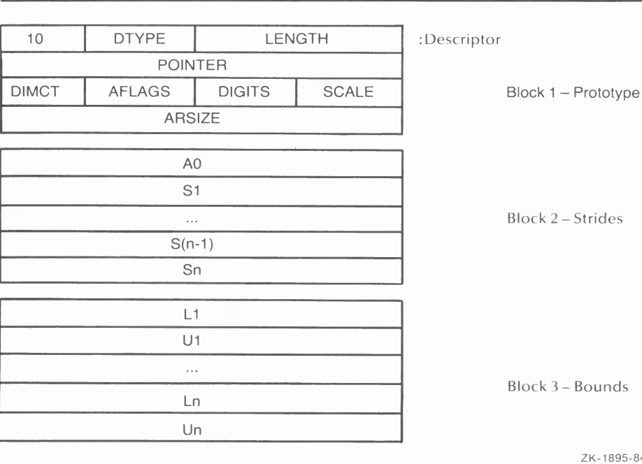
Figure 2-10 Noncontiguous Array Descriptor Format
