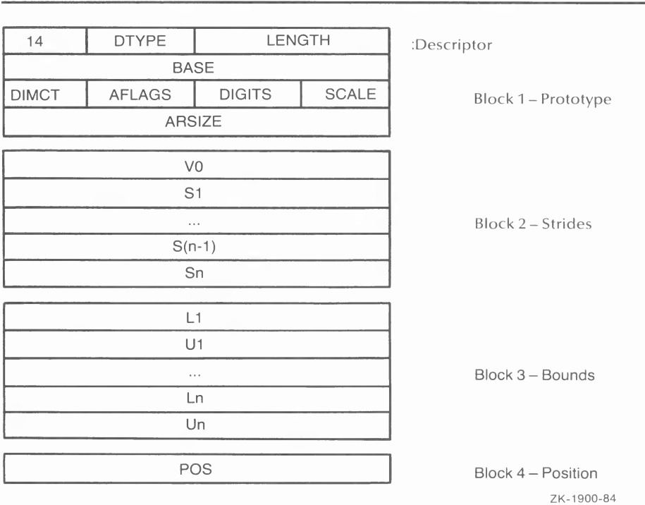
Figure 2-14 Unaligned Bit Array Descriptor Format
