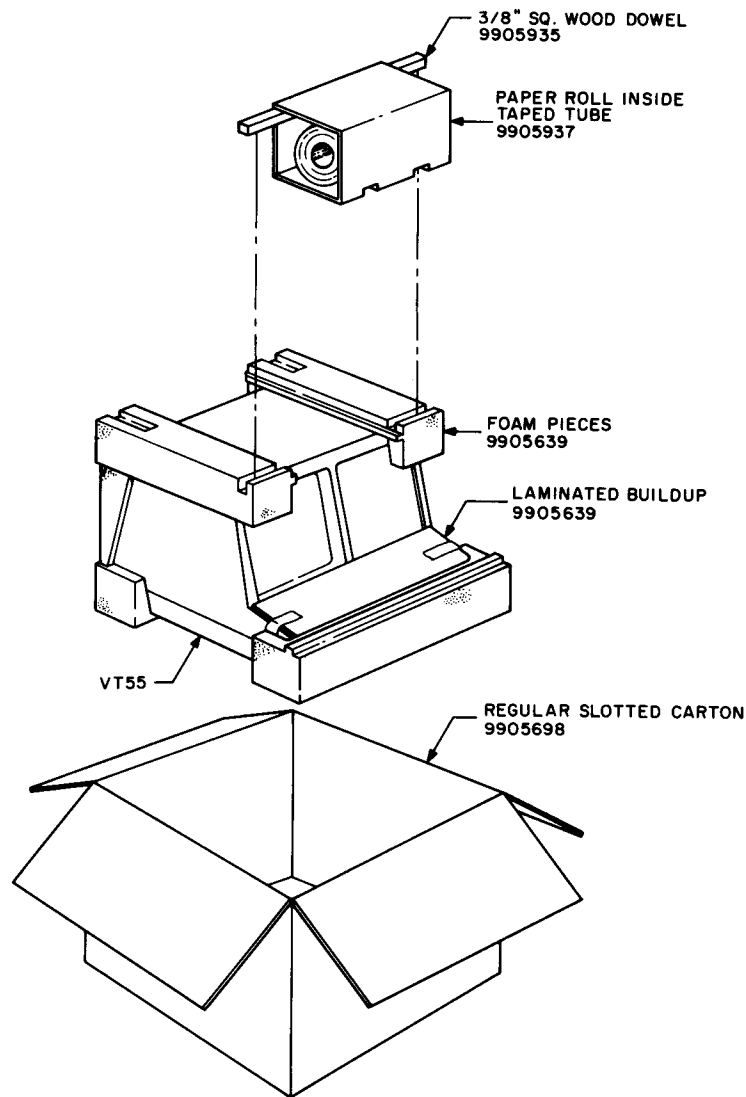
Figure 6-7 VT55 Packing
