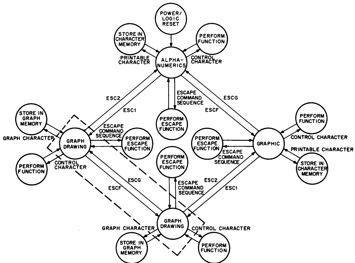
Figure 5-2 State Diagram showing Change Between Alphanumeric, Graphic, Graph Drawing, and Escape Modes
