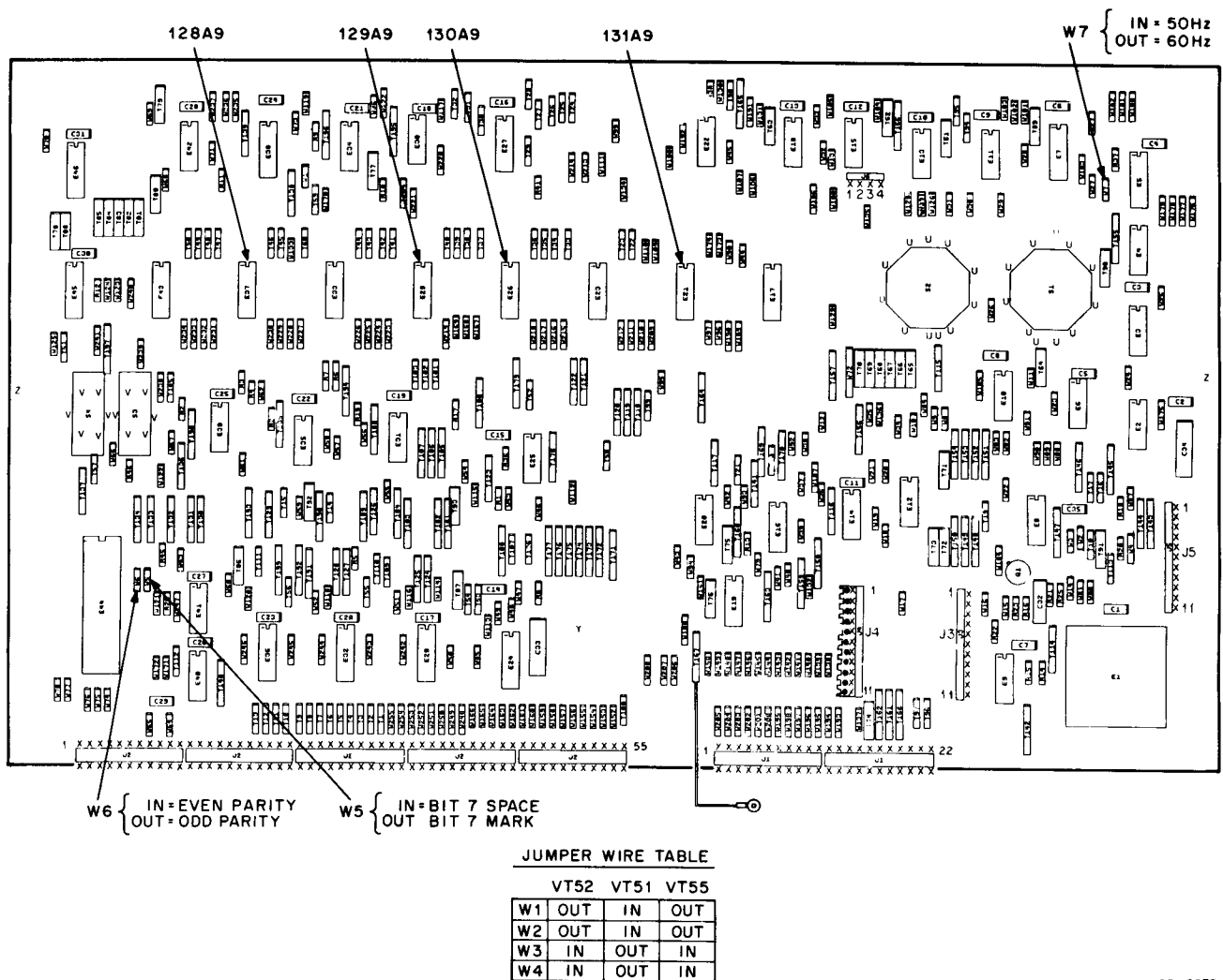
Figure 6-2 ROM, UART, and Timing Module
