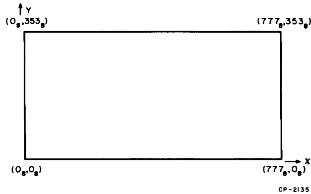
Figure 5-4 Graph Drawing Data Field Calibration
