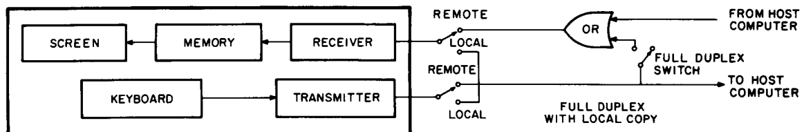
Figure 4-1 Interface Modes
