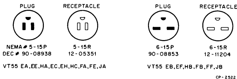
Figure 2-2 VT55 Power Connectors
