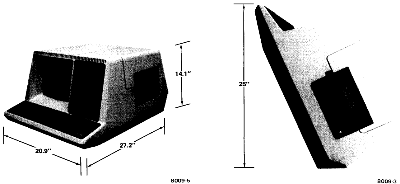
Figure 2-1 VT55 Installation Dimensions
