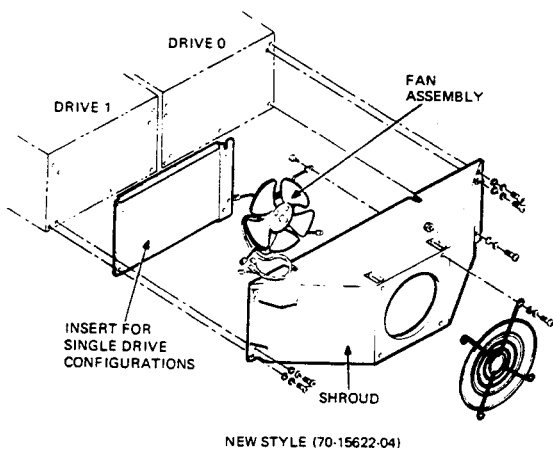
Figure 2-6 Plenum/Fan Assembly
