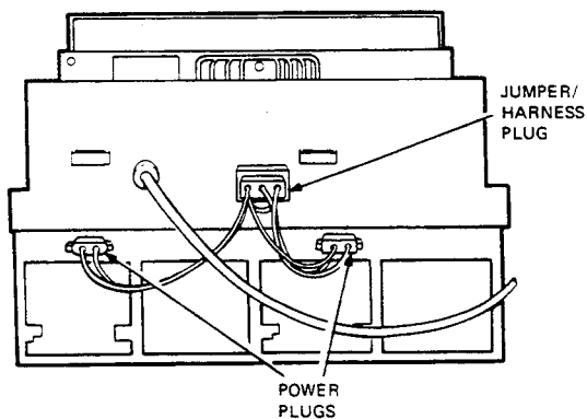
DRIVE POWER PLUGS (REAR VIEW; FAN REMOVED)
