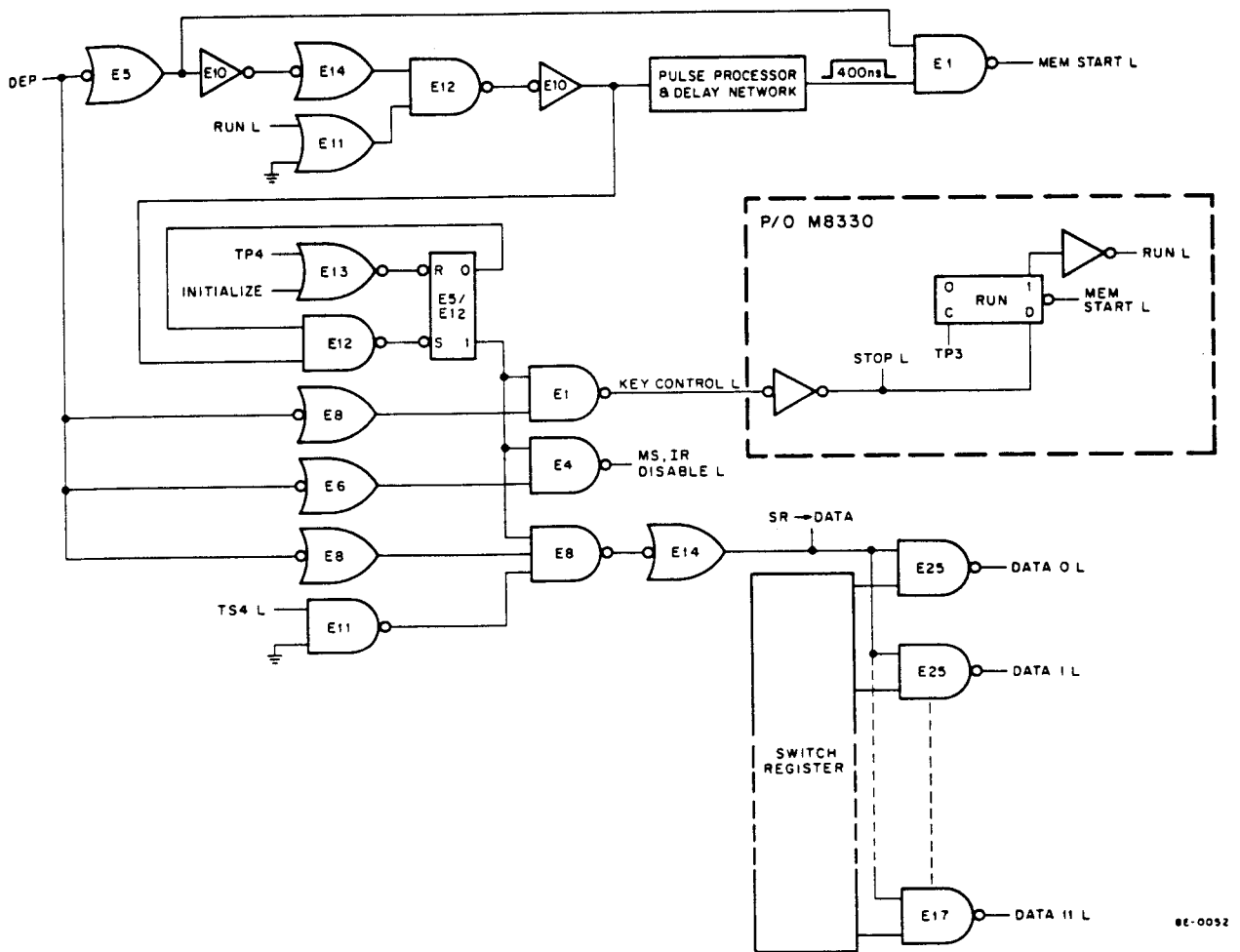
Figure 3-71 DEP Key Logic
