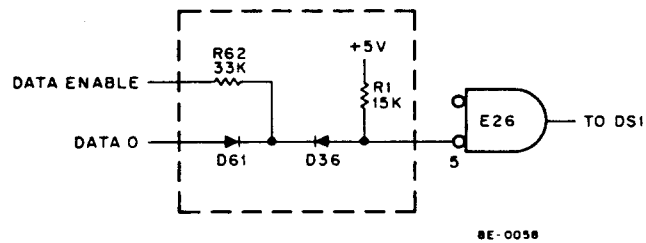
Figure 3-78 Enable Circuit
