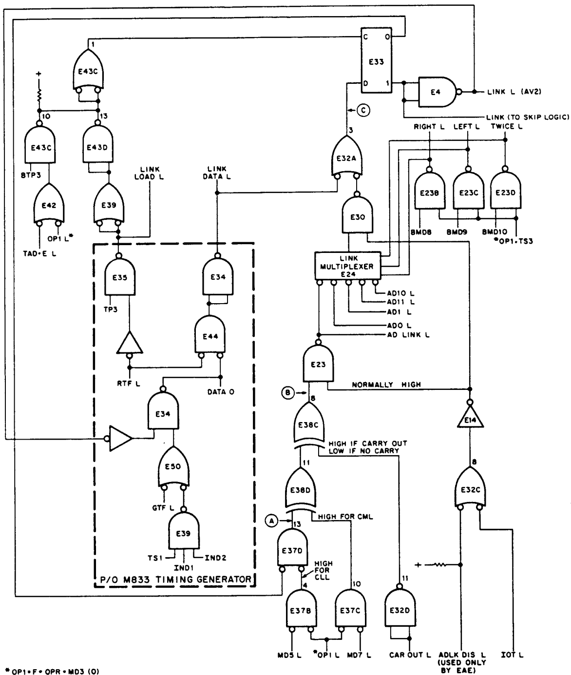
Figure 3-100 Link Logic
