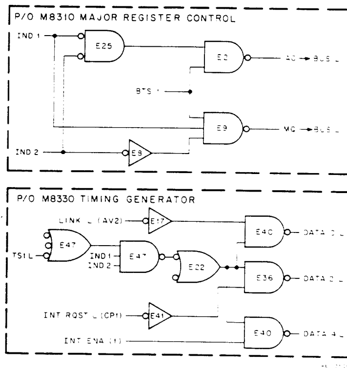
Figure 3-86 Data Bus Display Control Signals
