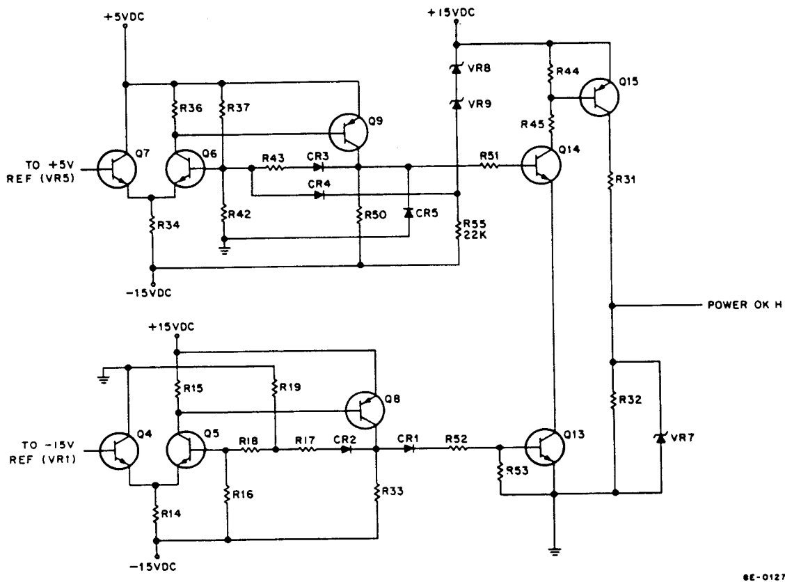
Figure 3-127 dc Voltage Monitor
