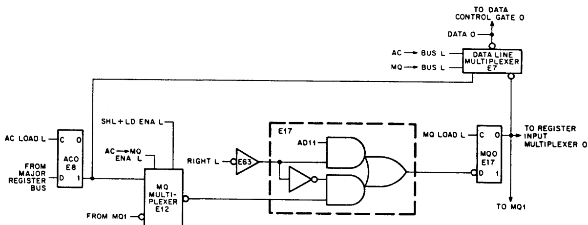
Figure 3-101 MQ Logic
