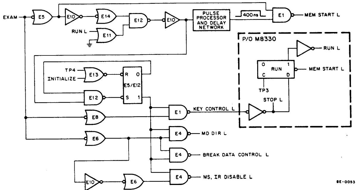
Figure 3-72 EXAM Key Logic
