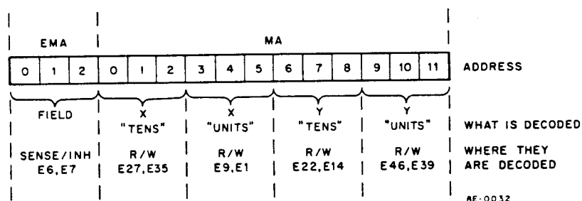
Figure 3-46 Decoding Relationships
