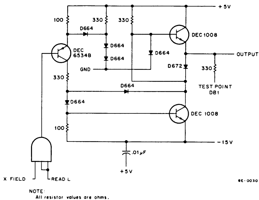
Figure 3-44 Bias Driver
