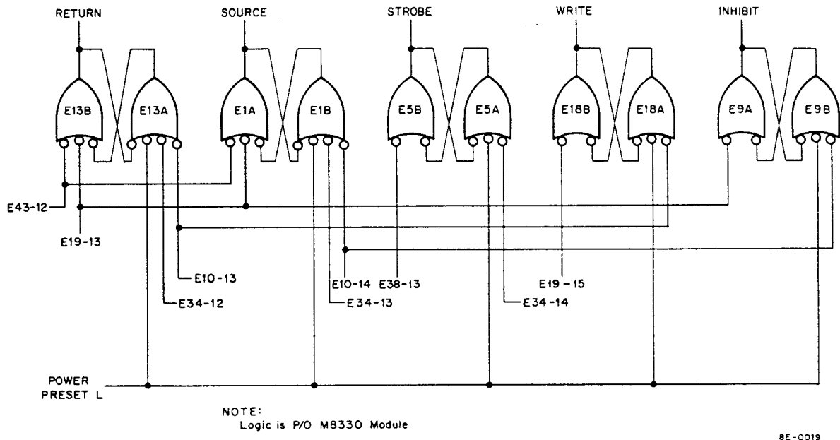
Figure 3-28 Memory Timing Signal Logic
