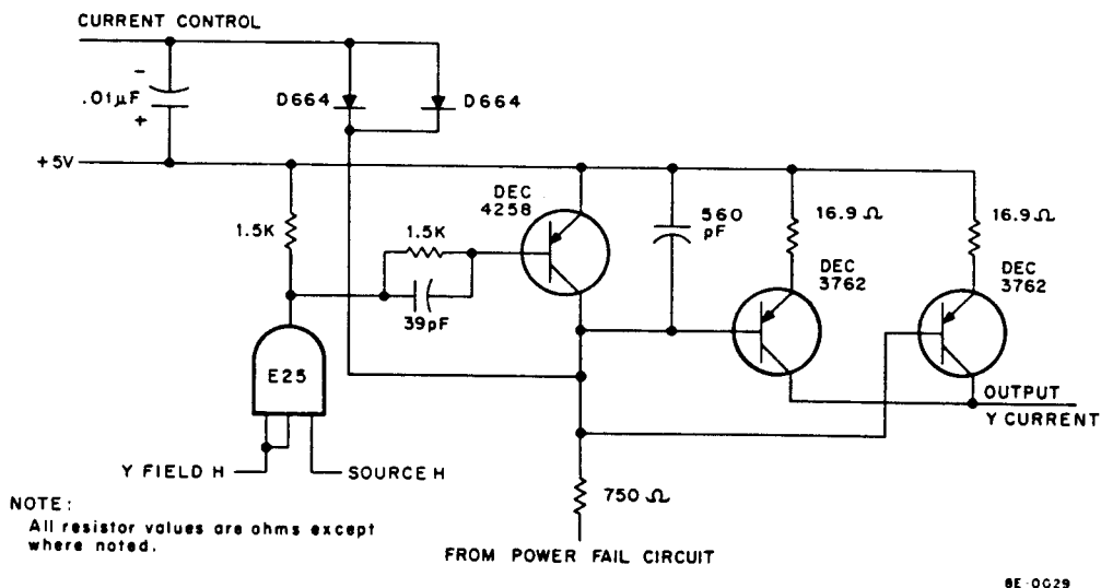
Figure 3-43 Y-Current Source
